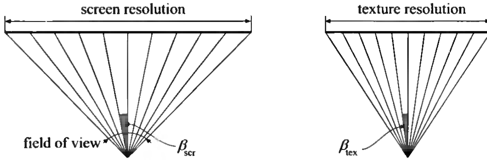
Figure 10.14. The angle of a screen pixel is computed as \beta_{scr} = fov/screenres , and the angle for the texture is computed similarly. Note that these are both approximations as neither of the angles are constant for all pixels/texels.
