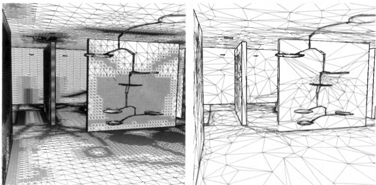
Figure 12.25. Simplification of radiosity solution. Left is the original mesh (150,983 faces); right is simplified mesh (10,000 faces). ( Images courtesy of Hugues Hoppe, Microsoft Research. )
