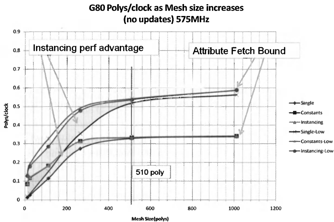
Figure 15.2. Batching performance benchmarks for an Intel Core 2 Duo 2.66 GHz CPU using an NVIDIA G80 GPU, running DirectX 10. Batches of varying size were run and timed under different conditions. The “Low” conditions are for triangles with just the position and a constant-color pixel shader; the other set of tests is for reasonable meshes and shading. “Single” is rendering a single batch many times. “Instancing” reuses the mesh data and puts the per-instance data in a separate stream. “Constants” is a DirectX 10 method where instance data is put in constant memory. As can be seen, small batches hurt all methods, but instancing gives proportionally much faster performance. At a few hundred polygons, performance levels out, as the bottleneck becomes how fast vertices are retrieved from the vertex buffer and caches. (Graph courtesy of NVIDIA Corporation.)
