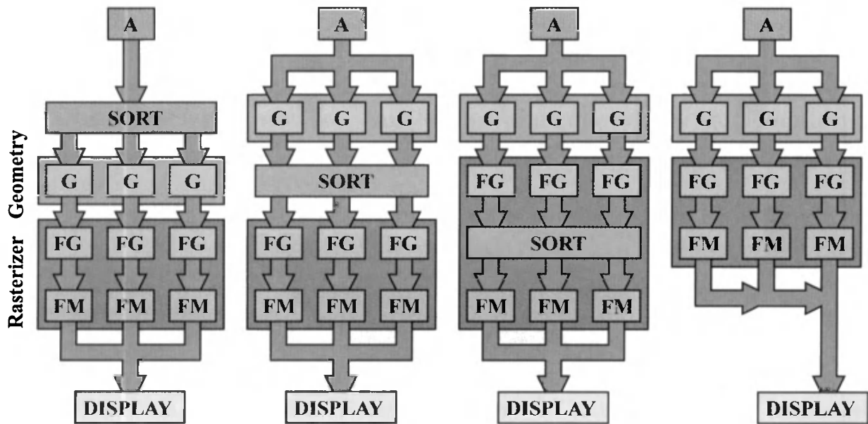
Figure 18.9. Taxonomy of parallel graphics architectures. A is the application, G is the geometry stage, then follows the rasterizer comprised of FG, which is fragment generation , and FM, which is fragment merging . The architectures are (left to right): sort-first, sort-middle, sort-last fragment, and sort-last image. (Illustration after Eldridge et al. [302].)
