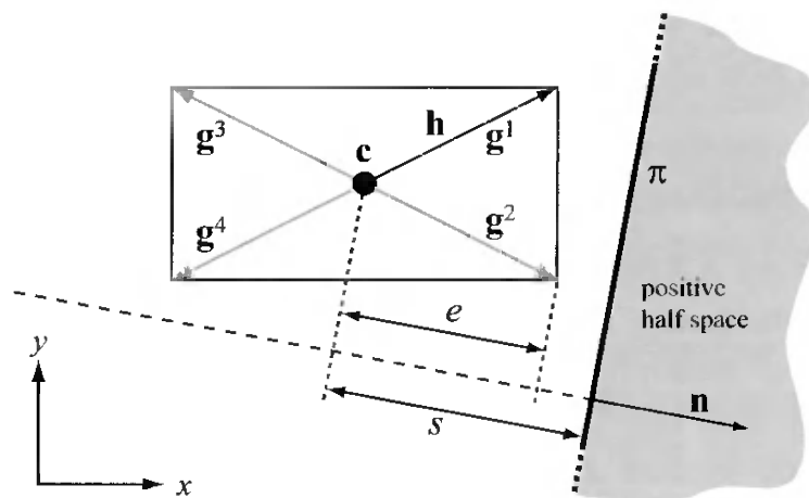
Figure 16.14. An axis-aligned box with center, \mathbf{c} , and positive half diagonal, \mathbf{h} , is tested against a plane, \pi . The idea is to compute the signed distance, s , from the center of the box to the plane, and compare that to the “extent,” e , of the box. The vectors \mathbf{g}^i are the different possible diagonals of the two-dimensional box, where \mathbf{h} is equal to \mathbf{g}^1 in this example. Note also that the signed distance s is negative, and its magnitude is larger than e , indicating that the box is inside the plane ( s + e < 0 ).
