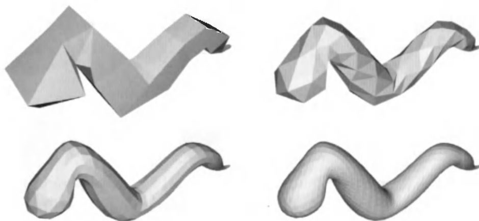
Figure 13.46. A worm is subdivided three times with the \sqrt{3} -subdivision scheme.
