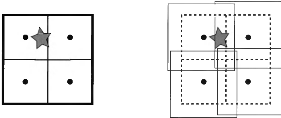
Figure 14.6. An ordinary octree compared to a loose octree. The dots indicate the center points of the boxes (in the first subdivision). To the left, the star pierces through one splitting plane of the ordinary octree. Thus, one choice is to put the star in the largest box (that of the root). To the right, a loose octree with k = 1.5 (that is, boxes are 50% larger) is shown. The boxes are slightly displaced, so that they can be discerned. The star can now be placed fully in the upper left box.
