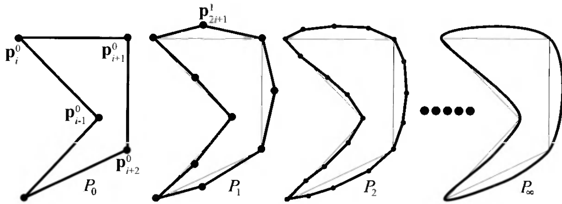
Figure 13.30. The 4-point subdivision scheme in action. This is an interpolating scheme as the curve goes through the initial points, and in general curve P_{i+1} goes through the points of P_i . Note that the same control polygon is used in Figure 13.29.
