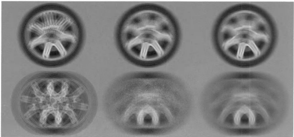
Figure 18.22. The top row shows a slowly rotating and translating wheel, while the bottom row shows a faster-moving wheel. The left column was rendered by accumulating four different images. The middle column was rendered with four samples using a new stochastic rasterizer targeting new GPU hardware, and the right column is a reference rendering with 64 jittered samples.
