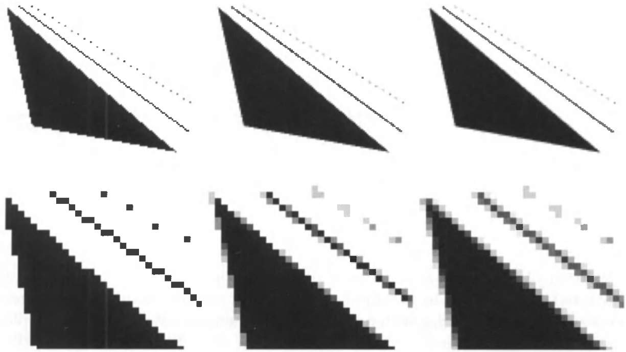
Figure 5.18. The upper row shows three images with different levels of antialiasing of a triangle, a line, and some points. The lower row images are magnifications of the upper row. The leftmost column uses only one sample per pixel, which means that no antialiasing is used. The middle column images were rendered with four samples per pixel (in a grid pattern), and the right column used eight samples per pixel (in a 4 \times 4 checkerboard). All images were rendered using InfiniteReality graphics [899].
