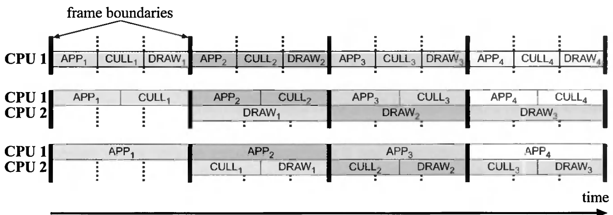
Figure 15.7. Different configurations for a multiprocessor pipeline. The thick lines represent synchronization between the stages, and the subscripts represent the frame number. At the top, a single CPU pipeline is shown. In the middle and at the bottom are shown two different pipeline subdivisions using two CPUs. The middle has one pipeline stage for APP and CULL and one pipeline stage for DRAW. This is a suitable subdivision if DRAW has much more work to do than the others. At the bottom, APP has one pipeline stage and the other two have another. This is suitable if APP has much more work than the others. Note that the bottom two configurations have more time for the APP, CULL, and DRAW stages.
