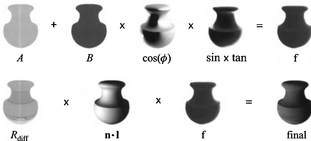
Figure 7.41. Visualization of simplified Oren-Nayar shading. The \sin \times \tan and f (BRDF) values extend beyond 1 and are visualized using a false-color ramp (black is 0, red is 1, yellow is 2 and white is 3). (Images courtesy of Michal Valient [1285, 1286].)
