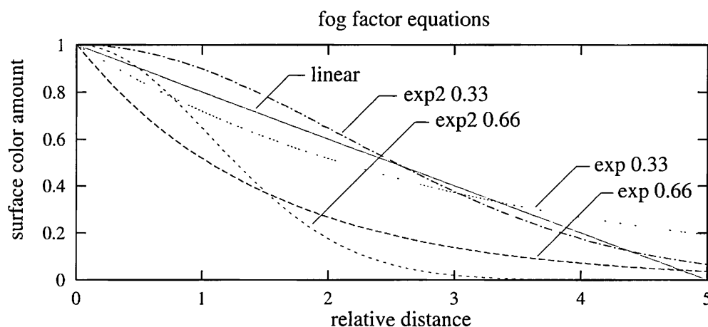
Figure 10.38. Curves for fog fall-off: linear, exponential, and squared-exponential, using various densities.
