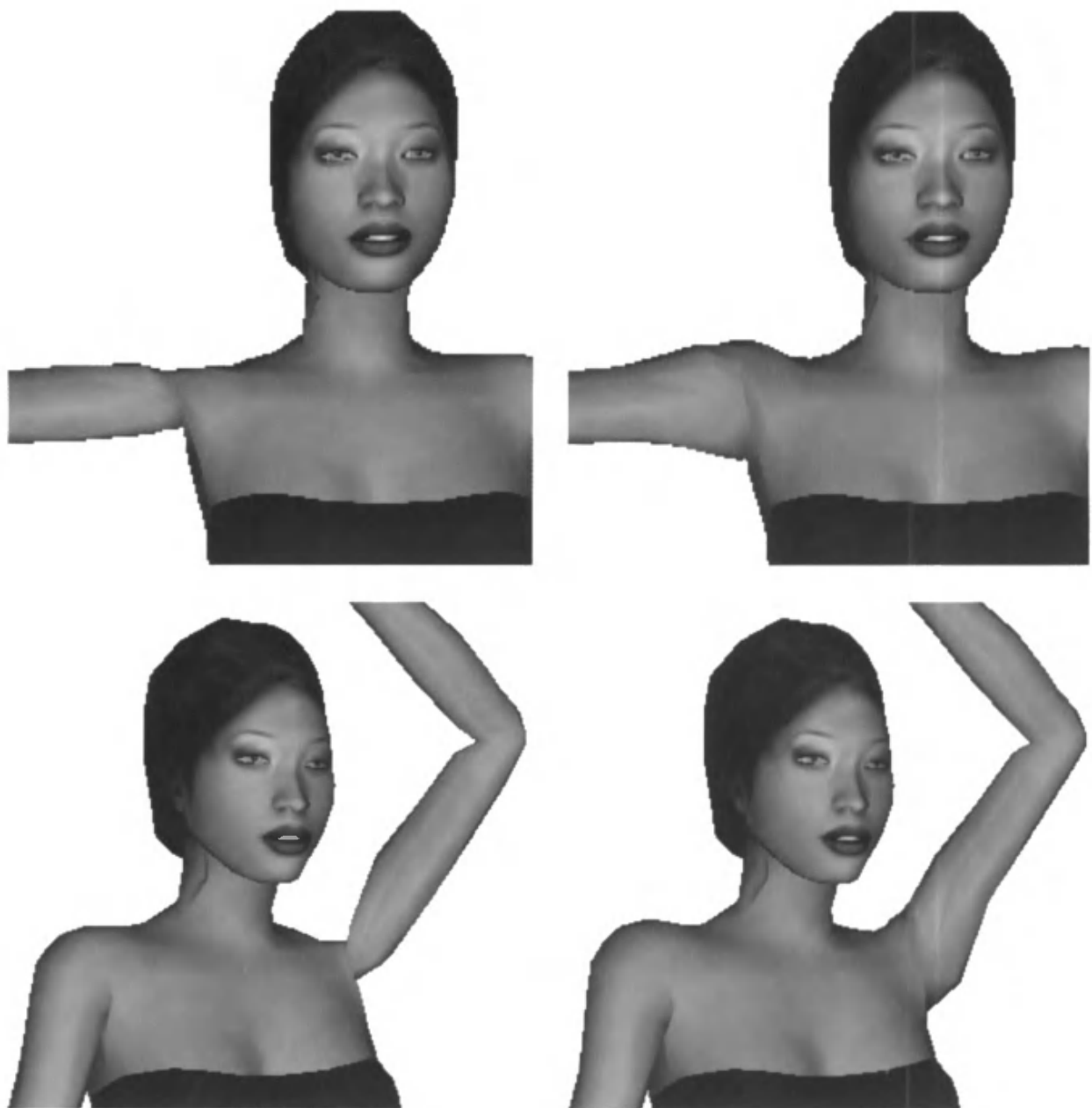
Figure 4.12. The left side shows problems at the joints when using linear blend skinning. On the right, blending using dual quaternions improves the appearance. ( Images courtesy of Ladislav Kavan et al., model by Paul Steed [1218]. )
