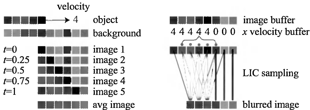
Figure 10.35. On the left an accumulation buffer rendering is visualized. The red set of pixels represents an object moving four pixels to the right over a single frame. The results for six pixels over the five frames are averaged to get the final, correct result at the bottom. On the right, an image and x direction velocity buffer are generated at time 0.5 (the y velocity buffer values are all zeroes, since there is no vertical movement). The velocity buffer is then used to determine how the image buffer is sampled. For example, the green annotations show how the velocity buffer speed of 4 causes the sampling kernel to be four pixels wide. For simplicity of visualization, five samples, one per pixel, are taken and averaged. In reality, the samples usually do not align on pixel centers, but rather are taken at equal intervals along the width of the kernel. Note how the three background pixels with a velocity of 0 will take all five samples from the same location.
