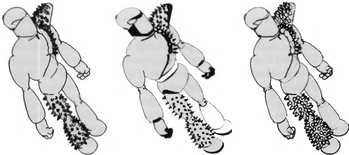
Figure 11.8. Silhouettes rendered with backfacing edge drawing with thick lines, z -bias, and fattened triangle algorithms. The backface edge technique gives poor joins between lines and nonuniform lines due to biasing problems on small features. The z -bias technique gives nonuniform edge width because of the dependence on the angles of the frontfaces. (Images courtesy of Raskar and Cohen [1046].)
