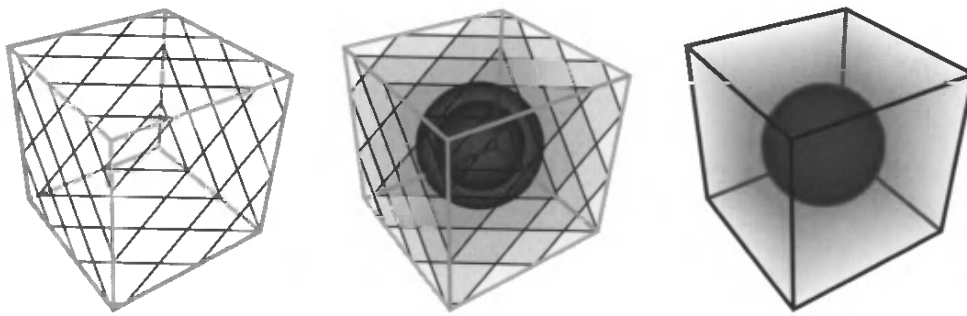
Figure 10.41. A volume is rendered by a series of slices parallel to the view plane. Some slices and their intersection with the volume are shown on the left. The middle shows the result of rendering just these slices. On the right the result is shown when a large series of slices are rendered and blended. ( Figures courtesy of Christof Rezk-Salama, University of Siegen, Germany. )
