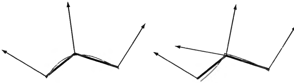
Figure 5.14. Side views of triangle meshes (in black, with vertex normals) representing curved surfaces (in red). On the left smoothed vertex normals are used to represent a smooth surface. On the right the middle vertex has been duplicated and given two normals, representing a crease.
