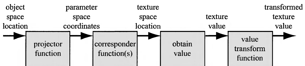
Figure 6.2. The generalized texture pipeline for a single texture.
