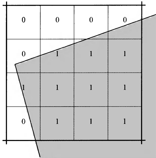
Figure 5.31. The corner of a polygon partially covers a single screen grid cell associated with a pixel. The grid cell is shown subdivided into a 4 \times 4 subgrid, and those cells that are considered covered are marked by a 1. The 16-bit mask for this cell is 0000 0111 1111 0111.
