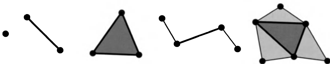
Figure 3.6. Geometry shader input for a geometry shader program is of some single type: point, line segment, triangle. The two rightmost primitives, which include vertices adjacent to the line and triangle objects, can also be used.
