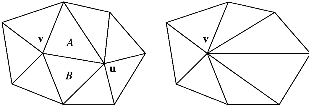
Figure 12.21. On the left is the figure before the uv edge collapse occurs; the right figure shows point u collapsed into point v , thereby removing triangles A and B and edge uv .
