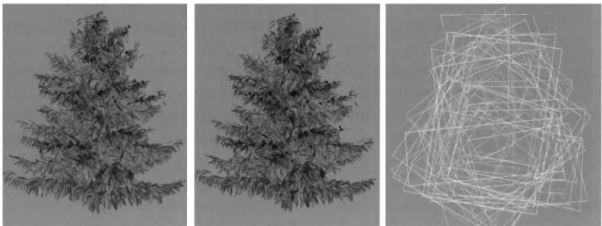
Figure 10.16. On the left, a tree model made of 20,610 triangles. In the middle, the tree modeled with 78 billboards. The overlapping billboards are shown on the right. ( Images courtesy of Dylan Lacewell, University of Utah. )
