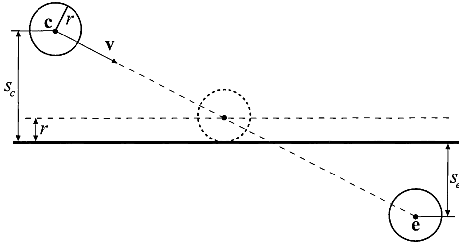
Figure 16.28. The notation used in the dynamic sphere/plane intersection test. The middle sphere shows the position of the sphere at the time when collision occurs. Note that s_c and s_e are both signed distances.
