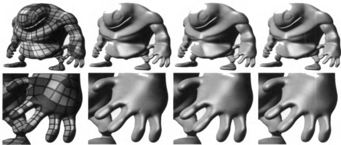
Figure 13.65. Left: quad structure of a mesh. White quads are ordinary, green have one extraordinary vertex, and blue have more than one. Mid-left: geometry path approximation. Mid-right: geometry patches with tangent patches. Note that the obvious shading artifacts disappeared. Right: true Catmull-Clark surface. (Image courtesy of Charles Loop and Scott Schaefer, reprinted with permission from Microsoft Corporation.)
