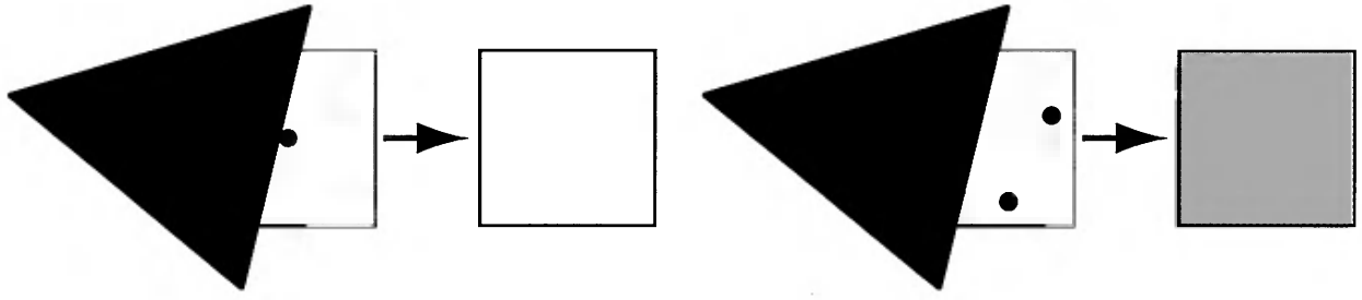
Figure 5.28. On the left, a red triangle is rendered with one sample at the center of the pixel. Since the triangle does not cover the sample, the pixel will be white, even though a substantial part of the pixel is covered by the red triangle. On the right, four samples are used per pixel, and as can be seen, two of these are covered by the red triangle, which results in a pink pixel color.
