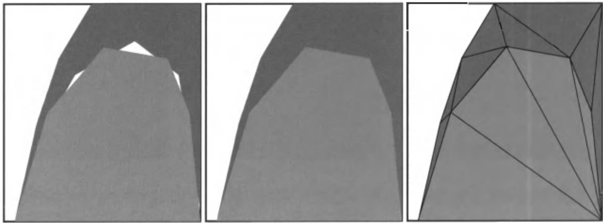
Figure 12.7. The left figure shows cracking where the two surfaces meet. The middle shows the cracking fixed by matching up edge points. The right shows the corrected mesh.
