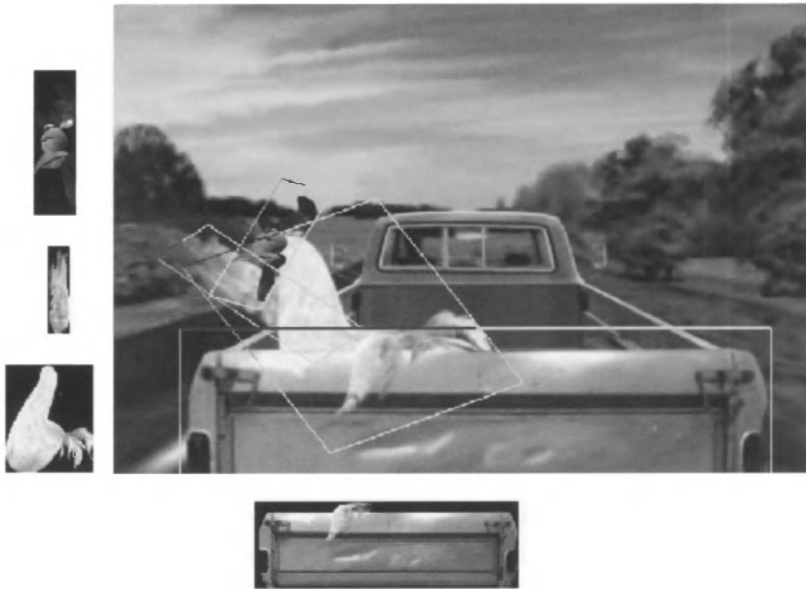
Figure 10.3. A still from the animation Chicken Crossing , rendered using a Talisman simulator. In this scene, 80 layers of sprites are used, some of which are outlined and shown on the left. Since the chicken wing is partially in front of and behind the tailgate, both were placed in a single sprite. (Reprinted with permission from Microsoft Corporation.)
