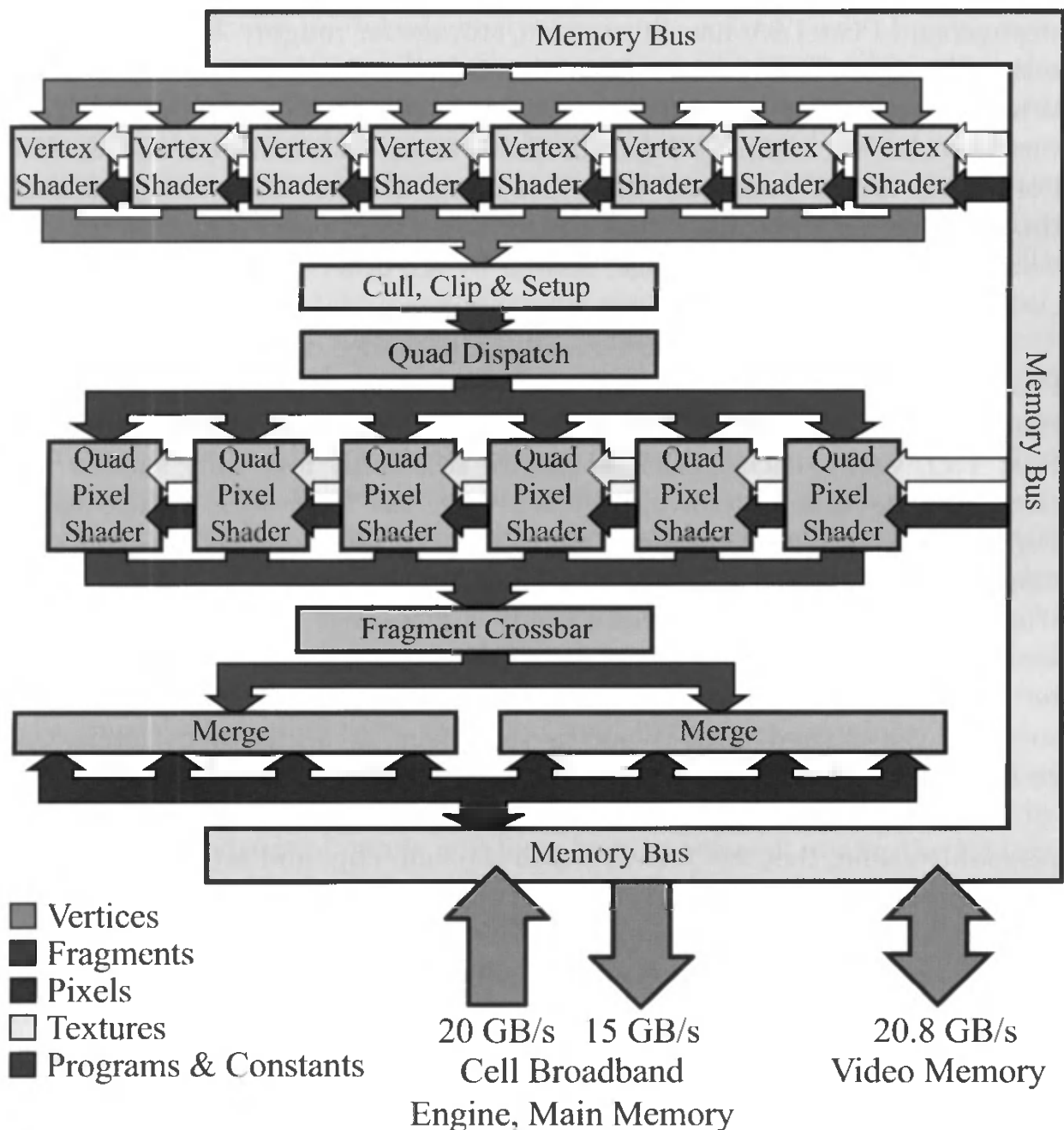
Figure 18.18. RSX architecture.
