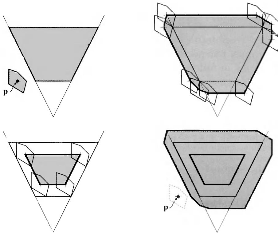
Figure 16.23. The upper left image shows a frustum (blue) and a general bounding volume (green), where a point p relative to the object has been selected. By tracing the point p where the object moves on the outside (upper right) and on the inside (lower left) of the frustum, as close as possible to the frustum, the frustum/BV can be reformulated into testing the point p against an outer and an inner volume. This is shown on the lower right. If the point p is outside the orange volume, then the BV is outside the frustum. The BV intersects the frustum if p is inside the orange area, and the BV is fully inside the frustum if p is inside the violet area.
