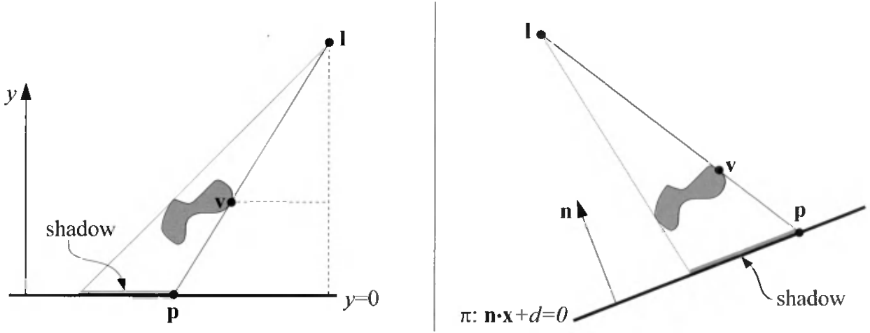
Figure 9.5. Left: A light source, located at \mathbf{l} , casts a shadow onto the plane y = 0 . The vertex \mathbf{v} is projected onto the plane. The projected point is called \mathbf{p} . The similar triangles are used for the derivation of the projection matrix. Right: The notation of the left part of this figure is used here. The shadow is being cast onto a plane, \pi : \mathbf{n} \cdot \mathbf{x} + d = 0 .
