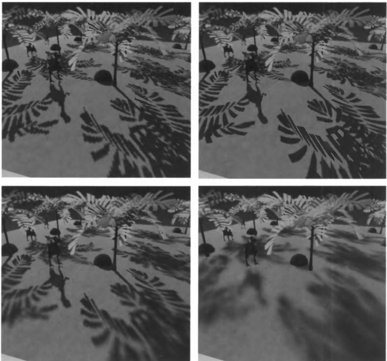
Figure 9.32. In the upper left, standard shadow mapping. Upper right, perspective shadow mapping, increasing the density of shadow map texel density near the viewer. Lower left, percentage-closer soft shadows, softening the shadows as the occluder's distance from the receiver increases. Lower right, variance shadow mapping with a constant soft shadow width, each pixel shaded with a single variance map sample. (Images courtesy of Nico Hempe, Yvonne Jung, and Johannes Behr.)
