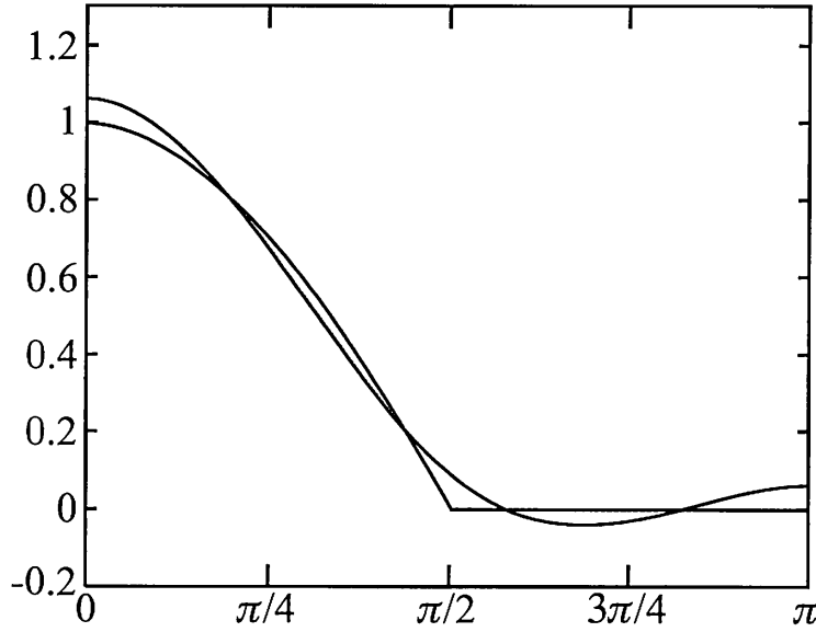
Figure 8.28. The clamped cosine function (in red) versus its nine-coefficient spherical harmonic approximation (in blue). The approximation is quite close. Note the slight dip below and the rise above zero between \pi/2 and \pi .
