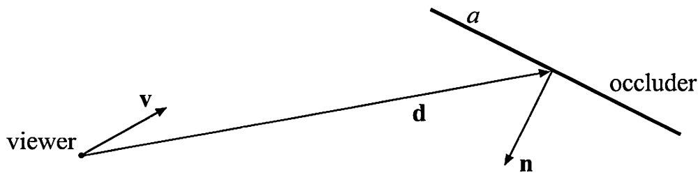
Figure 14.29. The geometry involved in the estimation of the solid angle.
