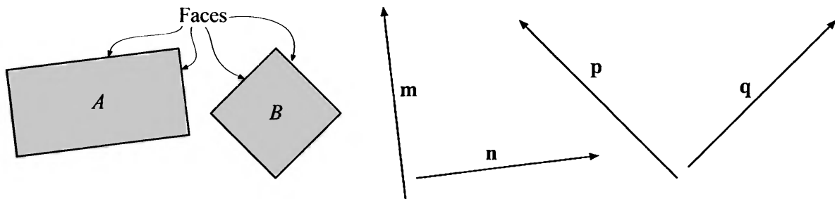
Figure 16.20. To determine whether two OBBs A and B overlap, the separating axis test can be used. Here, it is shown in two dimensions. The separating axes should be orthogonal to the faces of A and B . The axes \mathbf{m} and \mathbf{n} are orthogonal to the faces of A , and \mathbf{p} and \mathbf{q} are orthogonal to the faces of B . The OBBs are then projected onto the axes. If both projections overlap on all axes, then the OBBs overlap; otherwise, they do not. So it is sufficient to find one axis that separates the projections in order to know that the OBBs do not overlap. In this example, the \mathbf{n} axis is the only axis that separates the projections.
