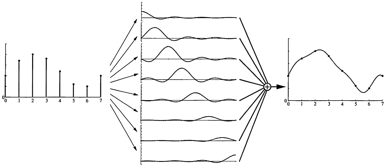
Figure 5.25. Here, the sinc filter is used to reconstruct the signal. The sinc filter is the ideal lowpass filter.
