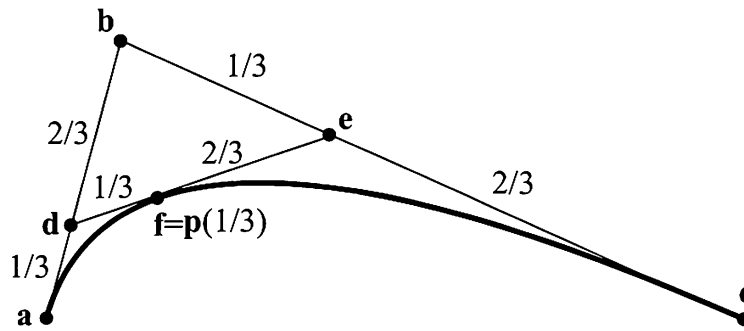
Figure 13.3. Repeated linear interpolation gives a Bézier curve. This curve is defined by three control points, \mathbf{a} , \mathbf{b} , and \mathbf{c} . Assuming we want to find the point on the curve for the parameter t = 1/3 , we first linearly interpolate between \mathbf{a} and \mathbf{b} to get \mathbf{d} . Next, \mathbf{e} is interpolated from \mathbf{b} and \mathbf{c} . The final point, \mathbf{p}(1/3) = \mathbf{f} is found by interpolating between \mathbf{d} and \mathbf{e} .
