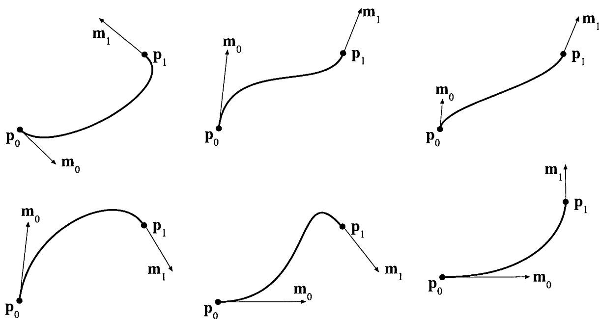
Figure 13.11. Hermite interpolation. A curve is defined by two points, \mathbf{p}_0 and \mathbf{p}_1 , and a tangent, \mathbf{m}_0 and \mathbf{m}_1 , at each point.
