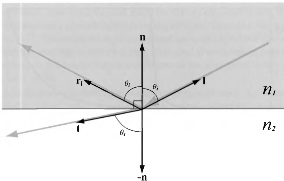
Figure 7.21. Internal reflection at a planar surface.
