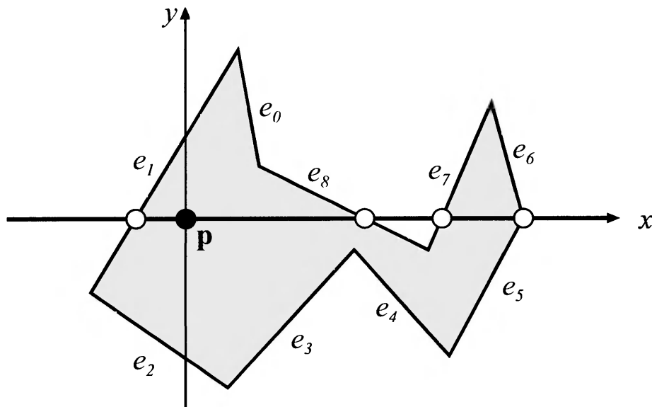
Figure 16.13. The polygon has been translated by -\mathbf{p} ( \mathbf{p} is the point to be tested for containment in the polygon), and so the number of crossings with the positive x -axis determines whether \mathbf{p} is inside the polygon. Edges e_0 , e_2 , e_3 , and e_4 do not cross the x -axis. The intersection between edge e_1 and the x -axis must be computed, but will not yield a crossing, since the intersection has a negative x -component. Edges e_7 and e_8 will each increase the number of crossings, since the vertices of these edges have positive x -components and one negative and one positive y -component. Finally, the edges e_5 and e_6 share a vertex where y = 0 and x > 0 , and they will together increase the number of crossings by one. By considering vertices on the x -axis as above the ray, e_5 is classified as crossing the ray, e_6 as above the ray.
