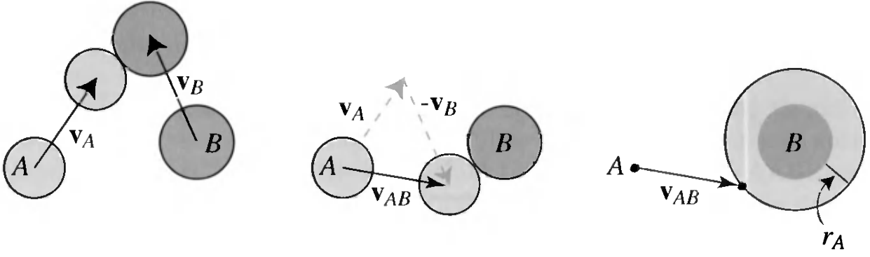
Figure 16.29. The left figure shows two spheres moving and colliding. In the center figure, sphere B has been made static by subtracting its velocity from both spheres. Note that the relative positions of the spheres at the collision point remains the same. On the right, the radius r_A of sphere A is added to B and subtracted from itself, making the moving sphere A into a ray.
