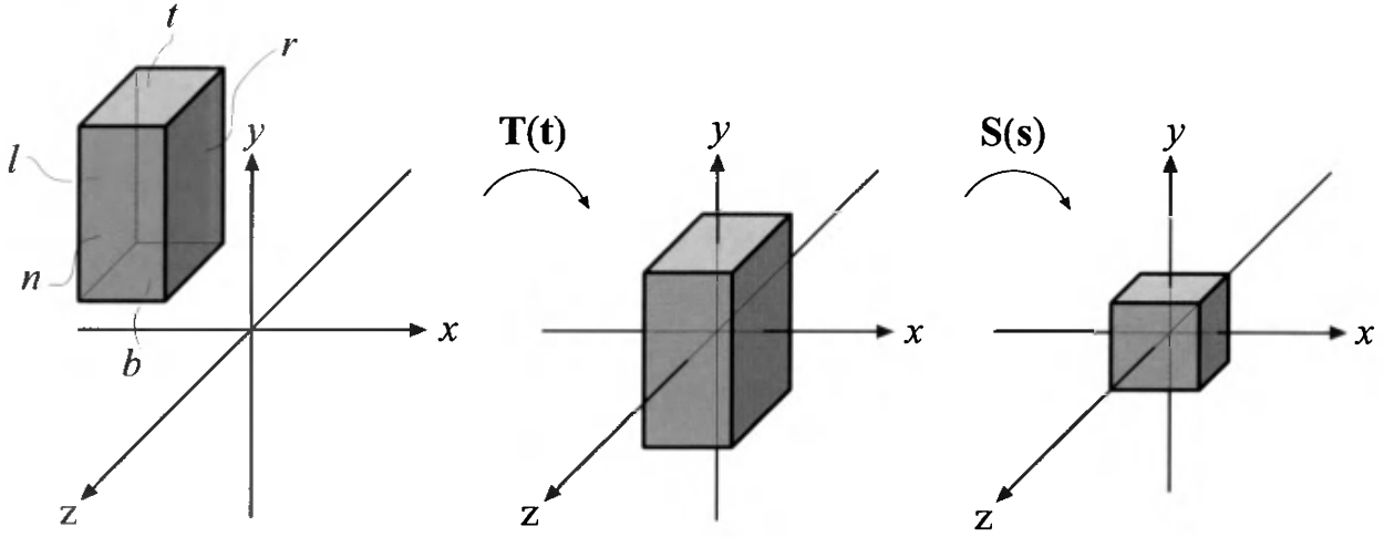
Figure 4.17. Transforming an axis-aligned box on the canonical view volume. The box on the left is first translated, making its center coincide with the origin. Then it is scaled to get the size of the canonical view volume, shown at the right.
