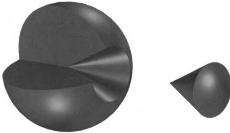
Figure 7.3. A cone with a solid angle of one steradian removed from a cutaway view of a sphere. The shape itself is irrelevant to the measurement; the coverage on the sphere’s surface is the key.
