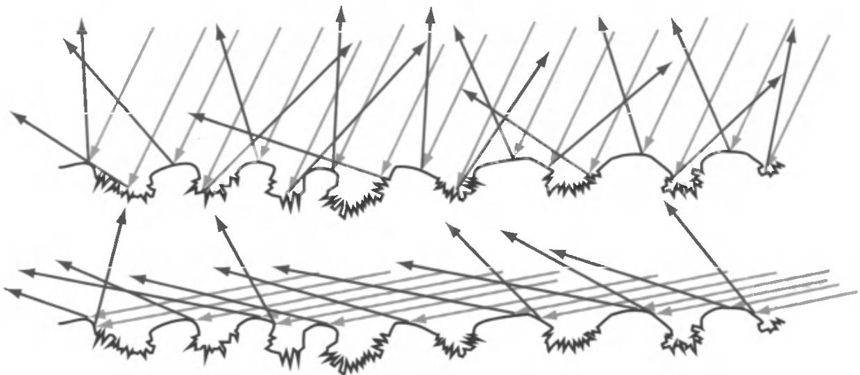
Figure 7.27. Microgeometry with a strong correlation between height and surface normal (raised areas are smooth, lower areas are rough). In the top image, the surface is illuminated from an angle close to the macroscopic surface normal. At this angle, the rough pits are accessible to many of the incoming light rays, and many of them are scattered in different directions. In the bottom image, the surface is illuminated from a glancing angle. Shadowing blocks most of the pits, so few light rays hit them, and most rays are reflected from the smooth parts of the surface. In this case, the apparent roughness depends strongly on the angle of illumination.
