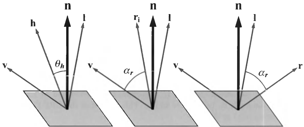
Figure 7.32. On the left, the angle \theta_h between the macroscopic surface normal \mathbf{n} and the half vector \mathbf{h} is shown. This angle is used in isotropic microfacet BRDFs. In the middle, the reflection vector \mathbf{r}_i and view vector \mathbf{v} define the angle \alpha_r . This angle is sometimes used in BRDFs instead of \theta_h . On the right, an alternative definition of \alpha_r , between the reflected view vector \mathbf{r} and \mathbf{l} . Due to symmetry, the same value of \alpha_r is obtained.
