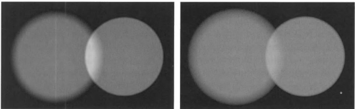
Figure 5.39. Two overlapping spotlights illuminating a plane. In the left image, the light values have been combined in a nonlinear space (i.e., gamma correction was not performed). In the right image, proper gamma correction has resulted in the light values being combined in linear space. Note the overbrightening of the overlap region in the left image; the right image is correct.
