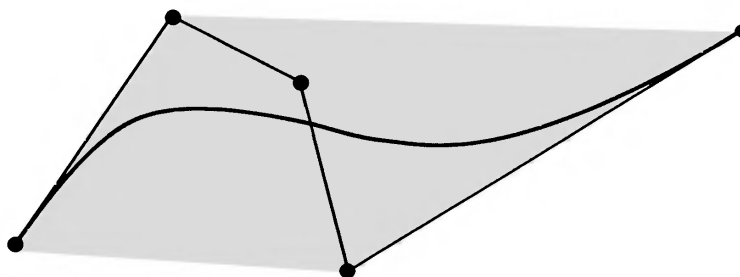
Figure 13.4. Repeated linear interpolation from five points gives a fourth degree (quartic) Bézier curve. The curve is inside the convex hull (gray region), of the control points, marked by black dots. Also, at the first point, the curve is tangent to the line between the first and second point. The same also holds for the other end of the curve.
