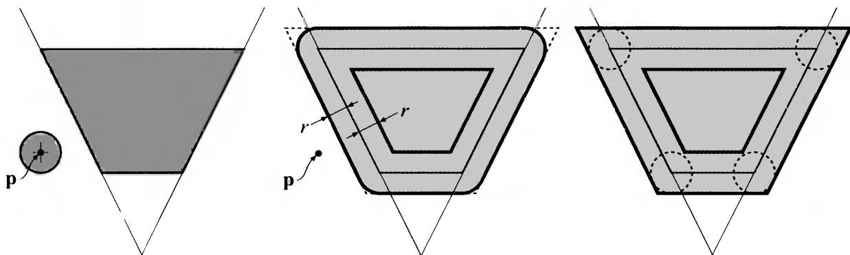
Figure 16.24. At the left, a frustum and a sphere are shown. The exact frustum/sphere test can be formulated as testing p against the orange and violet volumes in the middle figure. At the right is a reasonable approximation of the volumes in the middle. If the center of the sphere is located outside a rounded corner, but inside all outer planes, it will be incorrectly classified as intersecting, even though it is outside the frustum.
