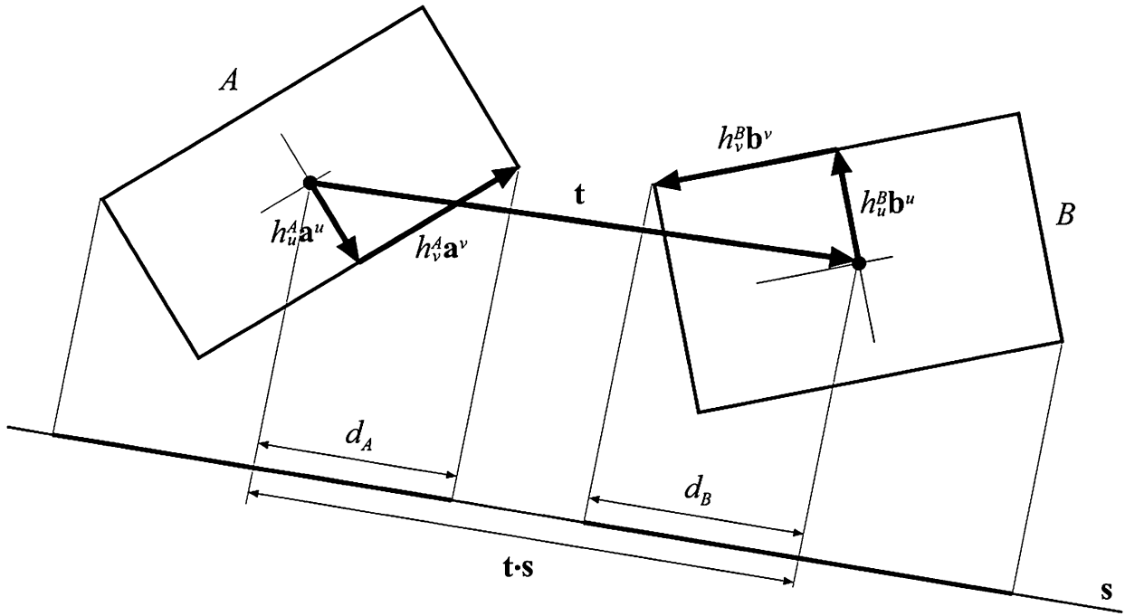
Figure 16.21. The separating axis test illustrated. The two OBBs, A and B , are disjoint, since the projections of their “radii” on the axis determined by s are not overlapping. (Illustration after Gottschalk et al. [433].)
