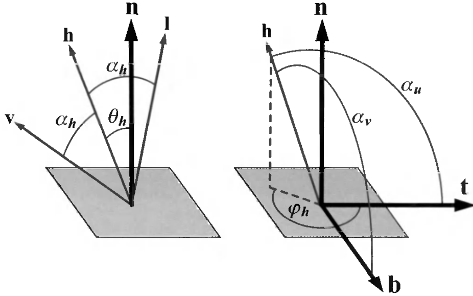
Figure 7.31. Angles relating to the half vector. On the left, the half vector \mathbf{h} lies halfway between \mathbf{v} and \mathbf{l} , all in the same plane, and defines \alpha_h . This is the incidence angle for the microfacets and is used to compute Fresnel reflectance. Here, \theta_h is the angle between \mathbf{h} and \mathbf{n} and is used for evaluating NDFs, isotropic ones in particular. On the right, \phi_h , \alpha_u , and \alpha_v give the orientation of \mathbf{h} relative to the tangent vector \mathbf{t} and the bitangent vector \mathbf{b} . These are used for evaluating anisotropic NDFs.
