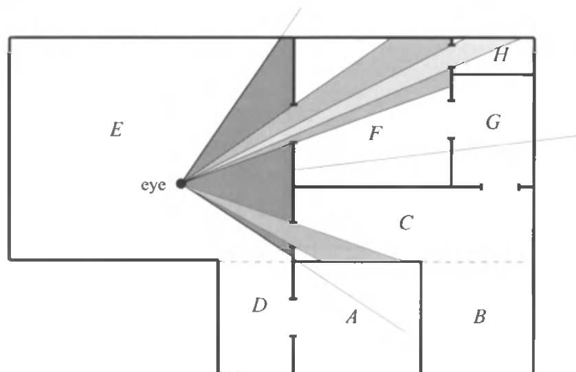
Figure 14.13. Portal culling: Cells are enumerated from A to H , and portals are openings that connect the cells. Only geometry seen through the portals is rendered.
