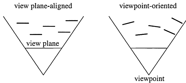
Figure 10.6. A top view of the two billboard alignment techniques. The five billboards face differently, depending on the method.
