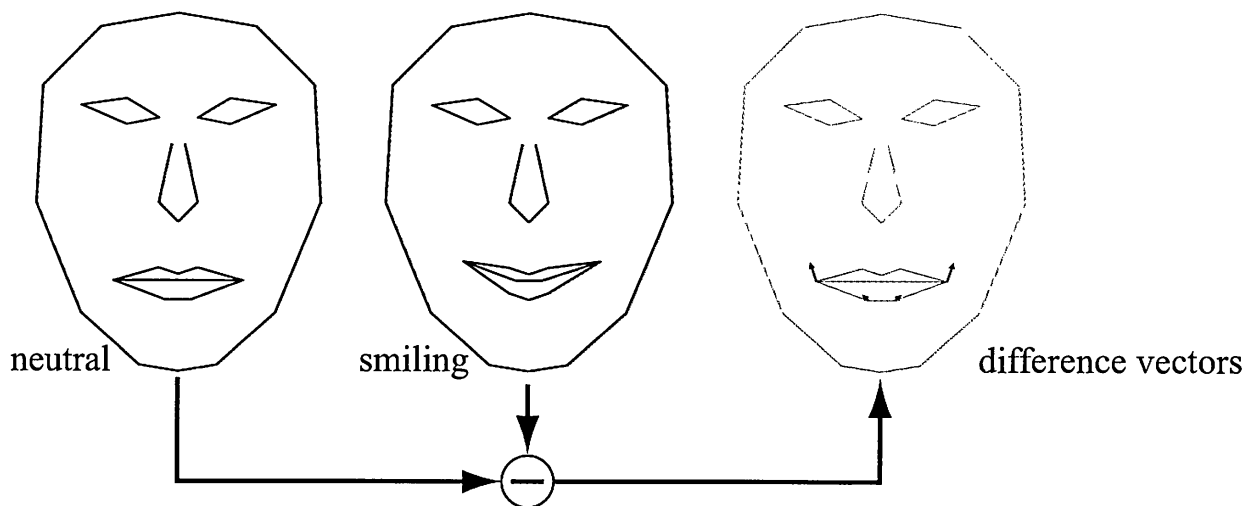
Figure 4.14. Given two mouth poses, a set of difference vectors is computed to control interpolation, or even extrapolation. In morph targets, the difference vectors are used to “add” movements onto the neutral face. With positive weights for the difference vectors, we get a smiling mouth, while negative weights can give the opposite effect.
