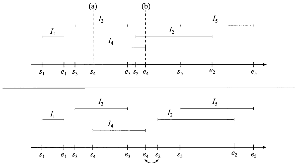
Figure 17.11. At the top, the interval I_4 is encountered (at the point marked (a)) when there is only one interval in the active list ( I_3 ), so it is concluded that I_4 and I_3 overlap. When I_2 is encountered, I_4 is still in the active list (since e_4 has not been encountered yet), and so I_4 and I_2 also overlap. When e_4 is encountered, I_4 is removed (at the point marked (b)) from the active list. At the bottom, I_2 has moved to the right, and when the insertion sort finds that s_2 and e_4 need to change places, it can also be concluded that I_2 and I_4 do not overlap any longer. (Illustration after Witkin et al. [1363].)
