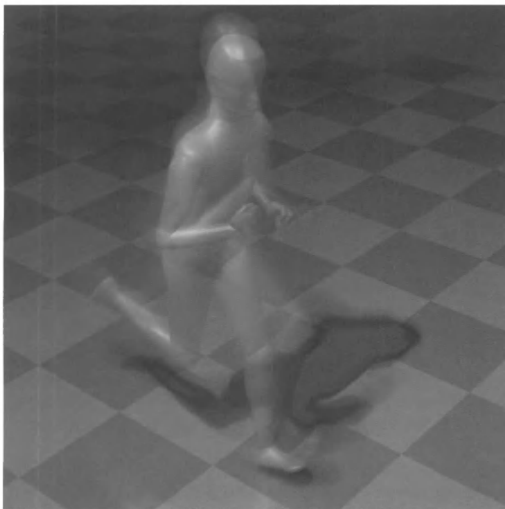
Figure 10.33. Motion blur done using the accumulation buffer. Note the ghosting on the arms and legs due to undersampling. Accumulating more images would result in a smoother blur.
