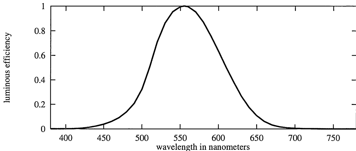
Figure 7.6. The photometric curve.
