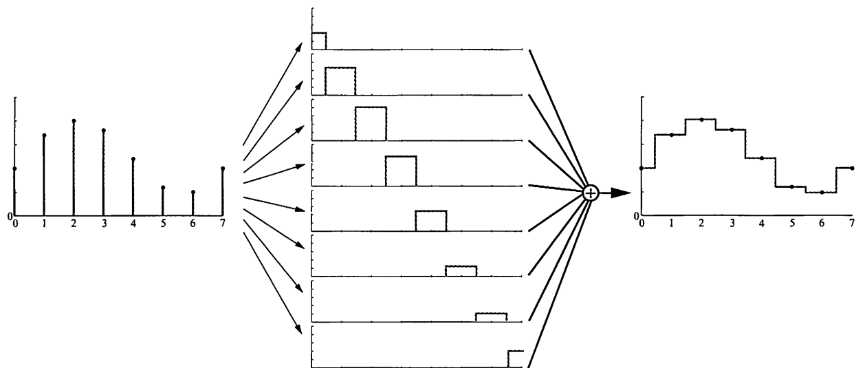
Figure 5.23. The sampled signal (left) is reconstructed using the box filter. This is done by placing the box filter (see Figure 5.22) over each sample point, and scaling it in the y -direction so that the height of the filter is the same as the sample point. The sum is the reconstruction signal (right).
