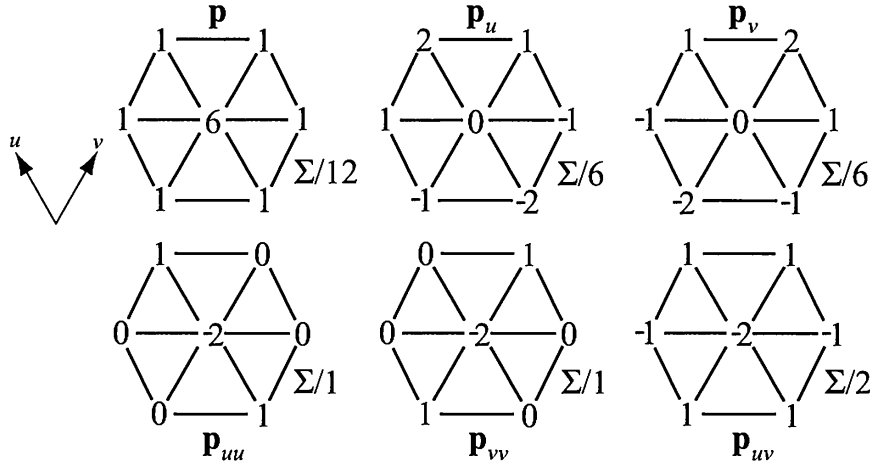
Figure 13.50. The masks for an ordinary vertex in Loop's subdivision scheme. Note that after using these masks, the resulting sum should be divided as shown. ( Illustration after Lee et al. [745]. )
