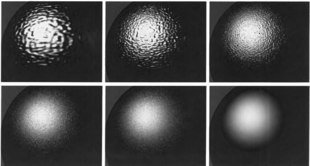
Figure 7.24. Gradual transition from visible detail to microscale. The sequence of images goes top row left to right, then bottom row left to right. The surface shape and lighting are constant; only the scale of the surface detail changes.
