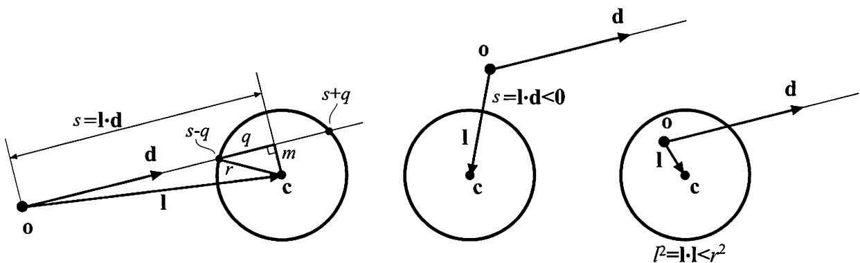
Figure 16.6. The notation for the geometry of the optimized ray/sphere intersection. In the left figure, the ray intersects the sphere in two points, where the distances are t = s \pm q along the ray. The middle case demonstrates a rejection made when the sphere is behind the ray origin. Finally, at the right, the ray origin is inside the sphere, in which case the ray always hits the sphere.
