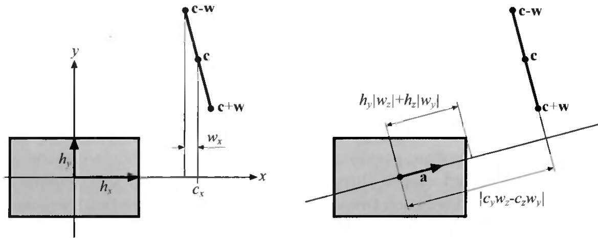
Figure 16.8. Left: The x -axis is tested for overlap between the box and the line segment. Right: The \mathbf{a} -axis is tested. Note that h_y|w_z| + h_z|w_y| and |c_y w_z - c_z w_y| are shown in this illustration as if \mathbf{w} is normalized. When this is not the case, then both the shown values should be scaled with \|\mathbf{w}\| . See text for notation.
