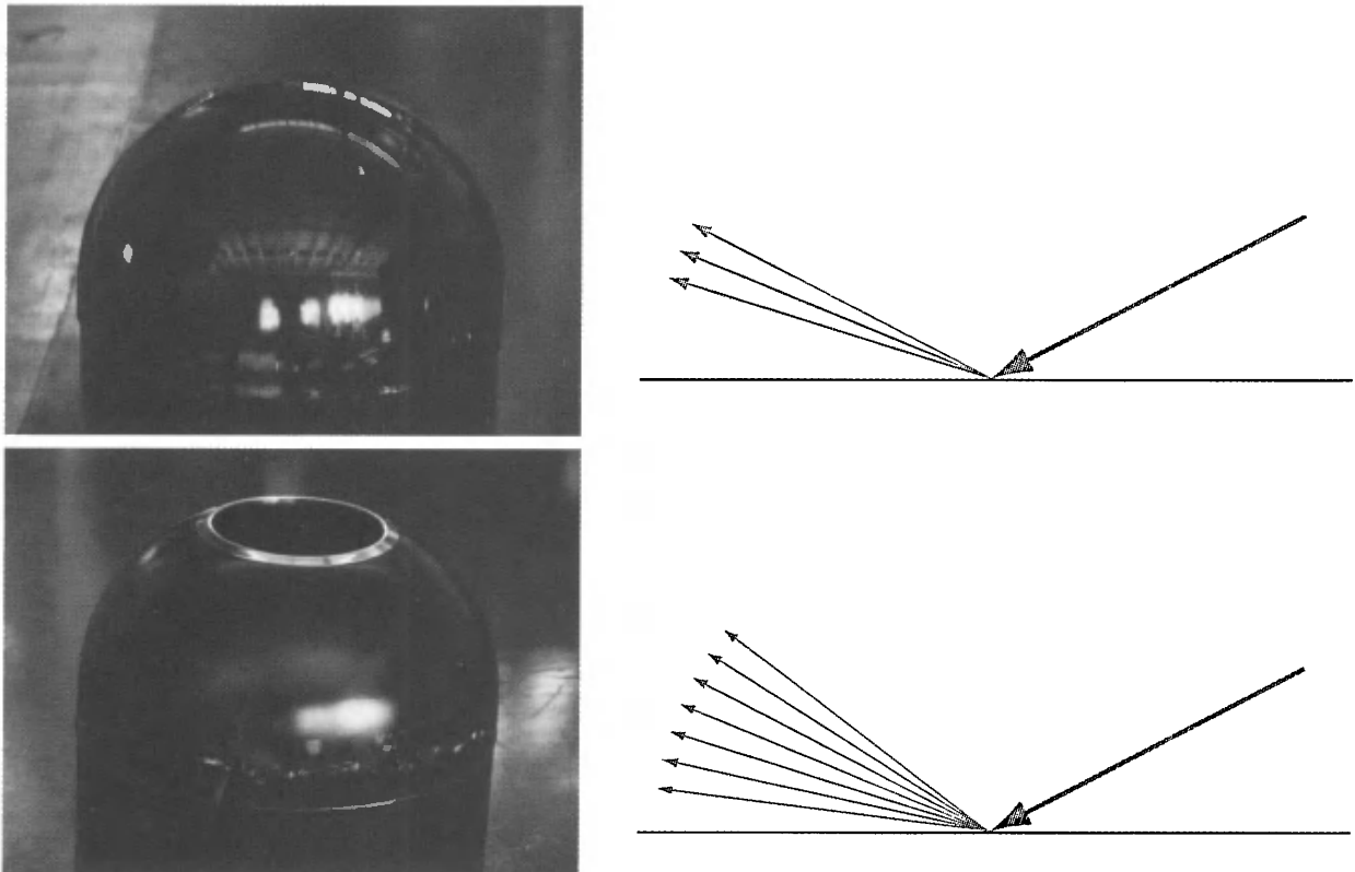
Figure 5.8. Light reflecting off surfaces of different smoothness.
