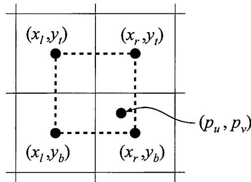
Figure 6.9. Notation for bilinear interpolation. The four texels involved are illustrated by the four squares.
