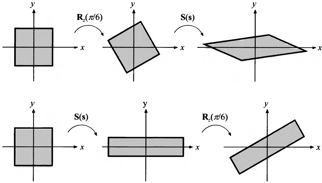
Figure 4.4. This illustrates the order dependency when multiplying matrices. In the top row, the rotation matrix R_z(\pi/6) is applied followed by a scaling, S(s) , where s = (2, 0.5, 1) . The composite matrix is then S(s)R_z(\pi/6) . In the bottom row, the matrices are applied in the reverse order, yielding R_z(\pi/6)S(s) . The results are clearly different. It generally holds that MN \neq NM , for arbitrary matrices M and N .
