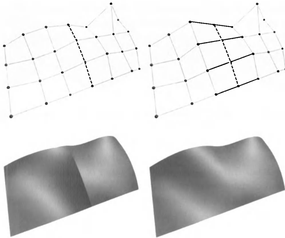
Figure 13.26. The left column shows two Bézier patches joined with only C^0 continuity. Clearly, there is a shading discontinuity between the patches. The right column shows similar patches joined with C^1 continuity, which looks better. In the top row, the dashed lines indicate the border between the two joined patches. To the upper right, the black lines show the collinearity of the control points of the joining patches.
