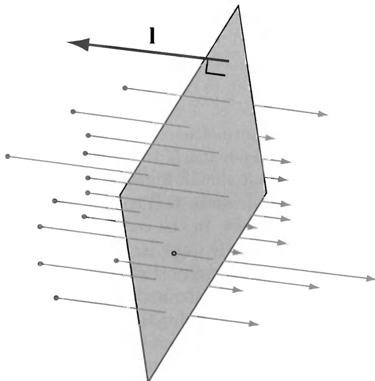
Figure 5.3. Measuring the magnitude of light emitted by a directional light source.
