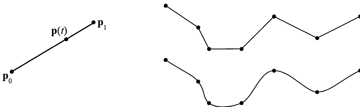
Figure 13.2. Linear interpolation between two points is the path on a straight line (left). For seven points, linear interpolation is shown at the upper right, and some sort of smoother interpolation is shown at the lower right. What is most objectionable about using linear interpolation are the discontinuous changes (sudden jerks) at the joints between the linear segments.
