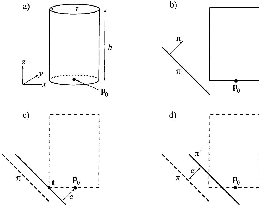
Figure 17.4. Figure (a) shows a cylinder with height h , radius r , and reference point \mathbf{p}_0 . The sequence (b)-(d) then shows how testing a plane, \pi , against a cylinder (shown from the side) can be recast into testing a point \mathbf{p}_0 against a new plane \pi' .
