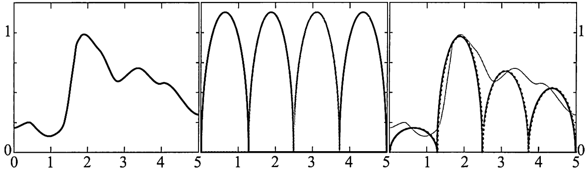
Figure 8.26. Orthonormal basis functions. This example uses the same space and target function as Figure 8.25, but the basis functions have been modified to be orthonormal. The left side shows the target function, the middle shows the orthonormal set of basis functions, and the right side shows the scaled basis functions. The resulting approximation to the target function is shown as a dotted black line, and the original function is shown in gray for comparison.
