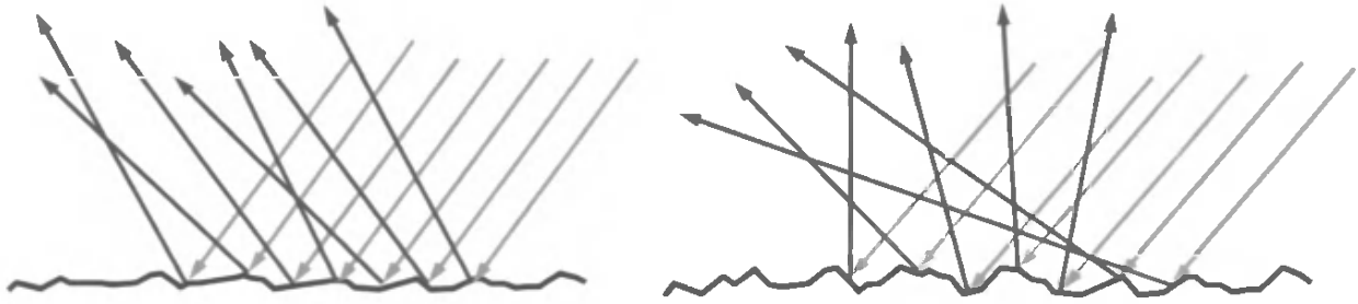
Figure 7.23. Light reflecting from two surfaces: a slightly rough surface on the left and a considerably rougher surface on the right.
