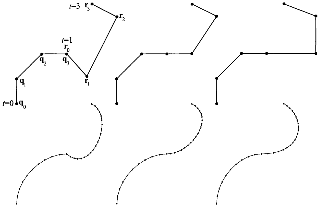
Figure 13.9. This figure shows from left to right C^0 , G^1 , and C^1 continuity between two cubic Bézier curves (four control points each). The top row shows the control points, and the bottom row the curves, with 10 sample points for the left curve, and 20 for the right. The following time-point pairs are used for this example: (0.0, \mathbf{q}_0) , (1.0, \mathbf{q}_3) , and (3.0, \mathbf{r}_3) . With C^0 continuity, there is a sudden jerk at the join (where \mathbf{q}_3 = \mathbf{r}_0 ). This is improved with G^1 by making the tangents at the join parallel (and equal in length). Though, since 3.0 - 1.0 \neq 1.0 - 0.0 , this does not give C^1 continuity. This can be seen at the join where there is a sudden acceleration of the sample points. To achieve C^1 , the right tangent at the join has to be twice as long as the left tangent.
