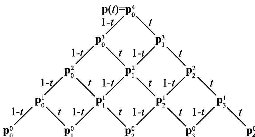
Figure 13.5. An illustration of how repeated linear interpolation works for Bézier curves. In this example, the interpolation of a quartic curve is shown. This means there are five control points, \mathbf{p}_i^0 , i = 0, 1, 2, 3, 4 , shown at the bottom. The diagram should be read from the bottom up, that is, \mathbf{p}_0^1 is formed from weighting \mathbf{p}_0^0 with weight 1-t and adding that with \mathbf{p}_1^0 weighted by t . This goes on until the point of the curve \mathbf{p}(t) is obtained at the top. (Illustration after Goldman [413].)
