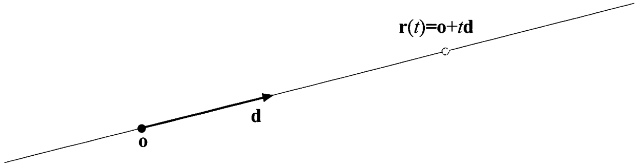
Figure 16.1. A simple ray and its parameters: \mathbf{o} (the ray origin), \mathbf{d} (the ray direction), and t , which generates different points on the ray, \mathbf{r}(t) = \mathbf{o} + t\mathbf{d} .
