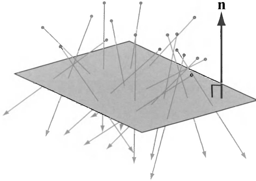
Figure 5.5. Irradiance measures light from all incoming directions.
