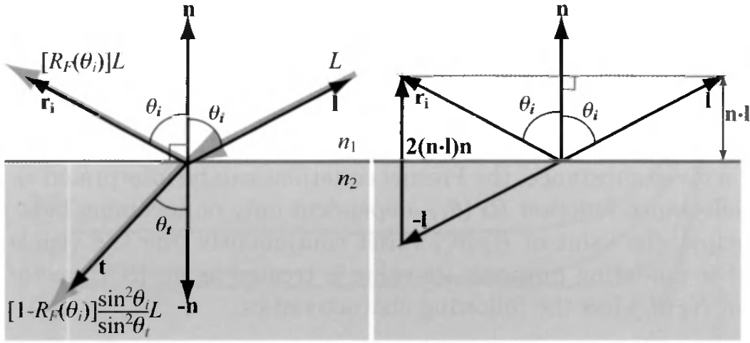
Figure 7.18. Reflection and refraction at a planar surface. The left side shows the indices of refraction n_1 and n_2 of the two substances, as well as the radiance and direction of the incoming, reflected, and refracted rays. The right side shows how the light vector \mathbf{l} is reflected around the normal \mathbf{n} in order to generate \mathbf{r}_i . First, \mathbf{l} is projected onto \mathbf{n} , and we get a scaled version of the normal: (\mathbf{n} \cdot \mathbf{l})\mathbf{n} . Then \mathbf{l} is negated, and if we add two times the projected vector, the reflection vector is obtained: \mathbf{r}_i = 2(\mathbf{n} \cdot \mathbf{l})\mathbf{n} - \mathbf{l} .
