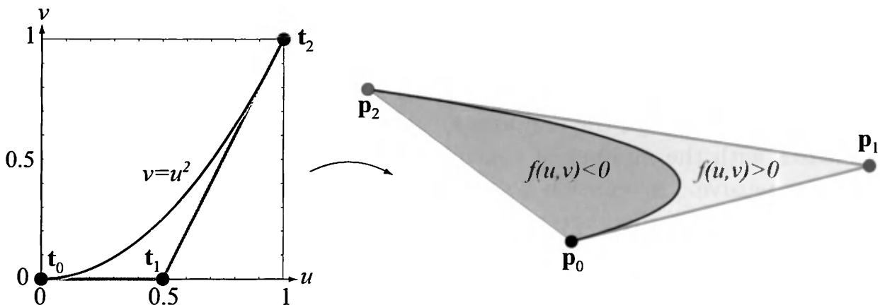
Figure 13.7. Bounded Bézier curve rendering. Left: The curve is shown in canonical texture space. Right: The curve is rendered in screenspace. If the condition f(u,v) \geq 0 is used to kill pixels, then the light blue region will result from the rendering.
