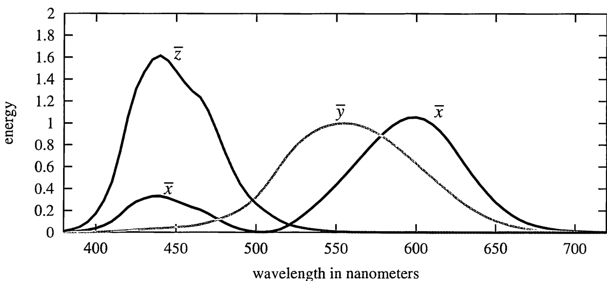
Figure 7.9. The Judd-Vos-modified CIE (1978) 2-degree color matching functions. Note that the two \bar{x} 's are part of the same curve. These color matching curves are not to be confused with the spectral distributions of the light sources used in the color matching experiment.
