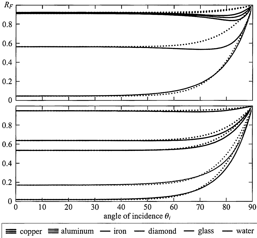
Figure 7.20. Schlick's approximation to Fresnel reflectance compared to the correct values for external reflection from a variety of substances (separated into two graphs for clarity). The solid lines were computed from the full Fresnel equations (in the case of copper and aluminum, this computation was performed at a dense sampling of frequencies and the resulting spectral distribution was converted to RGB values). The dotted lines are the result of Schlick's approximation (computed separately for R, G, and B in the case of copper and aluminum).
