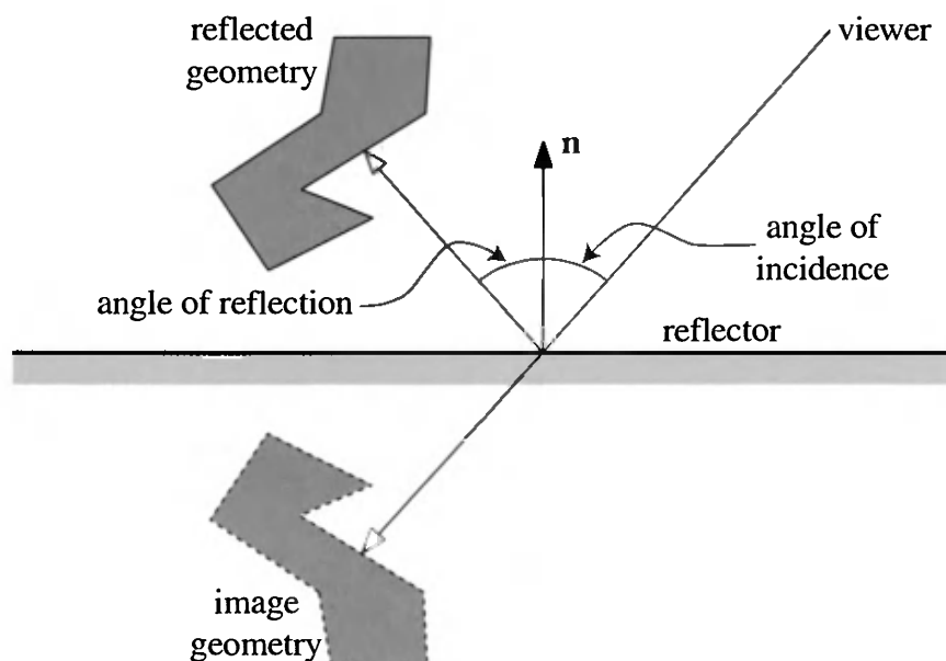
Figure 9.41. Reflection in a plane, showing angle of incidence and reflection, the reflected geometry, and the reflector.
