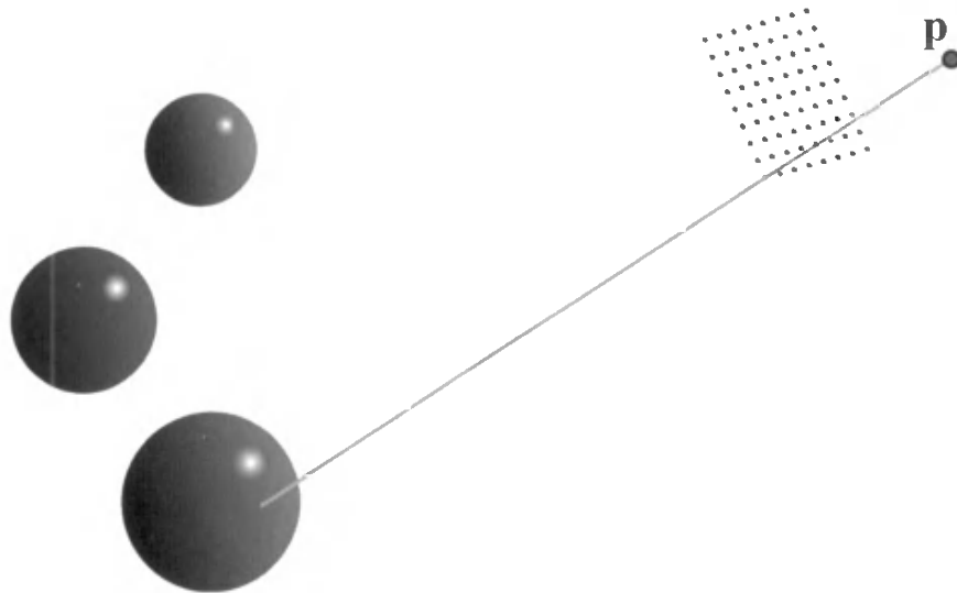
Figure 5.11. Idealized computer graphics model of imaging sensor.
