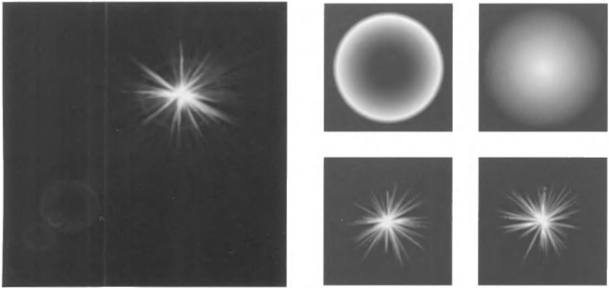
Figure 10.26. A lens flare and its constituent textures. On the right, a halo and a bloom are shown above, and two sparkle textures below. These textures are given color when rendered. ( Images from a Microsoft DirectX SDK program. )
