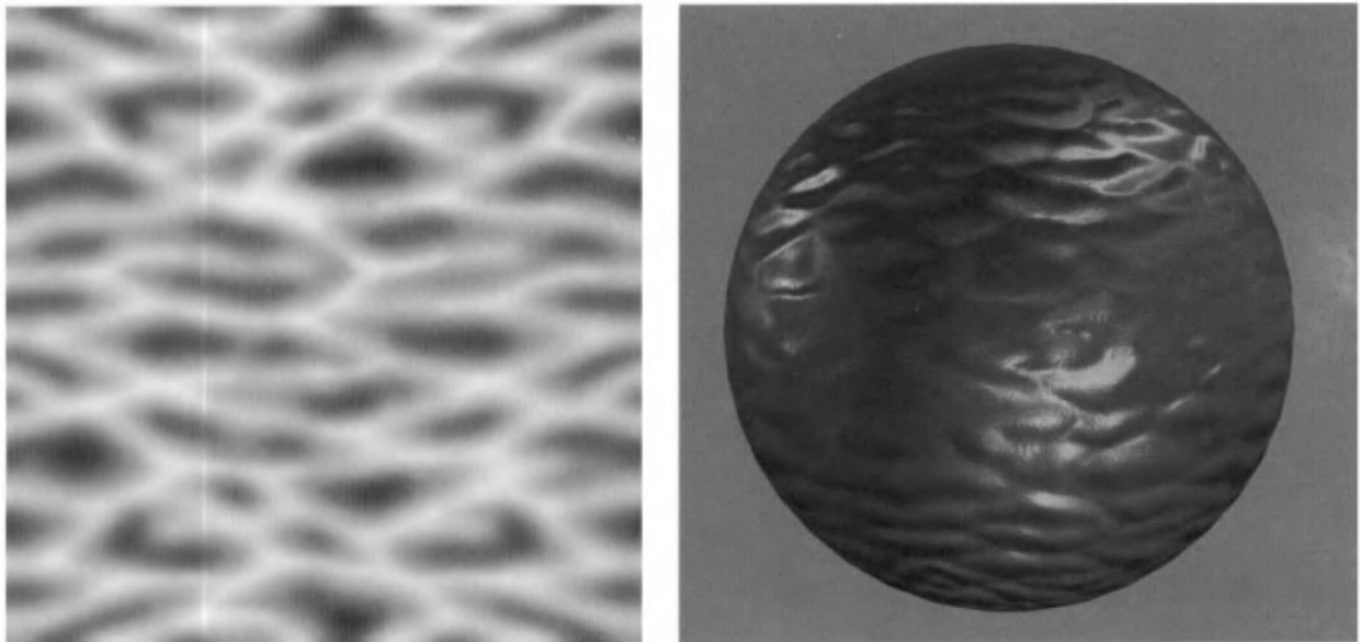
Figure 6.28. A wavy heightfield bump image and its use on a sphere, rendered with per-pixel illumination.
