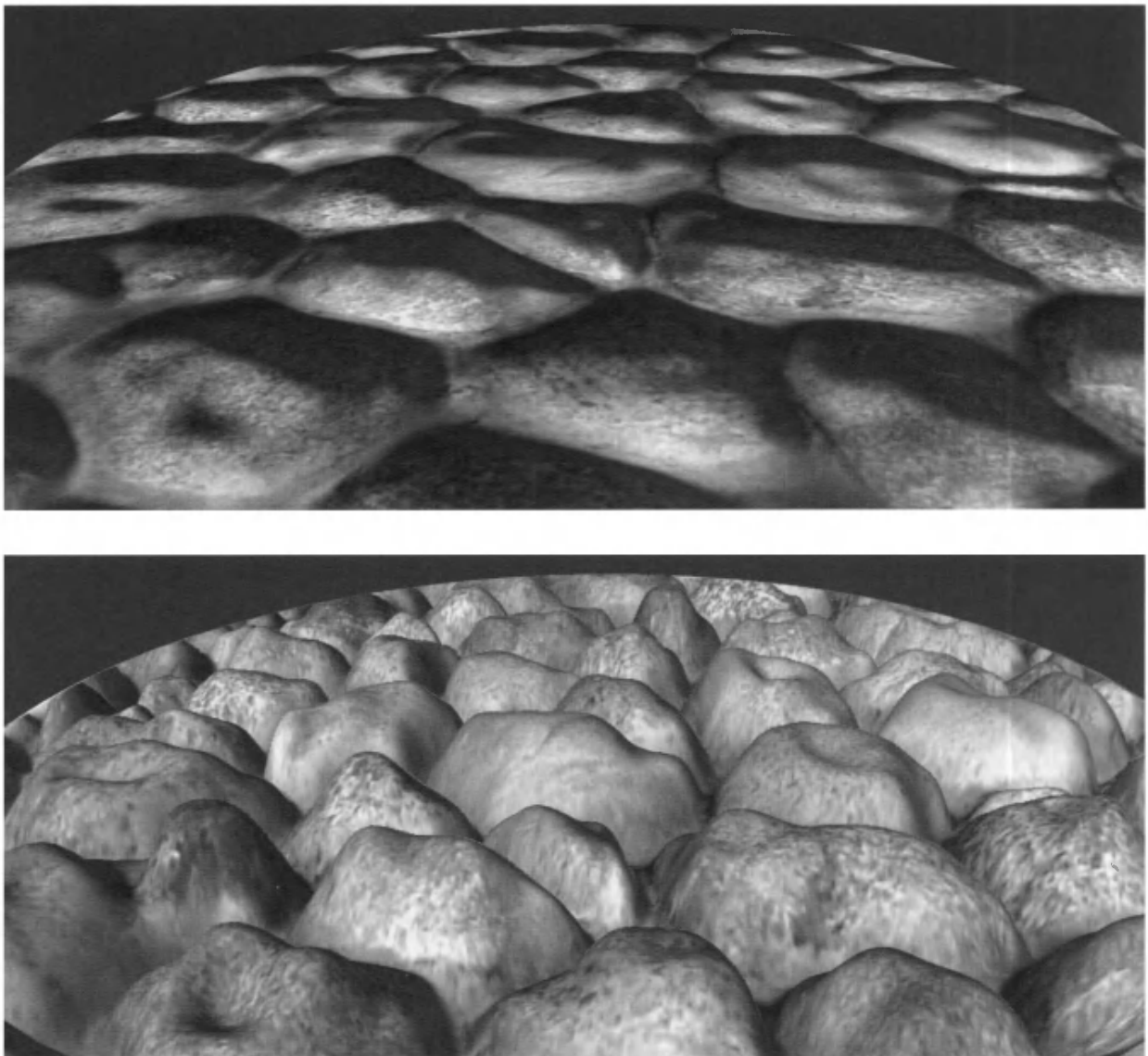
Figure 6.35. Normal mapping and relief mapping. No self-occlusion occurs with normal mapping. Relief mapping has problems with silhouettes for repeating textures, as the polygon is more of a view into the heightfield than a true boundary definition. (Images courtesy of NVIDIA Corporation.)
