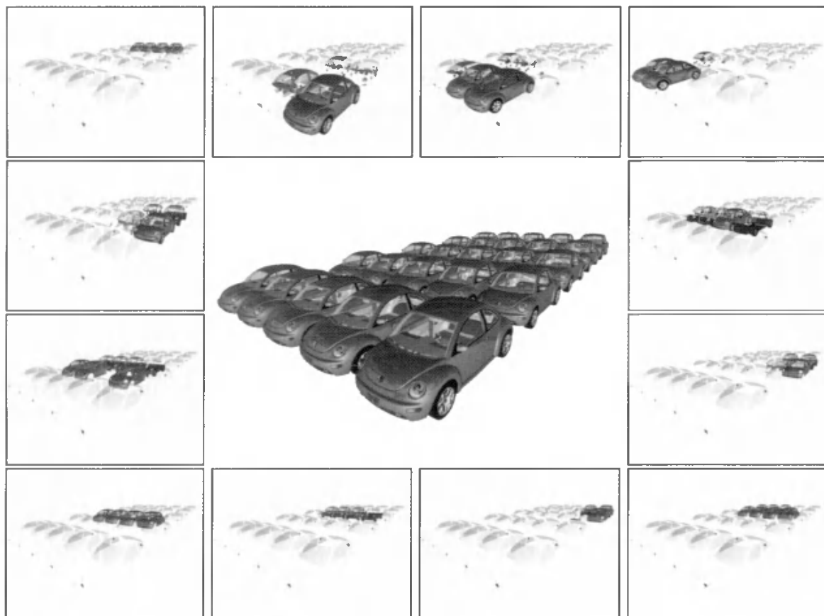
Figure 18.11. In sort-last image, different objects in the scene are sent to different processors. Transparency is difficult to deal with when compositing separate rendered images, so transparent objects are usually sent to all nodes. ( Images courtesy of Marcus Roth and Dirk Reiners. )
