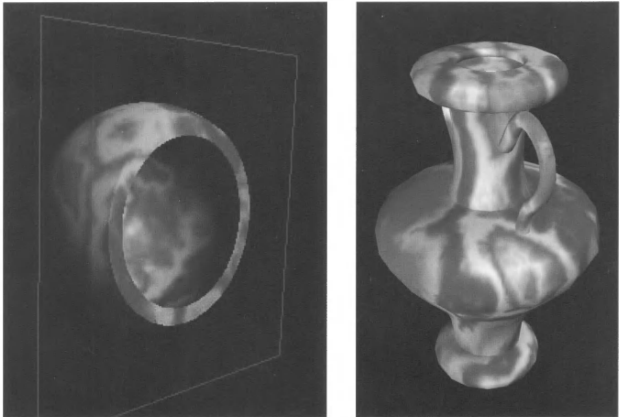
Figure 6.23. Two examples of real-time procedural texturing using a volume texture. The marble texture is continuous over the surface, with no mismatches at edges. The object on the left is formed by cutting a pair of spheres with a plane and using the stencil buffer to fill in the gap. ( Images courtesy of Evan Hart, ATI Technologies Inc. )
