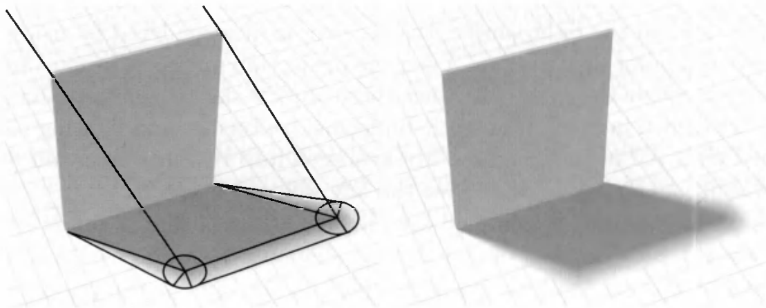
Figure 9.8. On the left, a visualization of Haines' method of soft shadowing on a plane. The object casts a hard shadow, and then gradient areas are drawn to simulate the penumbra. On the right is the result.
