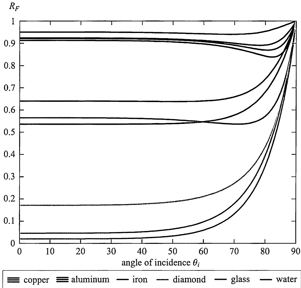
Figure 7.19. Fresnel reflectance for external reflection from a variety of substances. Since copper and aluminum have significant variation in their reflectance over the visible spectrum, their reflectance is shown as three separate curves for R, G, and B. Copper’s R curve is highest, followed by G, and finally B (thus its reddish color). Aluminum’s B curve is highest, followed by G, and finally R. Aluminum has a faint bluish tint that is most noticeable at an incidence angle of about 80^\circ .
