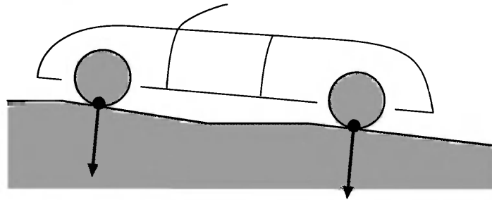
Figure 17.2. Instead of computing the collision between the entire car and the environment (the road), we place a ray at each wheel. These rays are then tested for intersection against the environment.
