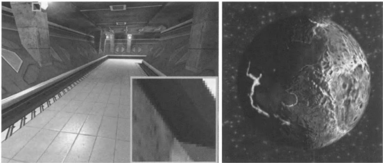
Figure 18.21. Two images rendered using the Mali 200 architecture for mobile devices, using the OpenGL ES 2.0 API. Rotated-grid supersampling (with four samples per pixel) is used to increase the image quality, and the antialiasing effect can be seen in the zoomed inset in the left image. The planet was rendered using pixel shader programs implementing a variety of techniques, including parallax mapping, environment mapping, and a full lighting equation. ( Images courtesy of ARM. )
