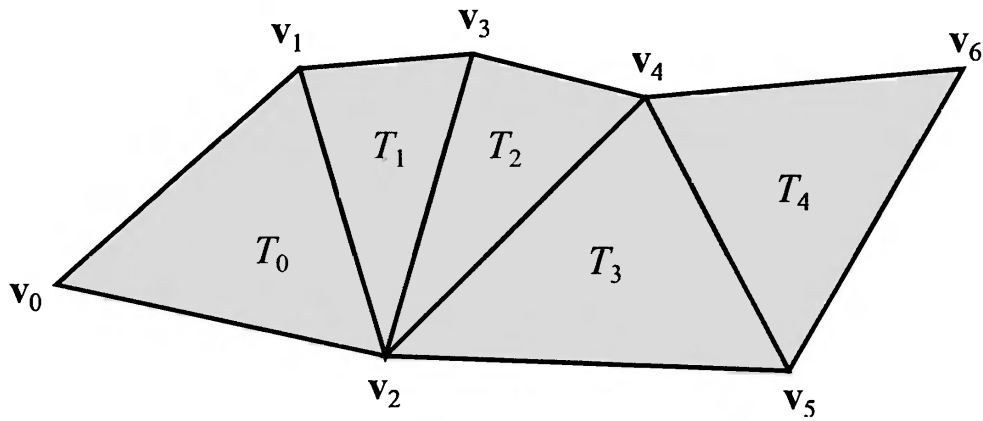
Figure 12.14. We would have to send (v_0, v_1, v_2, v_3, v_2, v_4, v_5, v_6) to the graphics pipeline to use these triangles as a strip. As can be seen, a swap has been implemented by including v_2 twice in the list.
