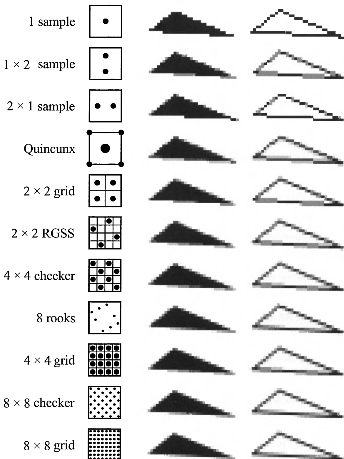
Figure 5.29. A comparison of some pixel sampling schemes. The 2 \times 2 rotated grid captures more gray levels for the nearly horizontal edge than a straight 2 \times 2 grid. Similarly, the 8 rooks pattern captures more gray levels for such lines than a 4 \times 4 grid, despite using fewer samples.
