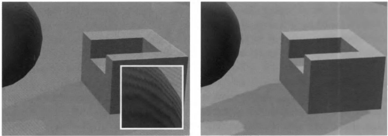
Figure 9.16. Shadow mapping problems. On the left there is no bias, so the surface erroneously shadows itself, in this case producing a Moiré pattern. The inset shows a zoom of part of the sphere’s surface. On the right, the bias is set too high, so the shadow creeps out from under the block object, giving the illusion that the block hovers above the surface. The shadow map resolution is also too low, so the texels of the map appear along the shadow edges, giving it a blocky appearance.
