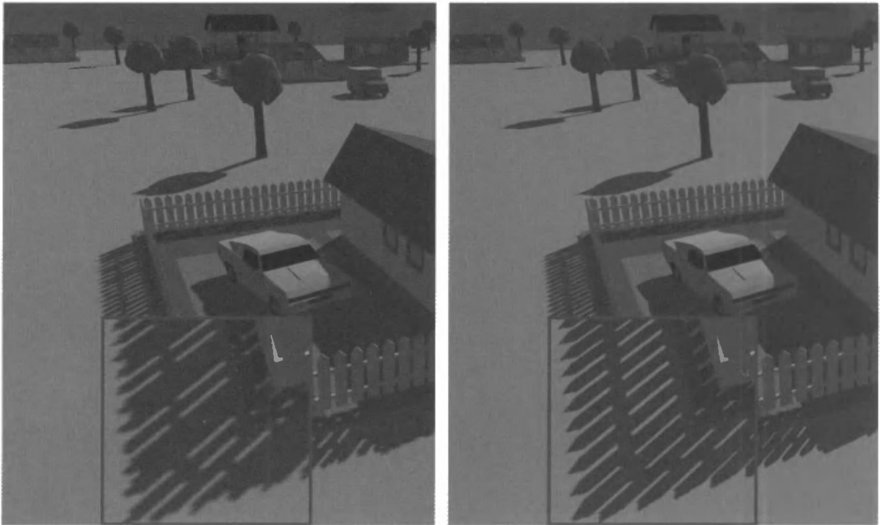
Figure 9.26. On the left, the scene's wide viewable area causes a single shadow map at a 2048 \times 2048 resolution to exhibit perspective aliasing. On the right, four 1024 \times 1024 shadow maps placed along the view axis improve quality considerably [1405]. A zoom of the front corner of the fence is shown in the inset red boxes. (Images courtesy of Fan Zhang, The Chinese University of Hong Kong.)
