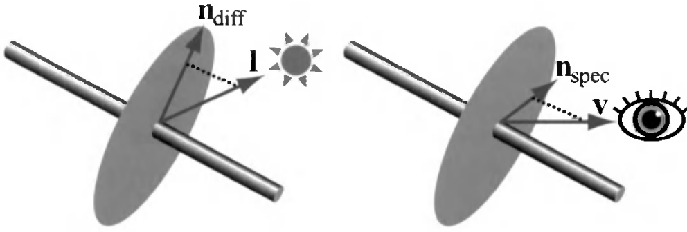
Figure 7.39. Shading normals used for the Kajiya-Kay model. A thin fiber is modeled as a cylinder that has an infinite number of surface normals (shown by the light blue circular plane) at each shaded point. On the left, the light vector \mathbf{l} is projected onto the normal plane, resulting in the vector \mathbf{n}_{\text{diff}} . This shading normal is used for computing the light projection cosine factor \overline{\cos} \theta'_i . On the right, the view vector \mathbf{v} is projected onto the normal plane, resulting in the vector \mathbf{n}_{\text{spec}} . This shading normal is used for computing the reflection vector \mathbf{r} used in the specular BRDF term.
