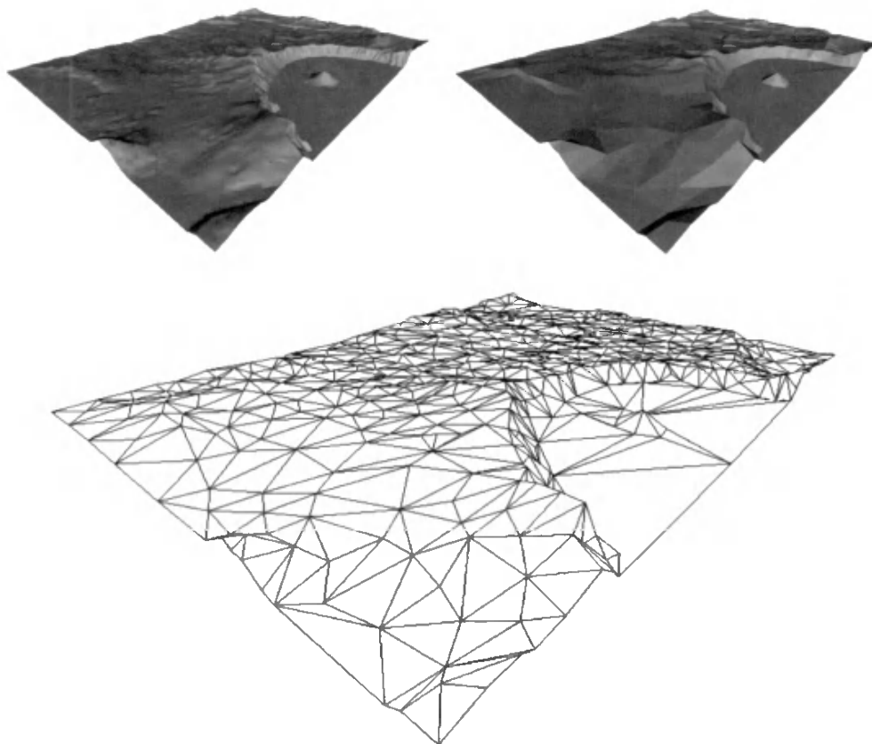
Figure 12.20. On the left is a heightfield of Crater Lake rendered with 200,000 triangles. The right figure shows this model simplified down to 1000 triangles. The underlying simplified mesh is shown below. (Images courtesy of Michael Garland.)
