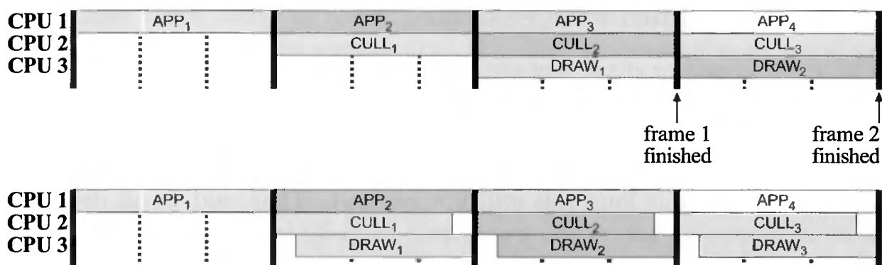
Figure 15.8. At the top, a three-stage pipeline is shown. In comparison to the configurations in Figure 15.7, this configuration has more time for each pipeline stage. The bottom illustration shows a way to reduce the latency: The CULL and the DRAW are overlapped with FIFO buffering in between.
