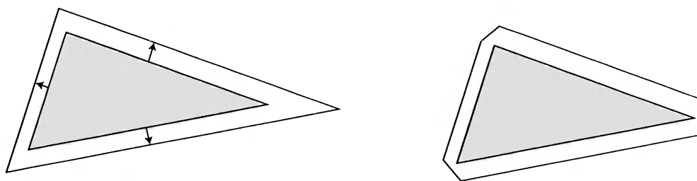
Figure 11.7. Triangle fattening. On the left, a backface triangle is expanded along its plane. Each edge moves a different amount in world space to make the resulting edge the same thickness in screen space. For thin triangles, this technique falls apart, as one corner becomes elongated. On the right, the triangle edges are expanded and joined to form mitered corners to avoid this problem.
