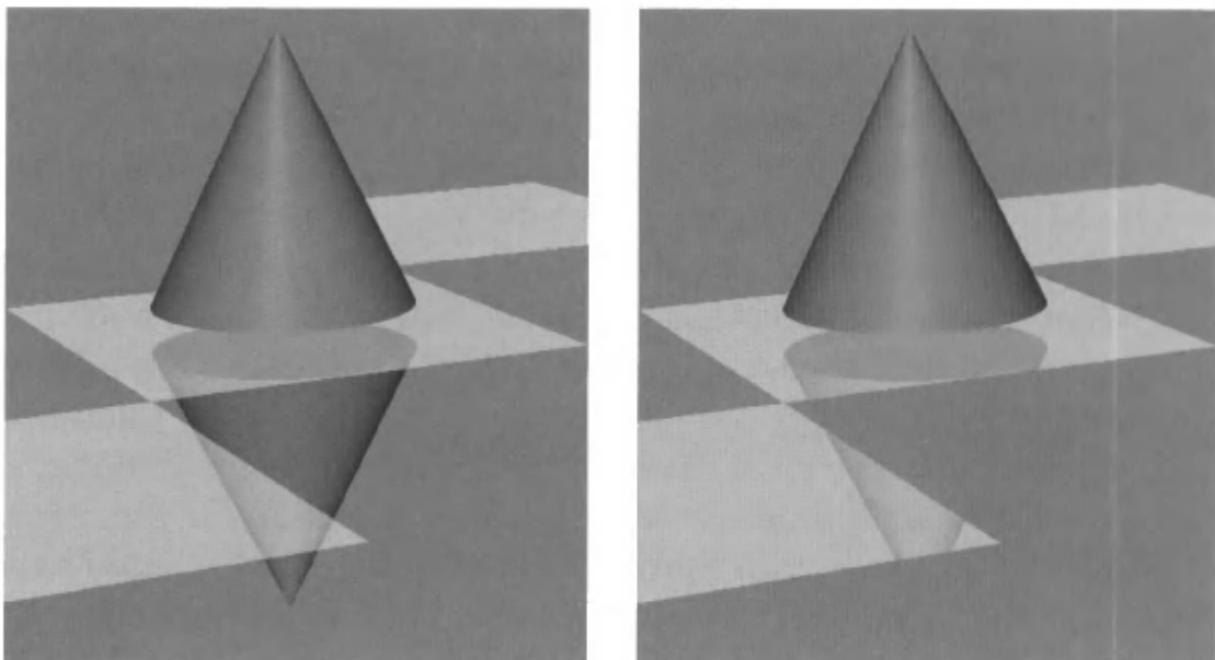
Figure 9.43. The left image shows an incorrectly rendered reflection against three mirrored squares. The right image was rendered with the use of the stencil buffer to mask out the part where there is visible reflector geometry, which yields a correct reflection.
