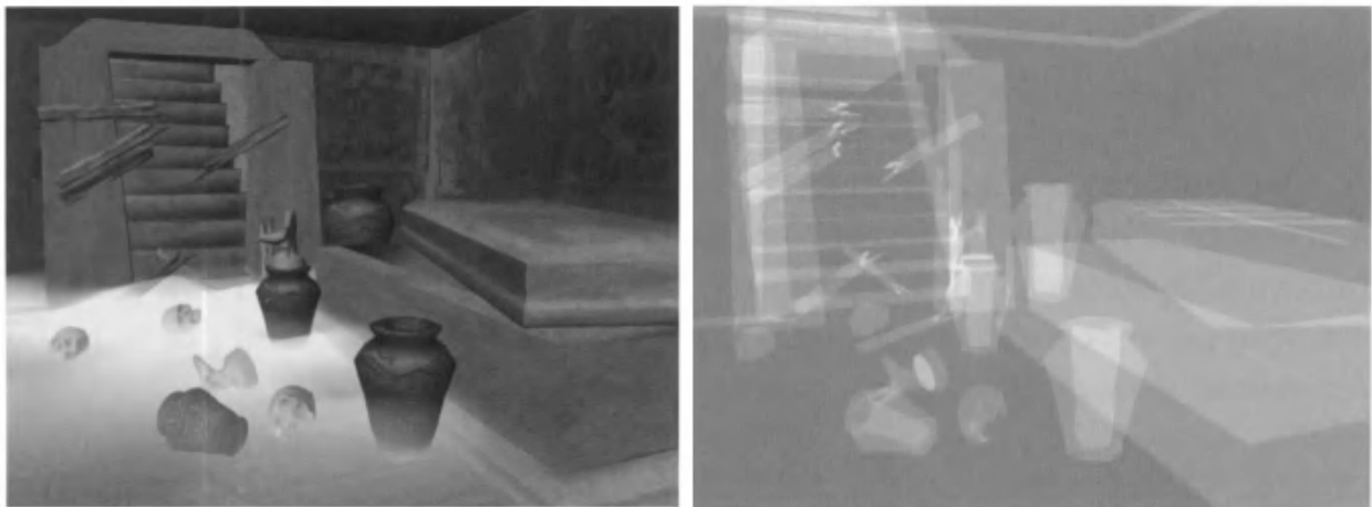
Figure 15.5. The depth complexity of the scene on the left is shown on the right. ( Images created using NVPerfHUD from NVIDIA Corporation. )
