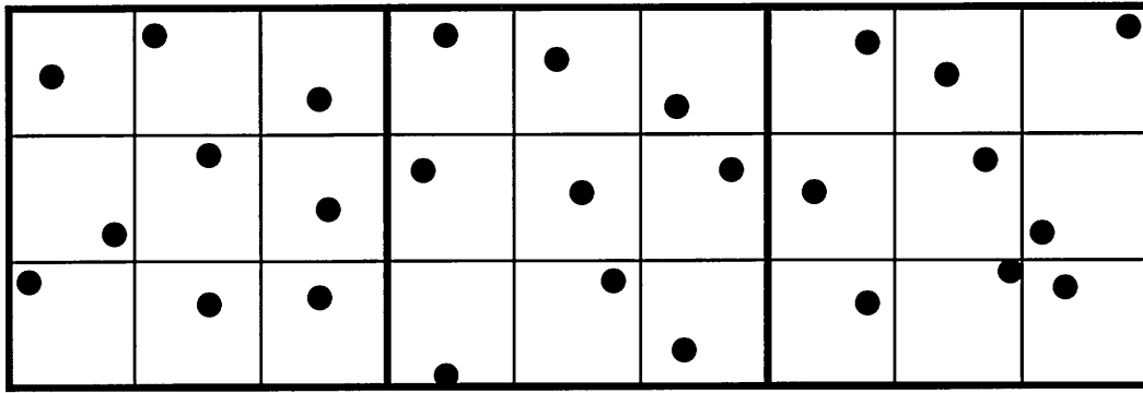
Figure 5.32. A typical jitter pattern for three pixels, each divided into a 3 \times 3 set of subcells. One sample appears in each subcell, in a random location.
