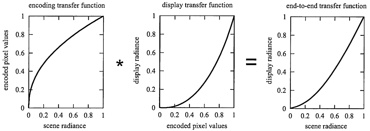
Figure 5.38. On the left is the function relating normalized scene radiance to encoded pixel values. In the middle is the function relating encoded pixel values to normalized display radiance. The concatenation of the two functions gives the end-to-end transfer function of the imaging system, shown to the right.
