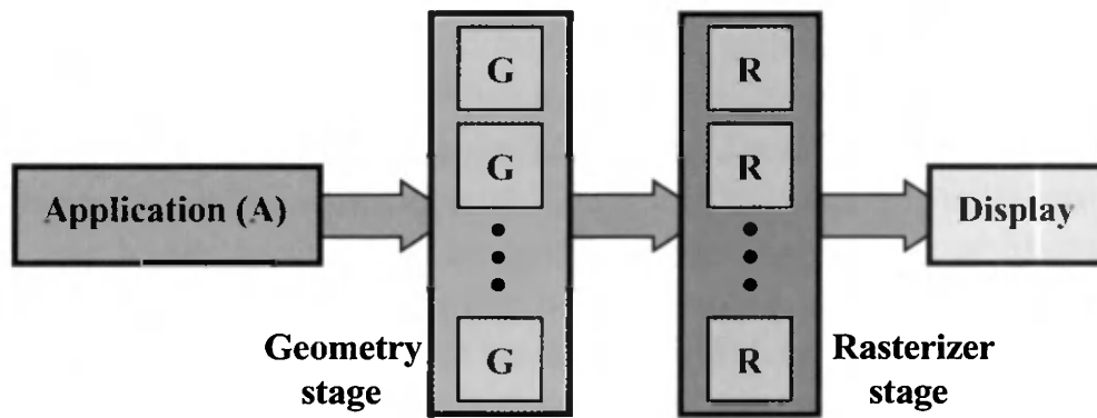
Figure 18.8. The general architecture for a high-performance, parallel computer graphics architecture. Each geometry unit (G) processes (i.e., transforms, projects, etc.) a portion of the geometry to be rendered, and each rasterizer unit (R) takes care of a portion of the pixel calculations.
