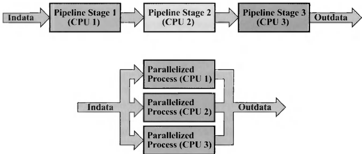
Figure 15.6. Two different ways of utilizing multiple processors. At the top we show how three processors (CPUs) are used in a multiprocessor pipeline , and at the bottom we show parallel execution on three CPUs. One of the differences between these two implementations is that lower latency can be achieved if the configuration at the bottom is used. On the other hand, it may be easier to use a multiprocessor pipeline. The ideal speedup for both of these configurations is linear, i.e., using n CPUs would give a speedup of n times.
