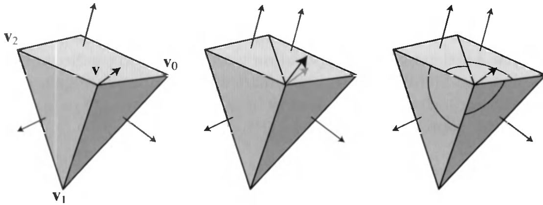
Figure 12.11. On the left, the surface normals of a rectangle and two triangles are averaged to give a vertex normal. In the middle, the square has been triangulated. This results in the average normal shifting, since each polygon's normal is weighted equally. On the right, Thürmer and Wüthrich's method weights each normal's contribution by its angle between the pair of edges forming it, so triangulation does not shift the normal.
