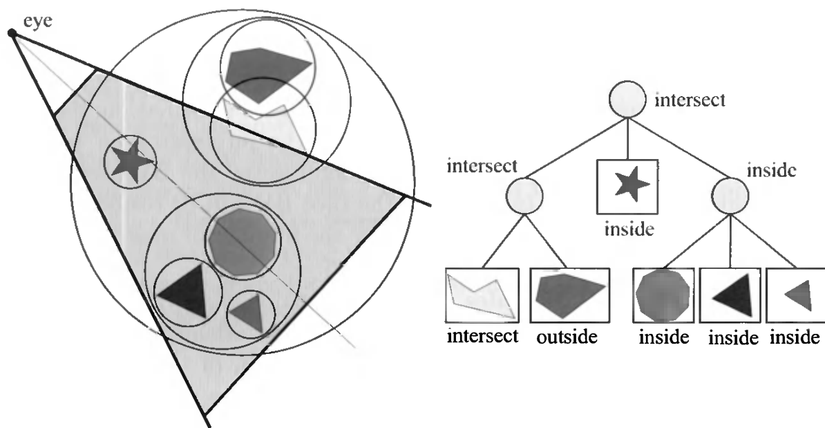
Figure 14.12. A set of geometry and its bounding volumes (spheres) are shown on the left. This scene is rendered with view frustum culling from the point of the eye. The BVH is shown on the right. The BV of the root intersects the frustum, and the traversal continues with testing its children's BVs. The BV of the left subtree intersects, and one of that subtree's children intersects (and thus is rendered), and the BV of the other child is outside and therefore is not sent through the pipeline. The BV of the middle subtree of the root is totally inside and is rendered immediately. The BV of the right subtree of the root is also fully inside, and the entire subtree can therefore be rendered without further tests.
