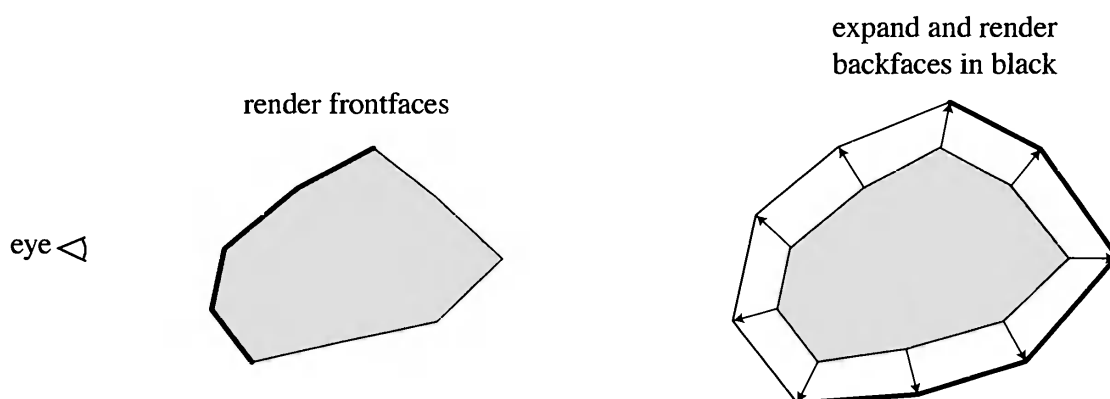
Figure 11.9. The triangle shell technique creates a second surface by shifting the surface along its vertex normals.
