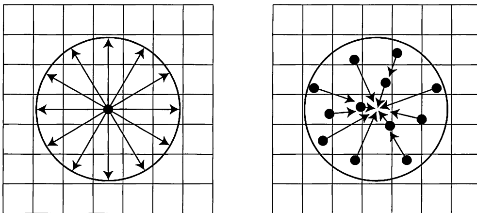
Figure 10.30. A scatter operation takes a pixel's value and spreads it to the neighboring area, for example by rendering a circular sprite. In a gather, the neighboring values are sampled and used to affect a pixel. The GPU's pixel shader is optimized to perform gather operations via texture sampling.
