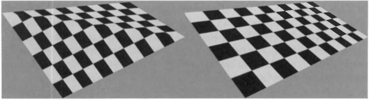
Figure 18.6. A textured quadrilateral consists of two triangles. To the left, linear interpolation is used over each triangle, and to the right, perspective-correct interpolation is used. Notice how linear interpolation ruins the three-dimensional effect.
