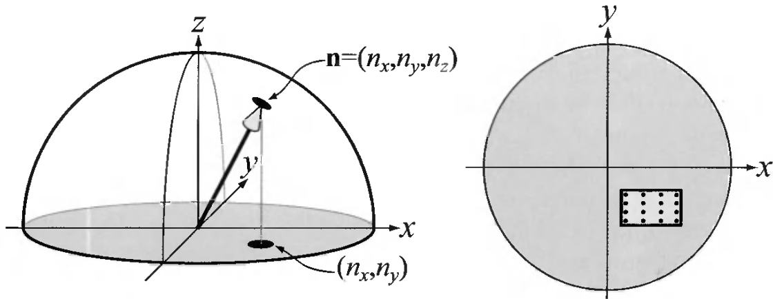
Figure 6.22. Left: the unit normal on a sphere only needs to encode the x - and y -components. Right: for BC4/3Dc, a box in the xy -plane encloses the normals, and 8 \times 8 normals inside this box can be used per 4 \times 4 block of normals (for clarity, only 4 \times 4 normals are shown here).
