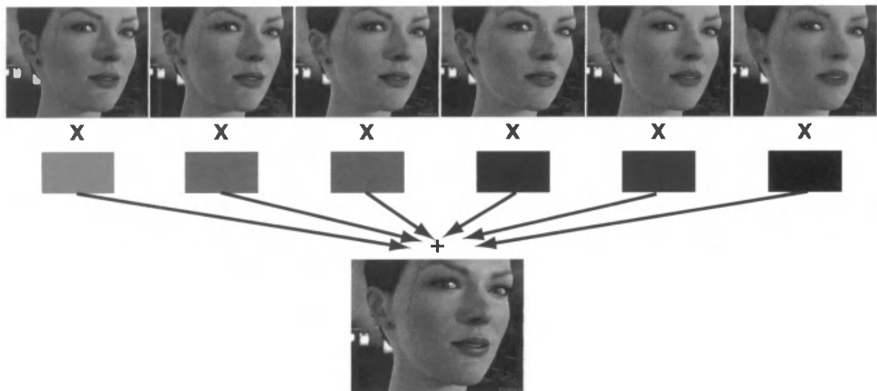
Figure 9.55. Texture space multilayer diffusion. Six different blurs are combined using RGB weights. The final image is the result of this linear combination, plus a specular term. ( Images courtesy NVIDIA Corporation. )
