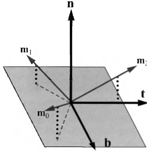
Figure 9.64. Half-Life 2 lighting basis. The three basis vectors have elevation angles of about 26^\circ above the tangent plane, and their projections into that plane are spaced equally (at 120^\circ intervals) around the normal. They are unit length, and each one is perpendicular to the other two.
