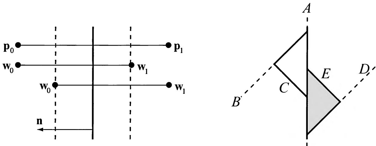
Figure 17.7. To the left, the line segment defined by p_0 and p_1 is clipped against a plane defined by a normal n . The dynamic adjustments of this plane is shown as dashed lines. The functions clipLineInside and clipLineOutside returns the line segments defined by w_0 and w_1 . Note that all three lines should have the same y -coordinates, but they are shown like this for clarity. To the right, an example is shown that explains why the lines should be clipped as shown to the left. The node A in the BSP tree belongs to both the triangle on the left and on the right. Therefore, it is necessary to move its plane in both directions.
