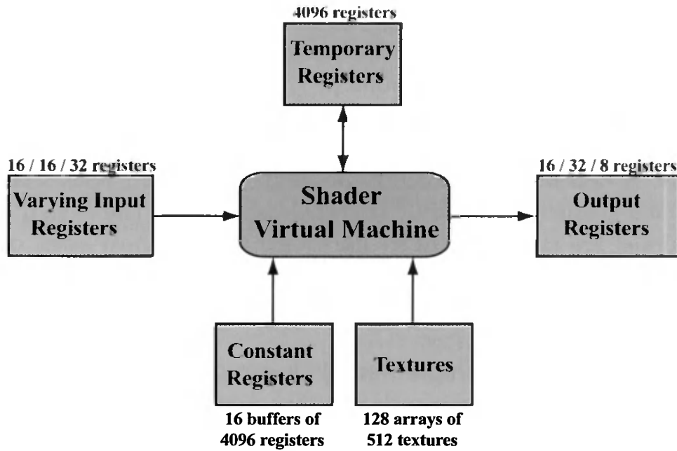
Figure 3.2. Common-shader core virtual machine architecture and register layout, under DirectX 10. The maximum available number is indicated next to each resource. Three numbers separated by slashes refer to the limits for vertex, geometry, and pixel shaders (from left to right).
