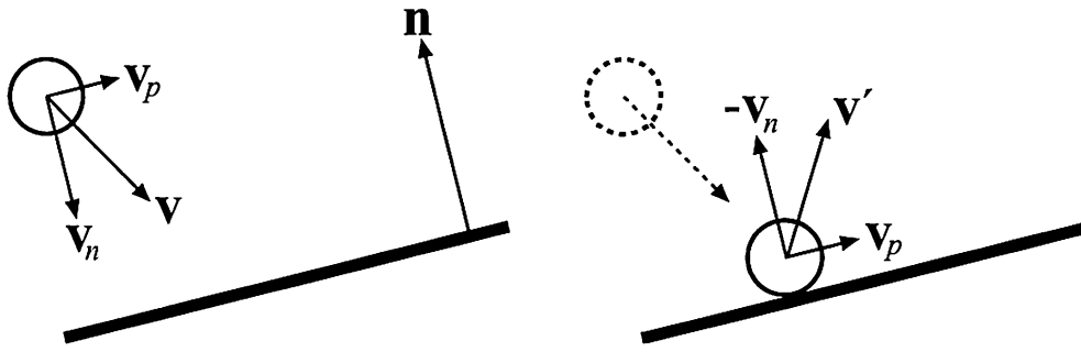
Figure 17.18. Collision response for a sphere approaching a plane. To the left the velocity vector \mathbf{v} is divided into two components, \mathbf{v}_n , and \mathbf{v}_p . To the right, perfectly elastic (bouncy) collision is shown, where the new velocity is \mathbf{v}' = \mathbf{v}_p - \mathbf{v}_n . For a less elastic collision, the length of -\mathbf{v}_n could be decreased.
