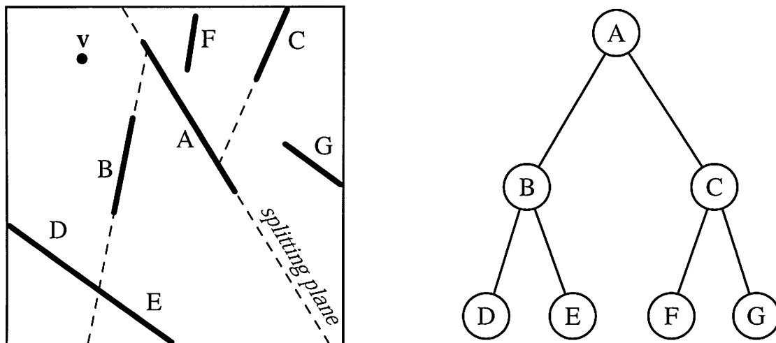
Figure 14.4. Polygon-aligned BSP tree. Polygons A through G are shown from above. Space is first split by polygon A, then each half-space is split separately by B and C. The splitting plane formed by polygon B intersects the polygon in the lower left corner, splitting it into separate polygons D and E. The BSP tree formed is shown on the right.
