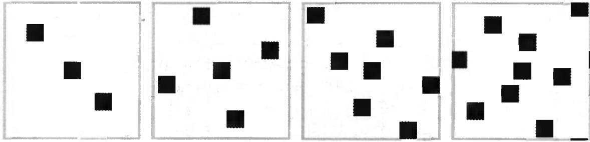
Figure 5.30. MSAA sampling patterns for ATI and NVIDIA graphics accelerators. The green square is the location of the shading sample, and the red squares are the positional samples computed and saved. From left to right: 2x, 4x, 6x (ATI), and 8x (NVIDIA) sampling. ( Generated by the D3D FSAA Viewer. )
