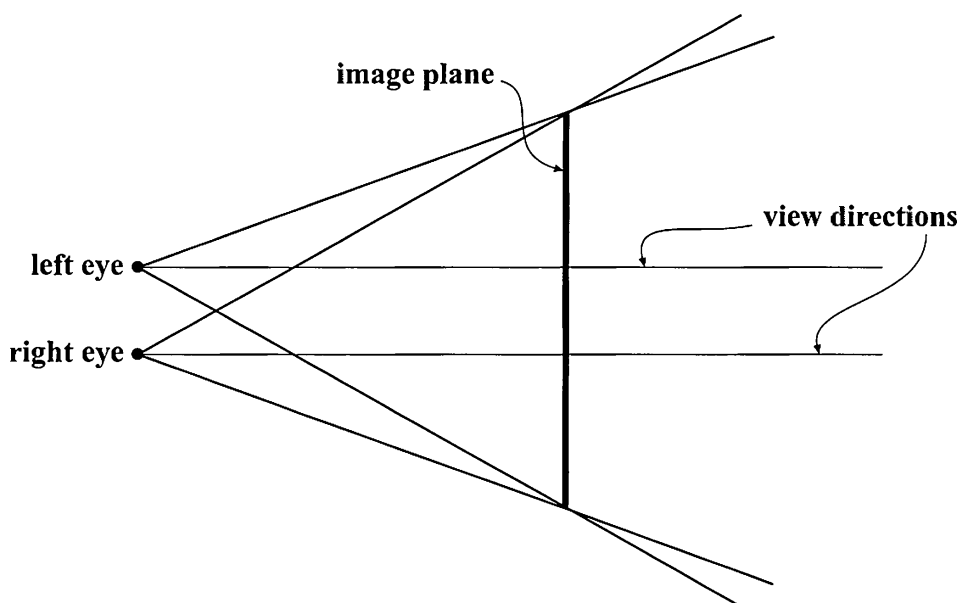
Figure 18.5. Stereo rendering. Note that the image plane is shared between the two frustums, and that the frustums are asymmetric. Such rendering would be used on, for example, a stereo monitor. Shutter glasses could use separate image planes for each eye.
