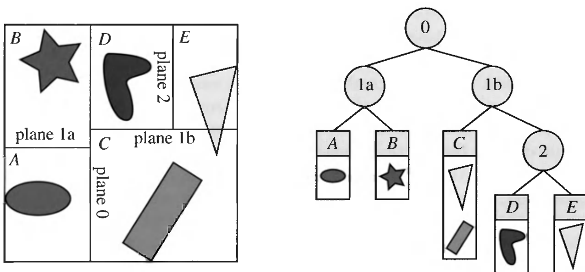
Figure 14.3. Axis-aligned BSP tree. In this example, the space partitions are allowed to be anywhere along the axis, not just at its midpoint. The spatial volumes formed are labeled A through E. The tree on the right shows the underlying BSP data structure. Each leaf node represents an area, with that area's contents shown beneath it. Note that the triangle is in the object list for two areas, C and E, because it overlaps both.
