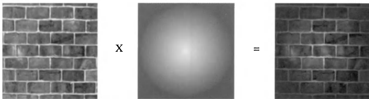
Figure 9.63. Irradiance map combined with a diffuse color, or albedo, map. The diffuse color map on the left is multiplied by the irradiance map in the middle to yield the result on the right. (Images courtesy of J.L. Mitchell, M. Tatro, and I. Bullard.)
