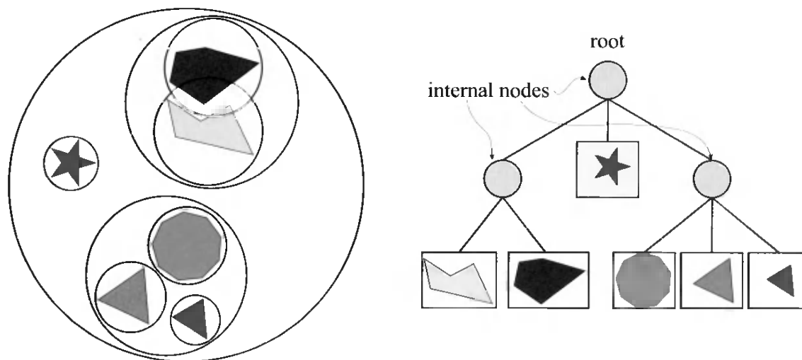
Figure 14.2. The left part shows a simple scene with six objects, each enclosed by a bounding sphere. The bounding spheres are then grouped together into larger bounding spheres, until all objects are enclosed by the largest sphere. The right part shows the bounding volume hierarchy (tree) that is used to represent the object hierarchy on the left. The BV of the root encloses all objects in the scene.
