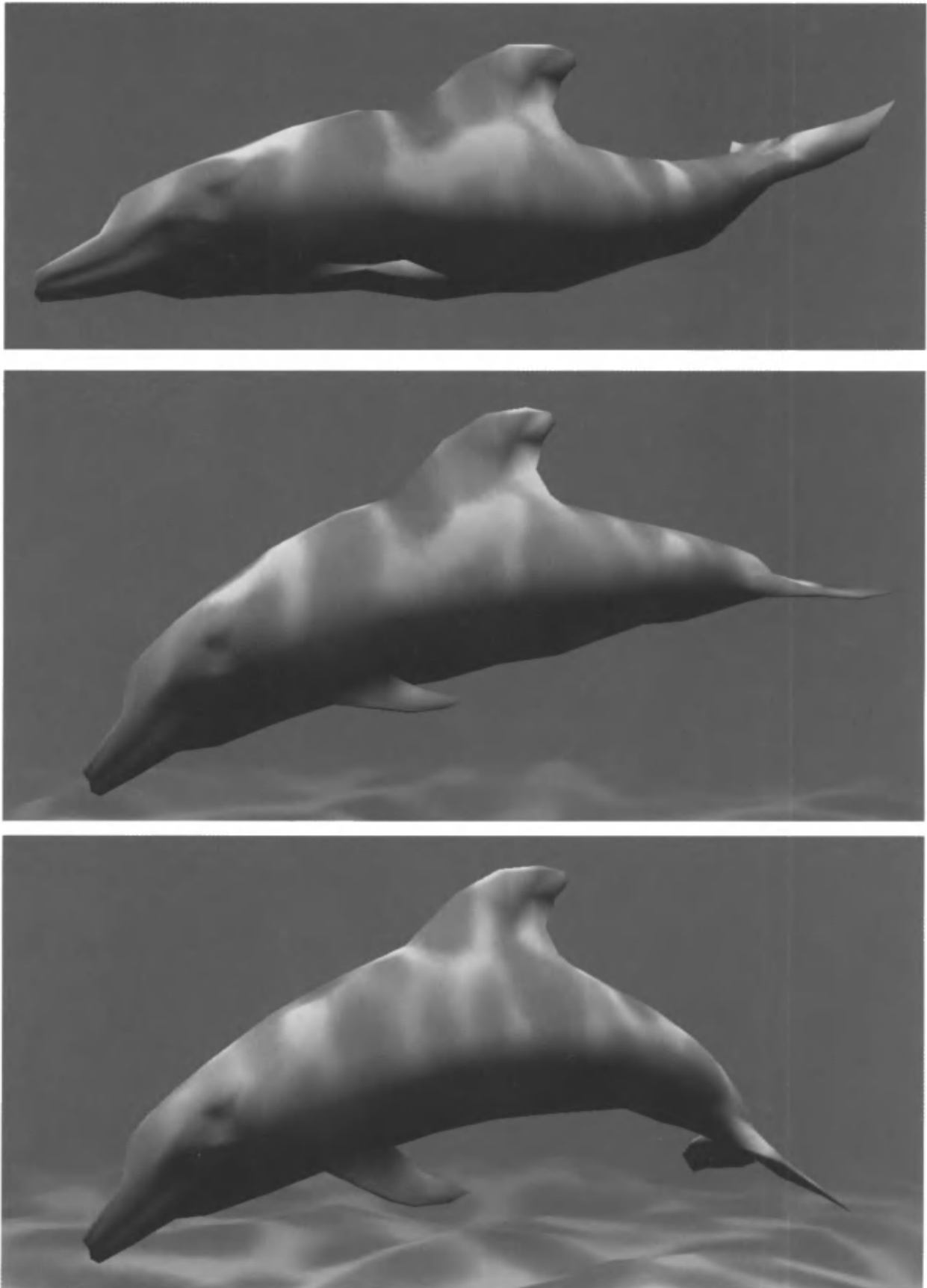
Figure 4.13. Vertex morphing. Two locations and normals are defined for every vertex. In each frame, the intermediate location and normal are linearly interpolated by the vertex shader. ( Images courtesy of NVIDIA Corporation. )
