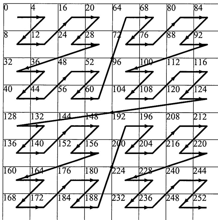
Figure 18.12. Texture swizzling increases coherency of texel memory accesses. Note that texel size here is four bytes, and that the texel address is shown in each texel's upper left corner.
