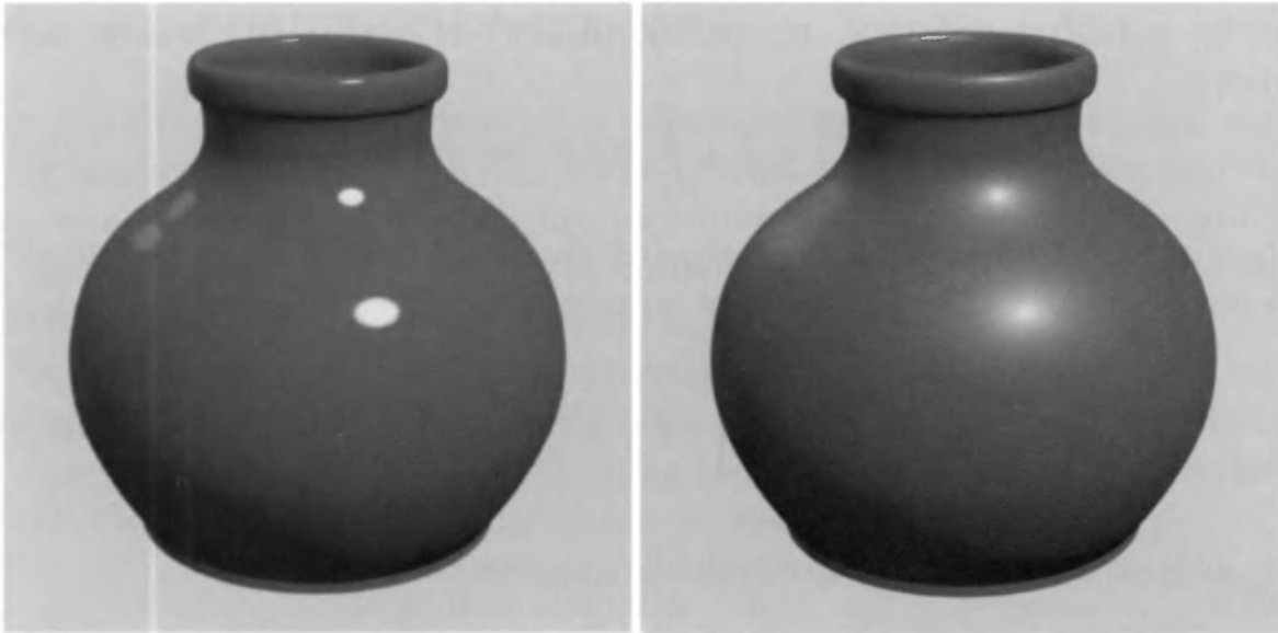
Figure 8.7. Highlights on smooth objects are sharp reflections of the light source shape. On the left, this appearance has been approximated by thresholding the highlight value of a Blinn-Phong shader. On the right, the same object rendered with an unmodified Blinn-Phong shader for comparison. ( Image courtesy of Larry Gritz. )
