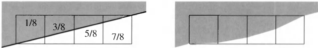
Figure 5.40. On the left, four pixels covered by the edge of a white polygon on a black (shown as gray) background, with true area coverage shown. If gamma correction is not performed, the darkening of midtones will cause the perception of the edge to be distorted, as seen on the right.
