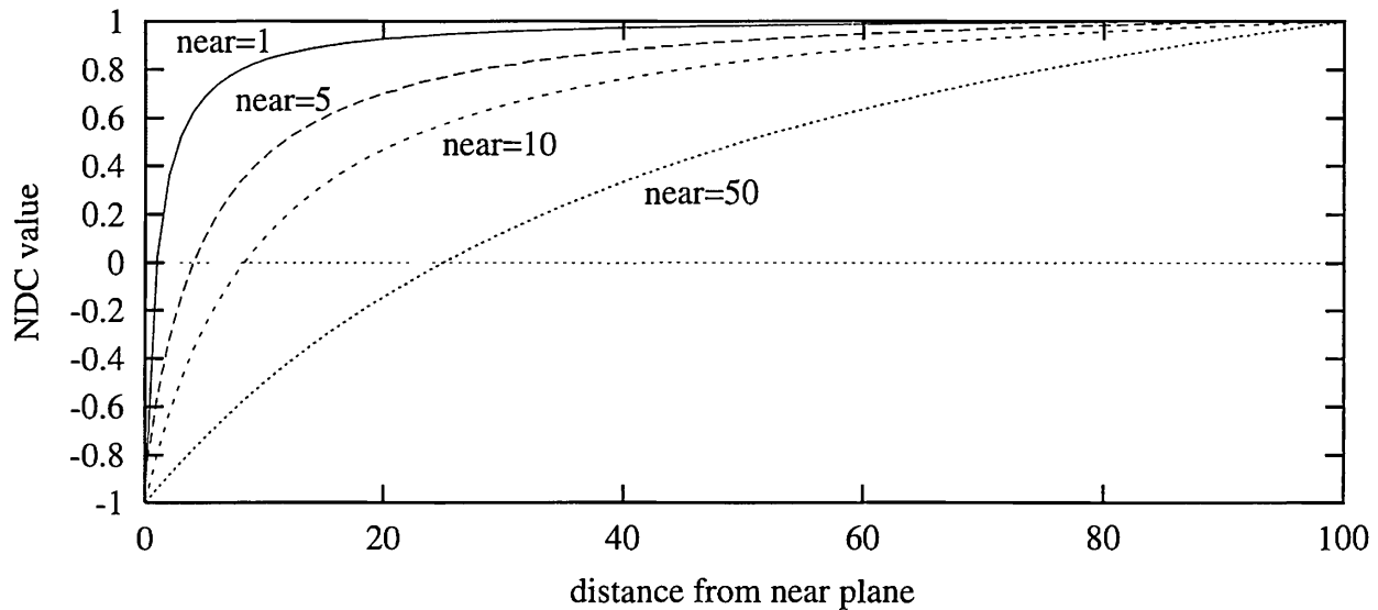
Figure 4.20. The effect of varying the distance of the near plane from the origin. The distance f' - n' is kept constant at 100. As the near plane becomes closer to the origin, points nearer the far plane use a smaller range of the normalized device coordinate depth space. This has the effect of making the Z-buffer less accurate at greater distances.
