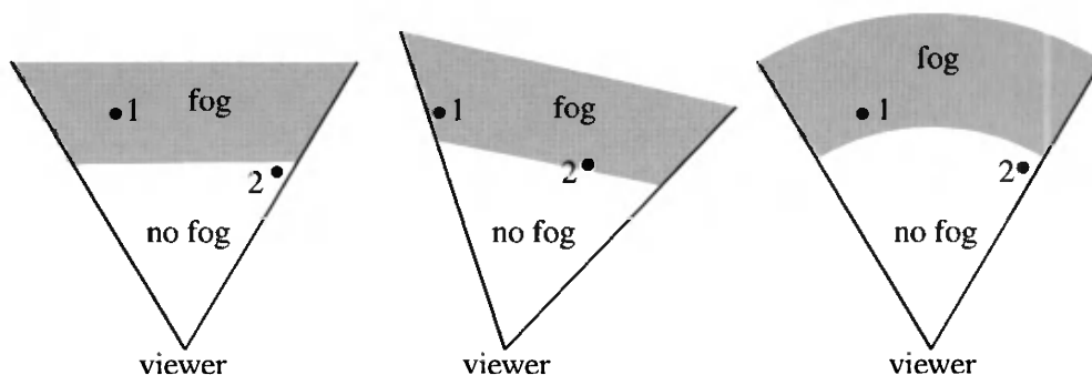
Figure 10.39. Use of z -depth versus radial fog. On the left is one view of two objects, using view-axis-based fog. In the middle, the view has simply been rotated, but in the rotation, the fog now encompasses object 2. On the right, we see the effect of radial fog, which will not vary when the viewer rotates.
