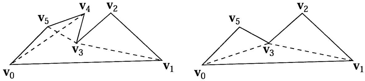
Figure 12.3. Ear clipping. A polygon with potential ears at v_2 , v_4 , and v_5 shown. On the right, the ear at v_4 is removed. The neighboring vertices v_3 and v_5 are reexamined to see if they now form ears; v_5 does.
