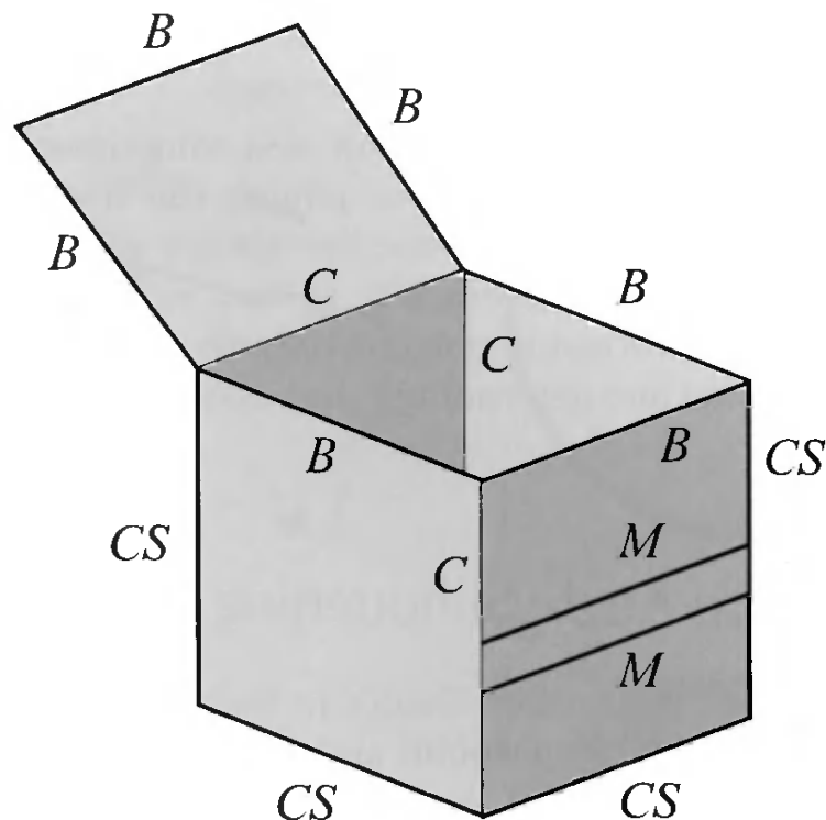
Figure 11.4. A box open on the top, with a stripe on the front. The boundary ( B ), crease ( C ), material ( M ), and silhouette ( S ) edges are shown.
