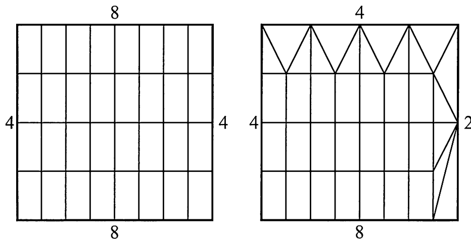
Figure 13.53. Left: normal tessellation—one factor is used for the rows, and another for the columns. Right: independent tessellation factors on all four edges. ( Illustration after Moreton [904]. )
