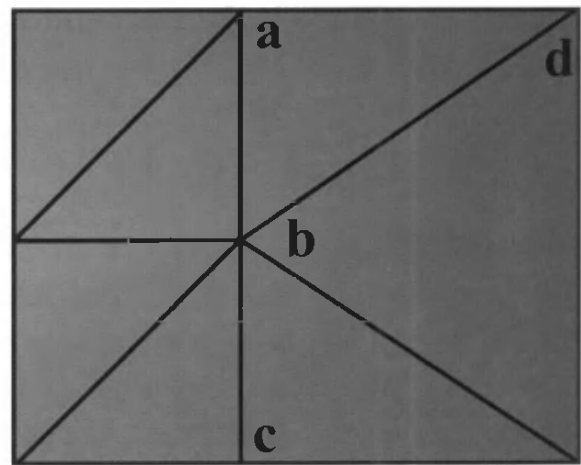
Figure 12.8. In the top row, the underlying mesh of a surface shows a shading discontinuity. Vertex b is a T-vertex, as it belongs to the polygons to the left of it, but is not a part of the triangle acd . One solution is to add this T-vertex to this triangle and create triangles abd and bcd (not shown). Long and thin triangles are more likely to cause other shading problems, so retriangulating is often a better solution, shown in the bottom row.
