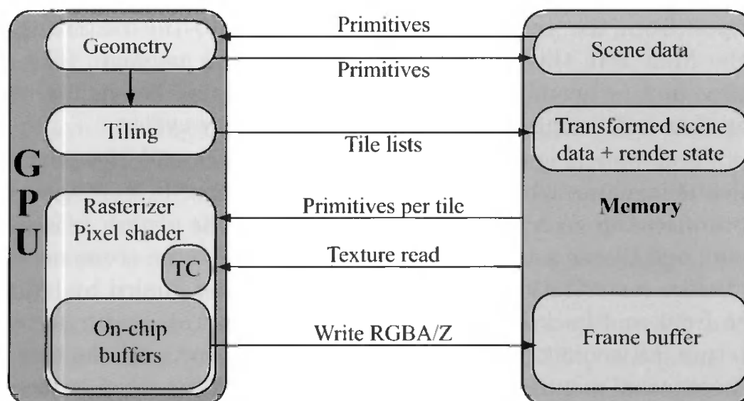
Figure 18.20. Overview of the Mali 200 tiling architecture, targeted toward mobile devices. The TC block is the texture cache.
