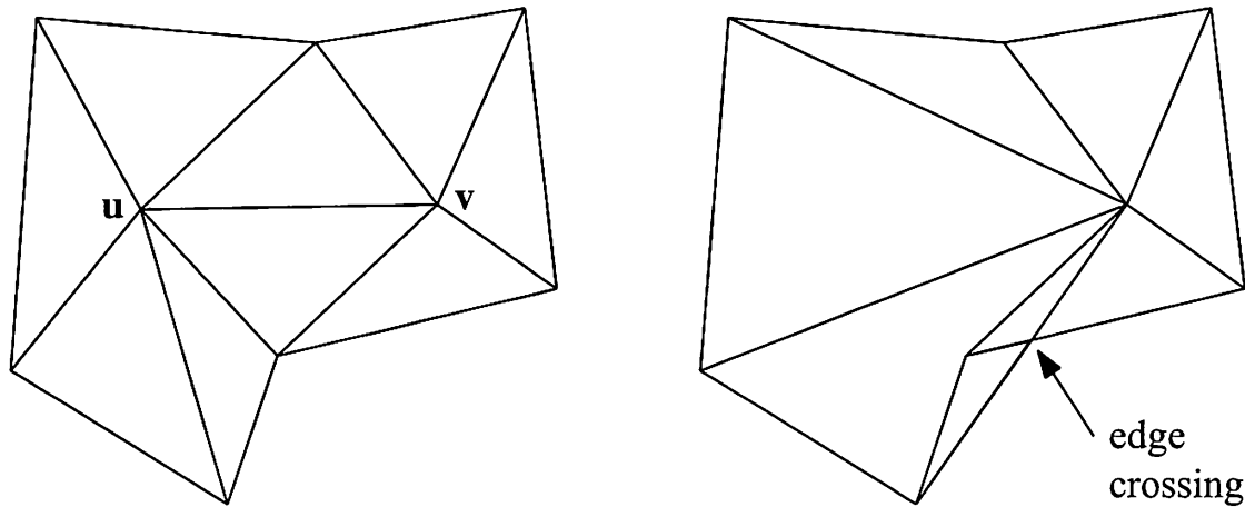
Figure 12.22. Example of a bad collapse. On the left is a mesh before collapsing vertex u into v . On the right is the mesh after the collapse, showing how edges now cross.
