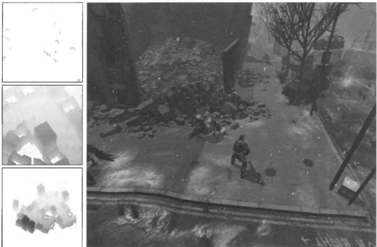
Figure 9.24. On the left, the three shadow maps are shown: animated objects, grid section, and whole level. On the right, a resulting image. (Images from “Hellgate: London” courtesy of Flagship Studios, Inc.)
