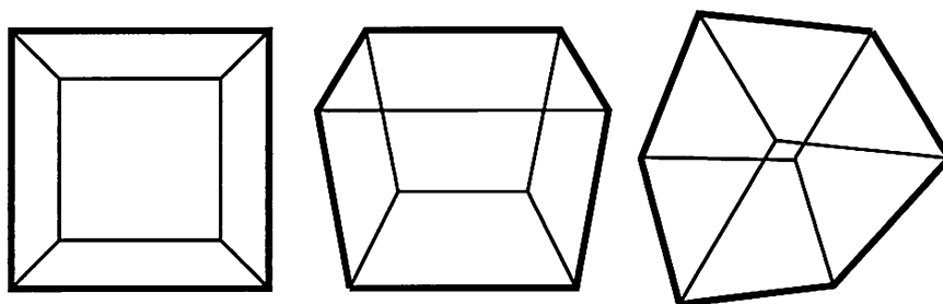
Figure 14.28. Three cases of projection of a cube, showing one, two, and three frontfaces. (Illustration after Schmalstieg and Tobler [1130].)
