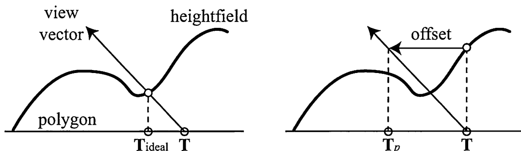
Figure 6.31. On the left is the goal: The actual position on the surface is found from where the view vector pierces the heightfield. Parallax mapping does a first-order approximation by taking the height at the location on the polygon and using it to find a new location \mathbf{p}_{\text{adj}} . (After Welsh [1338].)
