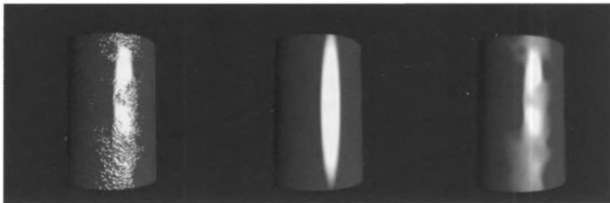
Figure 7.46. The cylinder from Figure 7.44. On the left, rendered with the original normal map. In the center, rendered with a much lower-resolution normal map containing averaged and renormalized normals (as shown in the bottom left of Figure 7.45). On the right, the cylinder is rendered with textures at the same low resolution, but containing normal and gloss values fitted to the ideal NDF, as shown in the bottom right of Figure 7.45. The image on the right is a significantly better representation of the original appearance. It will also be less prone to aliasing when rendered at low resolutions. (Image courtesy of Patrick Conran, ILM.)
