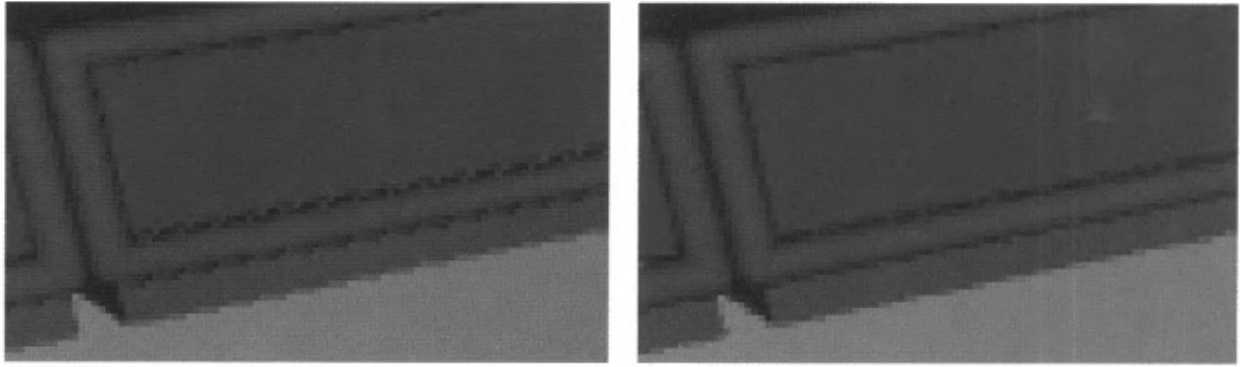
Figure 5.33. On the left, antialiasing with the accumulation buffer, with four samples per pixel. The repeating pattern gives noticeable problems. On the right, the sampling pattern is not the same at each pixel, but instead patterns are interleaved. (Images courtesy of Alexander Keller and Wolfgang Heidrich.)
