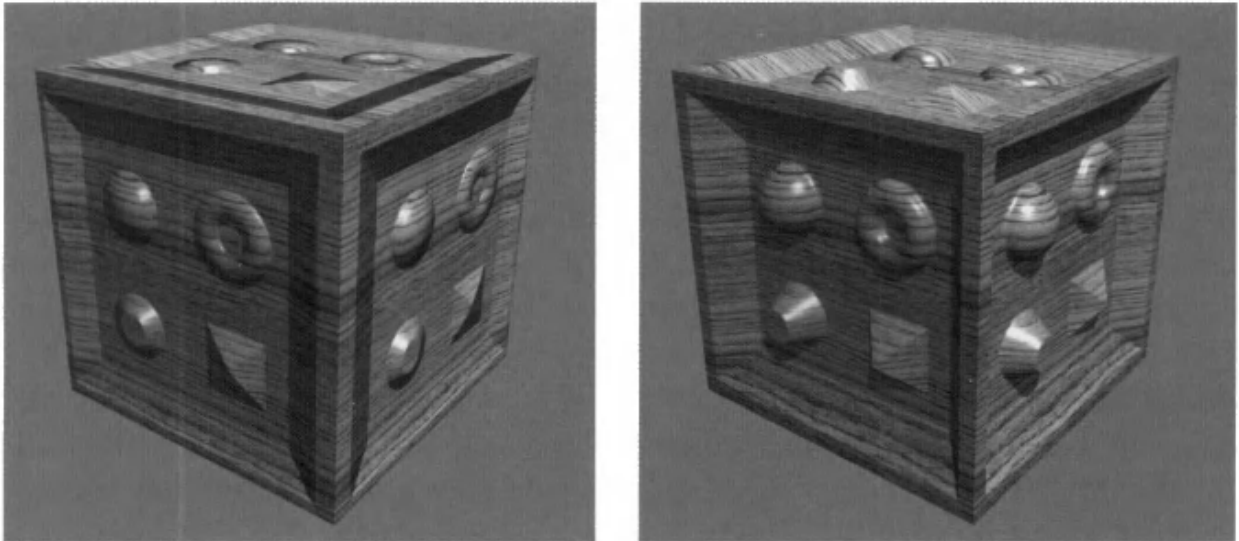
Figure 6.34. Parallax mapping compared to relief mapping. On the top of the cube there is flattening with parallax mapping. Relief mapping is also able to provide self-shadowing. ( Images courtesy of Manuel M. Oliveira and Fabio Policarpo. )
