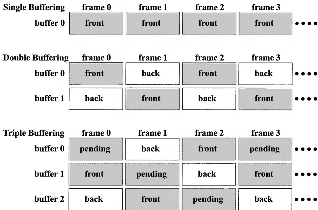
Figure 18.4. For single buffering, the front buffer is always shown. For double buffering, buffer 0 is first in front and buffer 1 is in the back. Then they swap from front-to-back and vice versa for each frame. Triple buffering works by having a pending buffer as well. Here, a buffer is first cleared, and rendering to it is begun (pending). Second, the system continues to use the buffer for rendering until the image has been completed (back). Finally, the buffer is shown (front).
