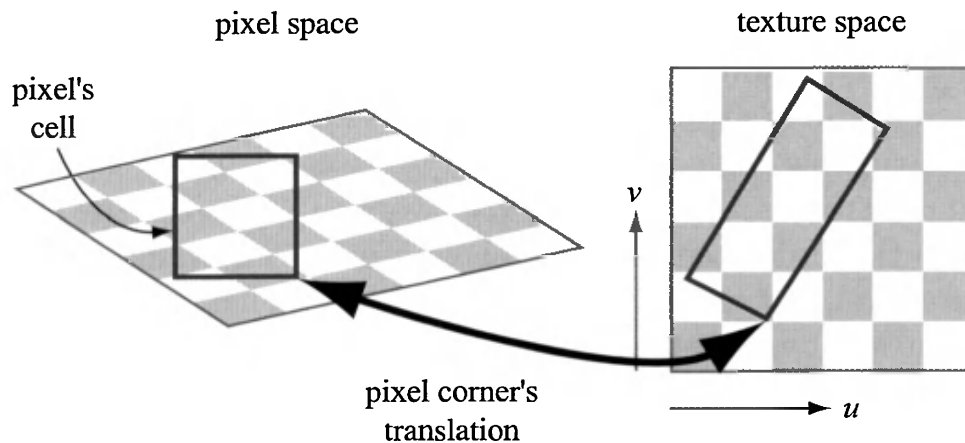
Figure 6.15. On the left is a square pixel cell and its view of a texture. On the right is the projection of the pixel cell onto the texture itself.
