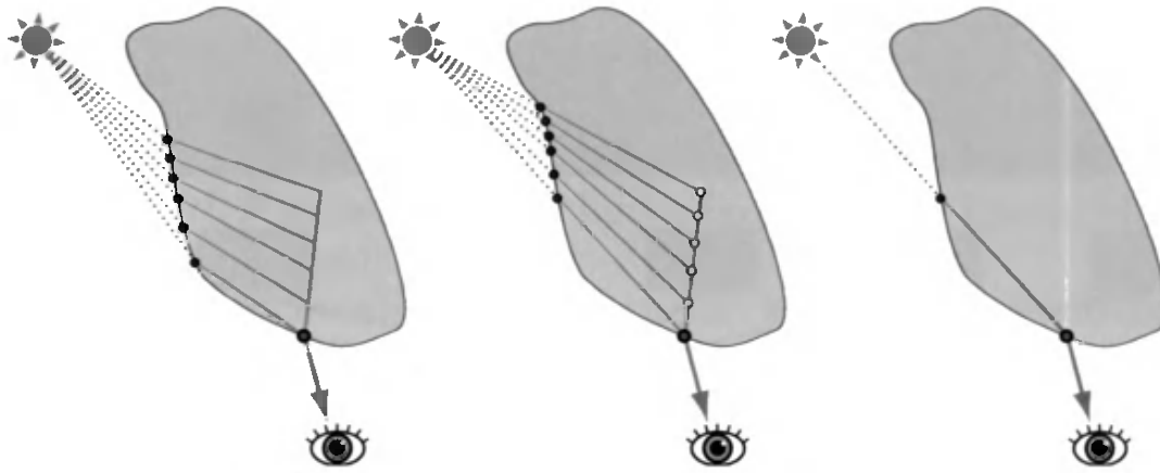
Figure 9.56. On the left, the ideal situation, in which light refracts when entering the object, then all scattering contributions that would properly refract upon leaving the object are computed. The middle shows a computationally simpler situation, in which the rays refract only on exit. The right shows a much simpler, and therefore faster, approximation, where only a single ray is considered.
