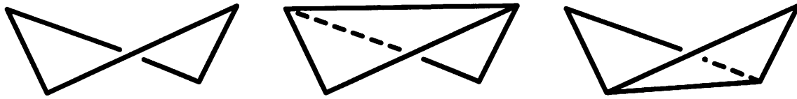
Figure 12.2. Warped quadrilateral viewed edge-on, forming an ill-defined bowtie or hourglass figure, along with the two possible triangulations.
