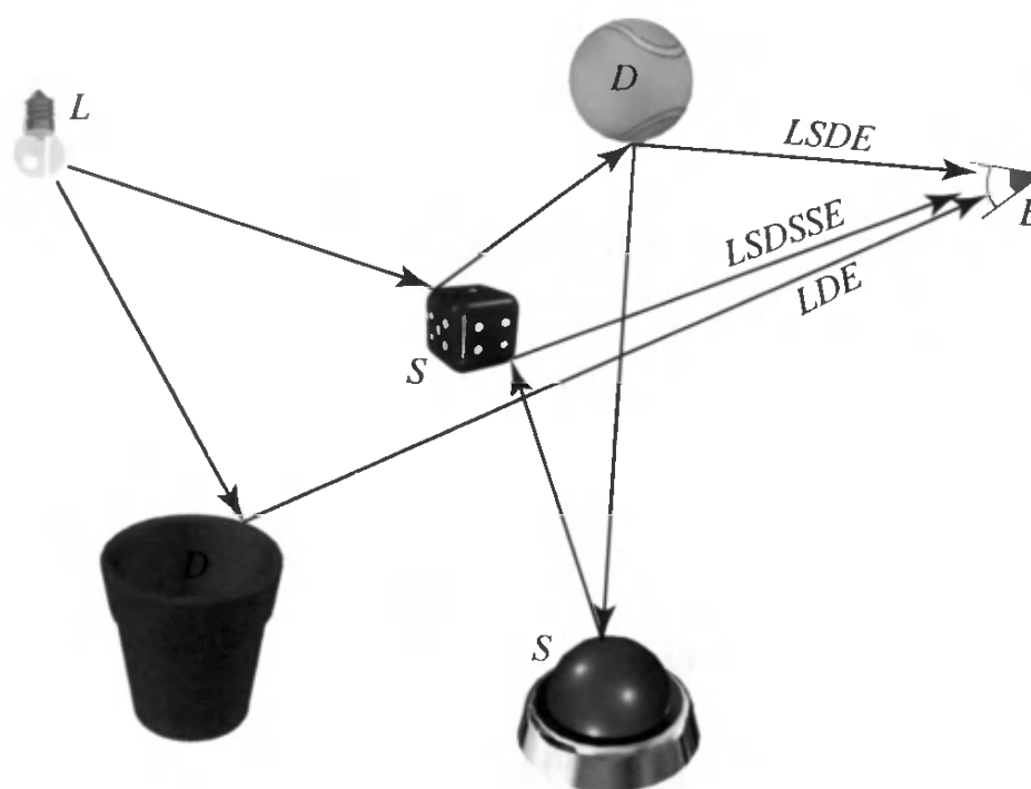
Figure 9.2. Some paths and their equivalent notation.
