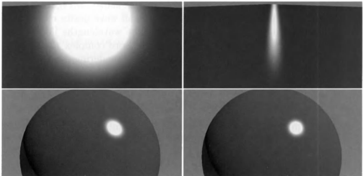
Figure 7.33. Renderings of a plane and sphere with both reflection-vector-based (on the left) and half-vector-based (on the right) BRDFs. The top row shows a flat plane with glancing viewing and lighting angles. The left side shows the circular highlight typical of reflection-vector-based BRDFs in this situation; the right side shows the narrow highlight typical of half-vector-based BRDFs. The bottom row shows a sphere; the difference in highlight shape is far more subtle in this case, where the surface curvature is the dominating factor, rather than the BRDF.
