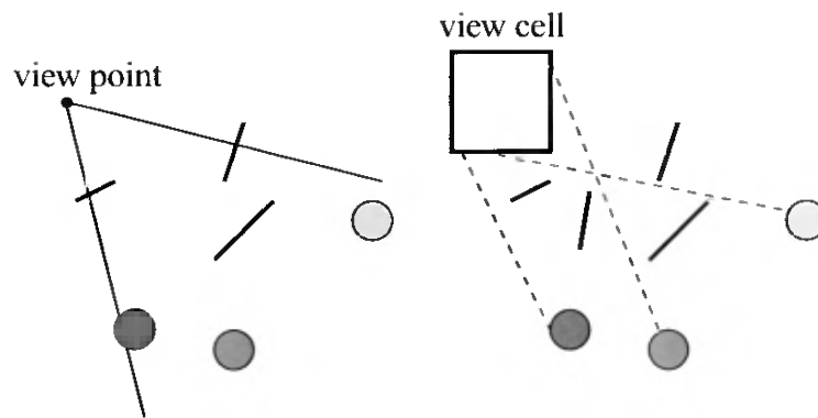
Figure 14.17. The left figure shows point-based visibility, while the right shows cell-based visibility, where the cell is a box. As can be seen, the circles are occluded to the left from the viewpoint. To the right, however, the circles are visible, since rays can be drawn from somewhere within the cell to the circles without intersecting any occluder.
