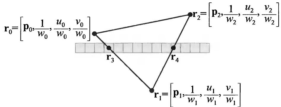
Figure 18.7. A triangle being rasterized. The vectors \mathbf{r}_i are linearly interpolated over the triangle.
