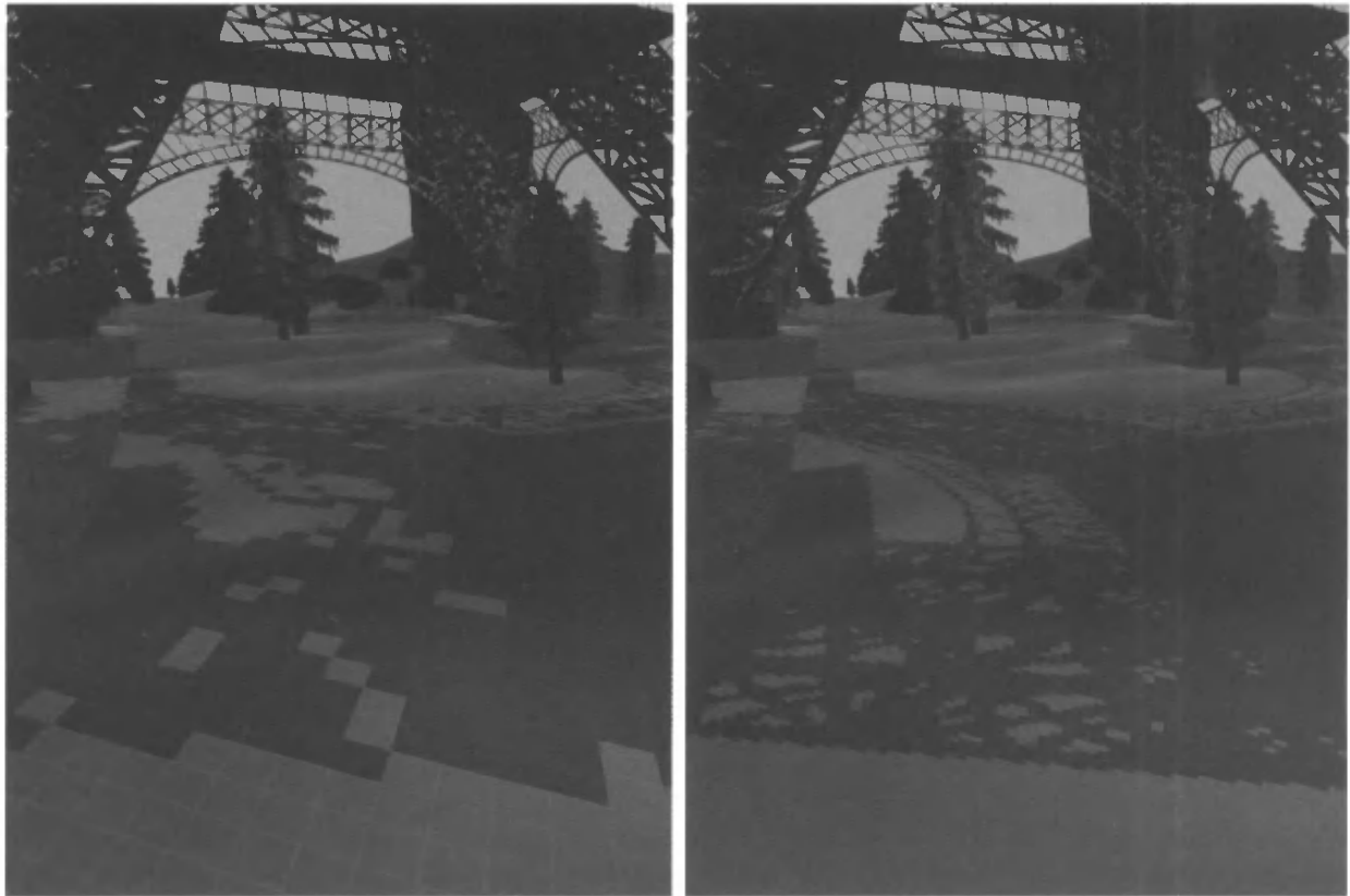
Figure 9.22. The image to the left is created using standard shadow mapping; the image to the right using LiSPSM. The projections of each shadow map's texels are shown. The two shadow maps have the same resolution, the difference being that LiSPSM reforms the light's matrices to provide a higher sampling rate nearer the viewer. (Images courtesy of Daniel Scherzer, Vienna University of Technology.)
