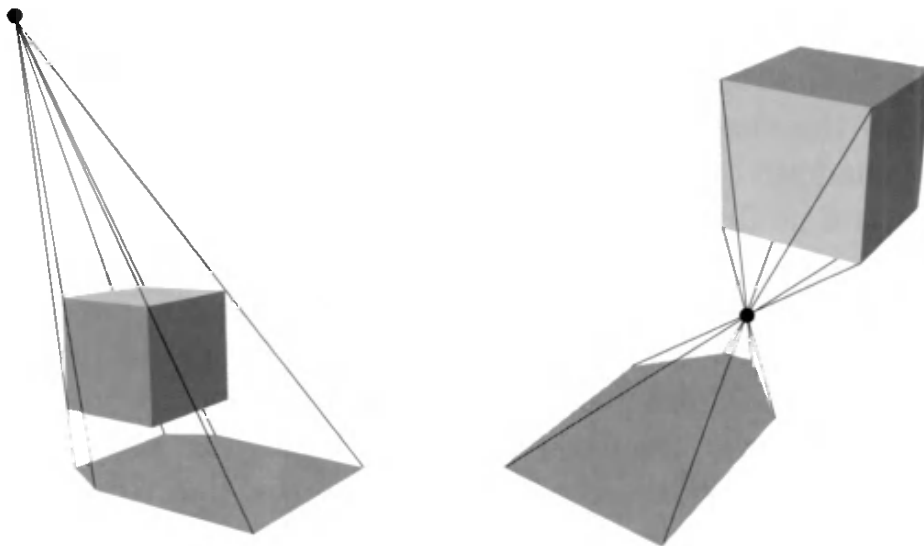
Figure 9.6. At the left, a correct shadow is shown, while in the figure on the right, an antishadow appears, since the light source is below the topmost vertex of the object.
