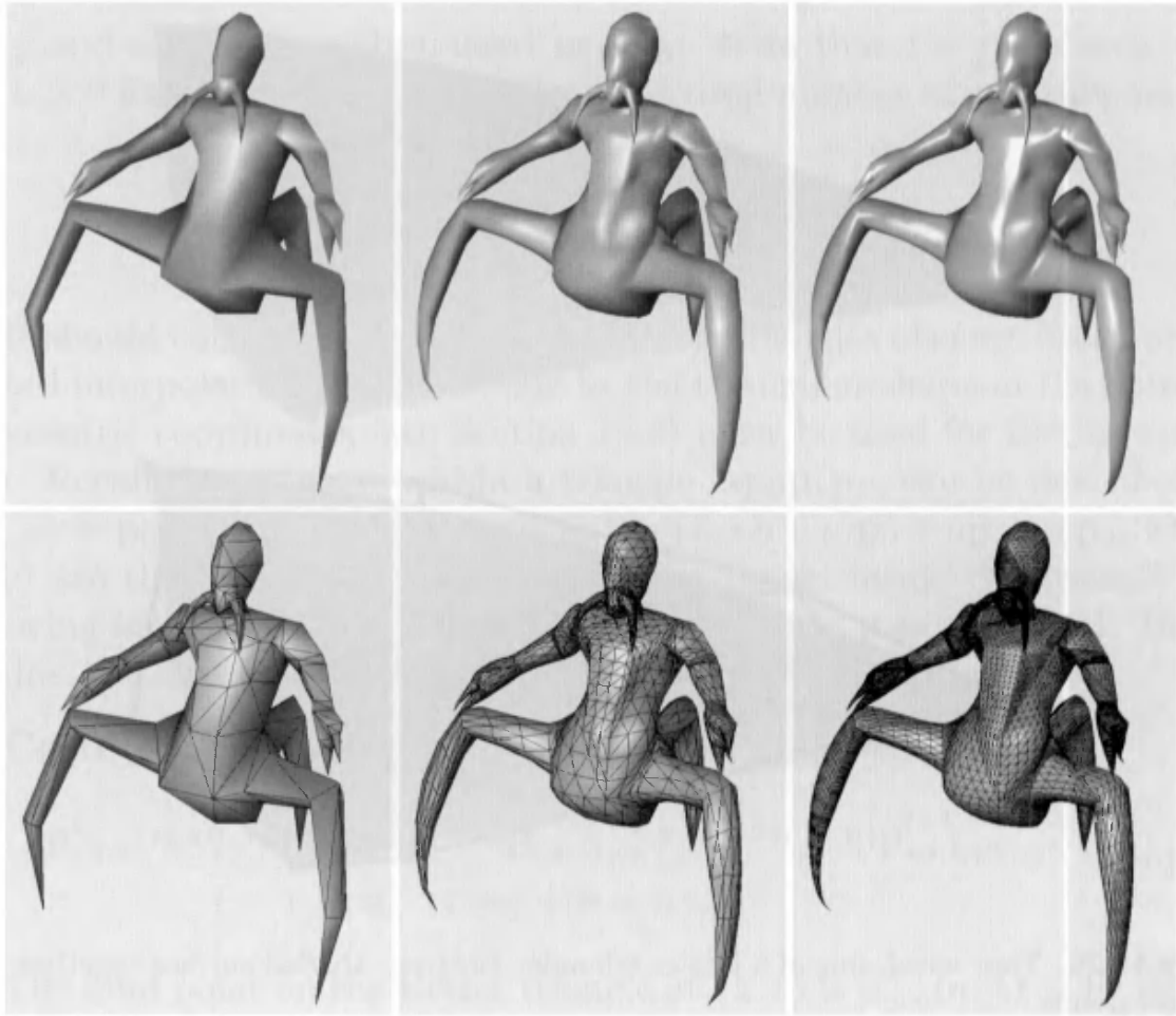
Figure 13.21. The columns show different levels of detail of the same model. The original triangle data, consisting of 414 triangles, is shown on the left. The middle model has 3,726 triangles, while the right has 20,286 triangles, all generated with the presented algorithm. Note how the silhouette and the shading improve. The bottom rows show the models in wireframe, which reveals that each original triangle generates the same amount of subtriangles. ( Model courtesy of id Software. Image from ATI Technologies Inc. demo. )
