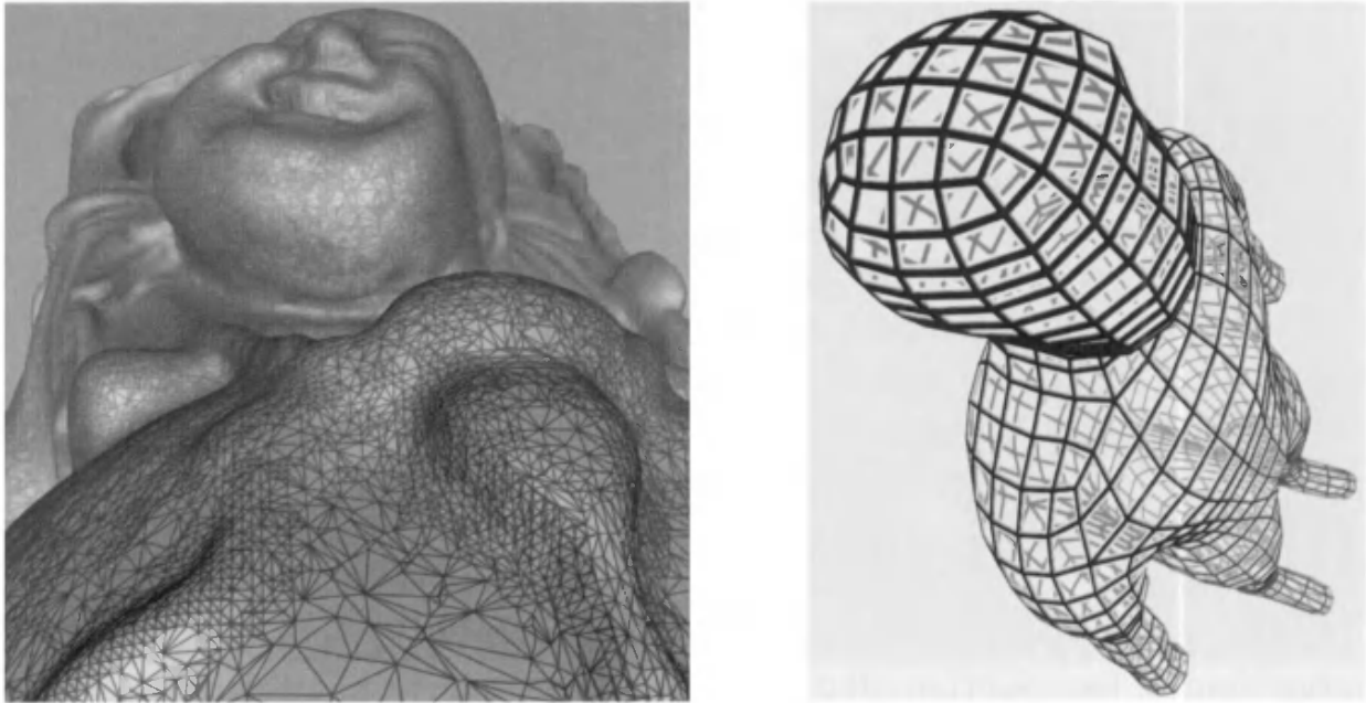
Figure 11.17. Pixel-shader-generated lines. On the left are antialiased single-pixel width edges; on the right are variable thickness lines with haloing. ( Images courtesy of J. Andreas Bærentzen. )
