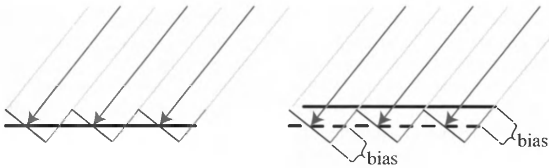
Figure 9.17. A shadow map samples a surface at discrete locations, shown by the blue arrows. The gray walls show the shadow map texel boundaries. Within each texel, the red line represents the distance that the shadow map stores for the surface, i.e., where it considers the surface to be located. Where the actual surface is below these red (and dark gray) lines, its distance is greater than the stored depth for that texel, so will be considered, erroneously, to be in shadow. By using a bias to shift the receiver so that it is considered above the red texel depth lines, no self-shadowing occurs. (After Schüler [1138].)
