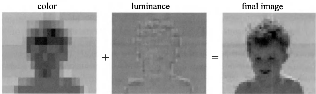
Figure 6.21. ETC (Ericsson texture compression) encodes the color of a block of pixels and then modifies the luminance per pixel to create the final texel color.
