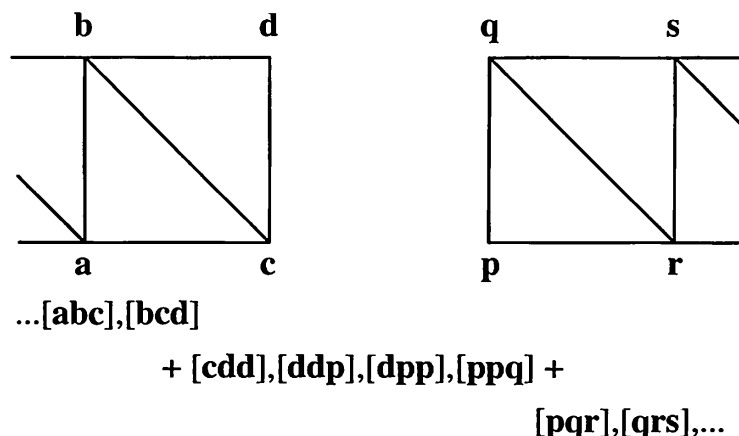
Figure 12.15. Two triangle strips are joined by replicating the end vertex d and beginning vertex p , forming four degenerate triangles. (Illustration after Huddy [573].)
