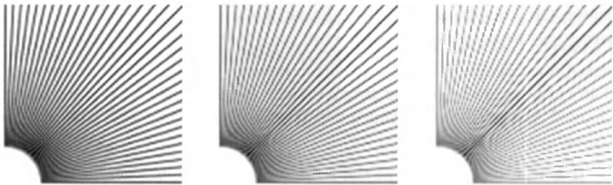
Figure 5.41. On the left, the set of antialiased lines are gamma-corrected; in the middle, the set is partially corrected; on the right, there is no gamma correction. (Images courtesy of Scott R. Nelson.)
