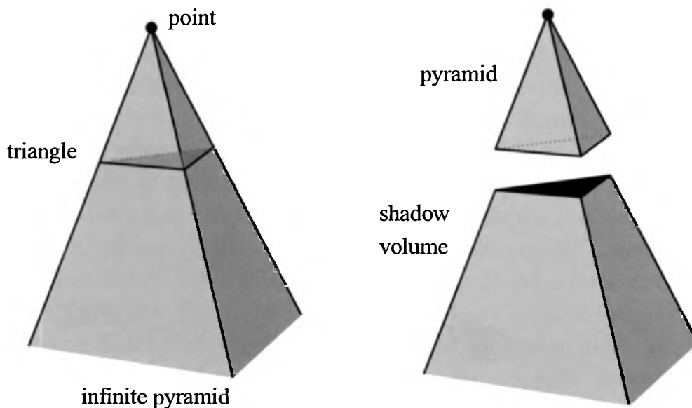
Figure 9.10. Left: The lines from a point light are extended through the vertices of a triangle to form an infinite pyramid. Right: The upper part is a pyramid, and the lower part is an infinite truncated pyramid, also called the shadow volume. All geometry that is inside the shadow volume is in shadow.
