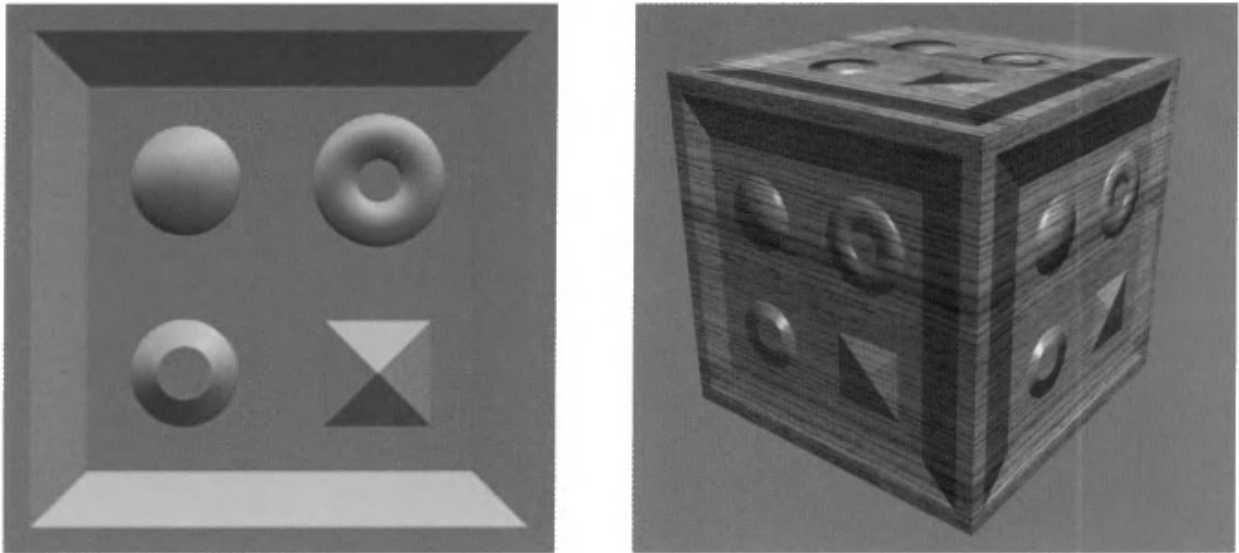
Figure 6.29. Bump mapping with a normal map. Each color channel is actually a surface normal coordinate. The red channel is the x deviation; the more red, the more the normal points to the right. Green is the y deviation, and blue is z . At the right is an image produced using the normal map. Note the flattened look on the top of the cube. ( Images courtesy of Manuel M. Oliveira and Fabio Polcarpo. )
