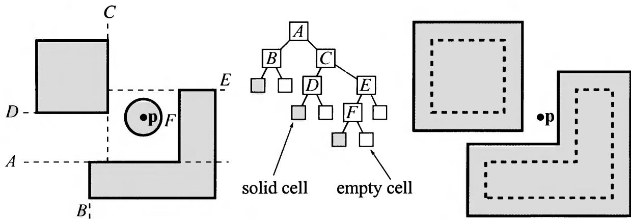
Figure 17.3. To the left is some geometry (blue) seen from above. Its BSP tree is shown in the middle. To test this tree against a circle with origin at p , the BSP tree is grown outwards with the circle's radius, and then the point p can instead be tested against the grown BSP tree. This is shown to the right. Notice that the corners should really be rounded, so this is an approximation that the algorithm introduces.
