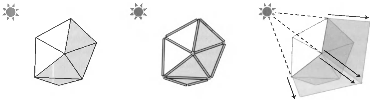
Figure 9.14. Forming a shadow volume using the vertex shader. This process is done twice, once for each of the two stencil buffer passes. The occluder is shown in the left figure. In the middle figure, all its edges are sent down as degenerate quadrilaterals, shown schematically here as thin quadrilaterals. On the right, those edges found by the vertex shader to be silhouette edges have two of their vertices projected away from the light, so forming quadrilaterals that define the shadow volume sides. Edges that are not silhouettes render as degenerate (no area) polygons and so cover no pixels.
