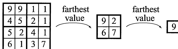
Figure 14.20. On the left, a 4 \times 4 piece of the Z -buffer is shown. The numerical values are the actual z -values. This is downsampled to a 2 \times 2 region where each value is the farthest (largest) of the four 2 \times 2 regions on the left. Finally, the farthest value of the remaining four z -values is computed. These three maps compose an image pyramid that is called the hierarchical Z -buffer.
