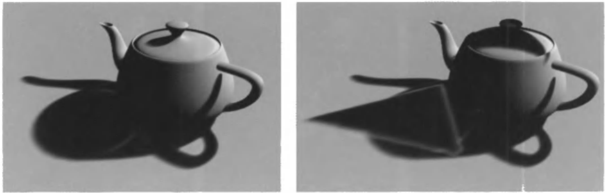
Figure 9.34. On the left, variance shadow mapping applied to a teapot. On the right, a triangle (not shown) casts a shadow on the teapot, causing objectionable artifacts in the shadow on the ground. (Images courtesy of Marco Salvi.)
