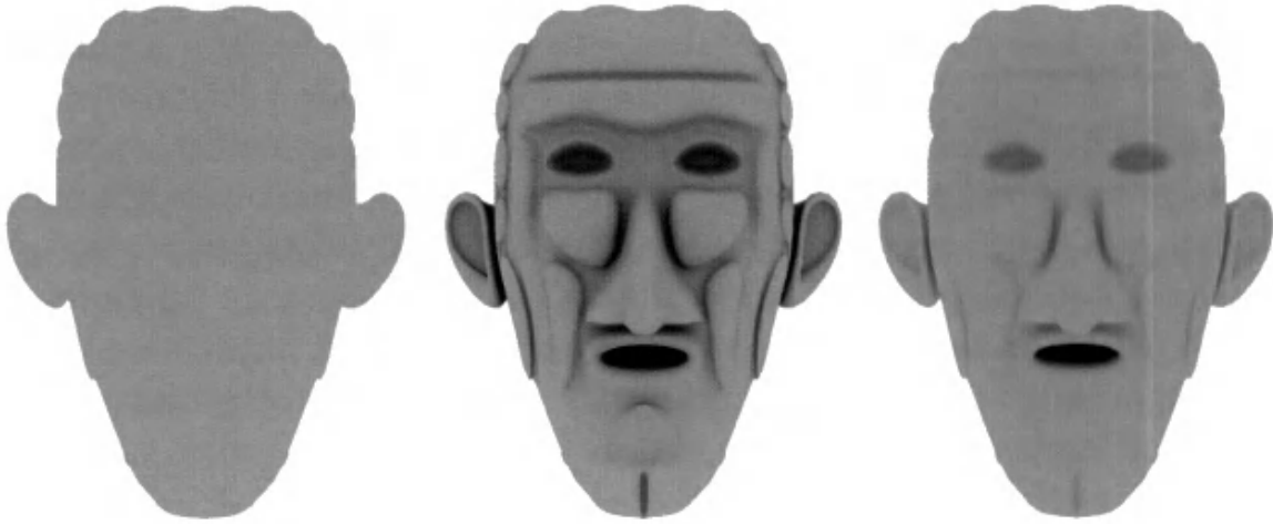
Figure 9.36. A diffuse object lit evenly from all directions. On the left, the object is rendered without any shadowing or interreflections. No details are visible, other than the outline. In the center, the object has been rendered with ambient occlusion. The image on the right was generated with a full global illumination simulation. (Images generated using the Microsoft SDK [261] sample “PRTDemo.”)
