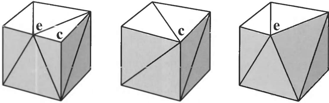
Figure 12.23. The left figure shows a cube with an extra point along one edge. The middle figure shows what happens if this point e is collapsed to corner c . The right figure shows c collapsed to e .
