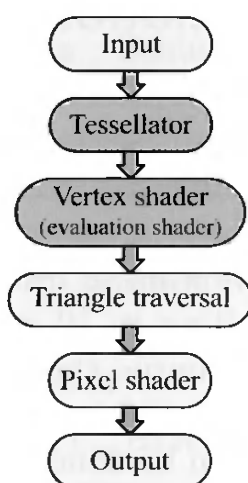
Figure 13.52. Pipeline with hardware tessellator. The new parts are in blue, where the geometrical primitives, e.g., triangles, are tessellated into many smaller primitives in the tessellator. These generated vertices are sent to the vertex shader, which is basically a standard vertex shader, except that it also knows the parametric coordinates of the vertex inside the primitive. This makes it possible to compute the three-dimensional position and normal of the vertex within the vertex shader.
