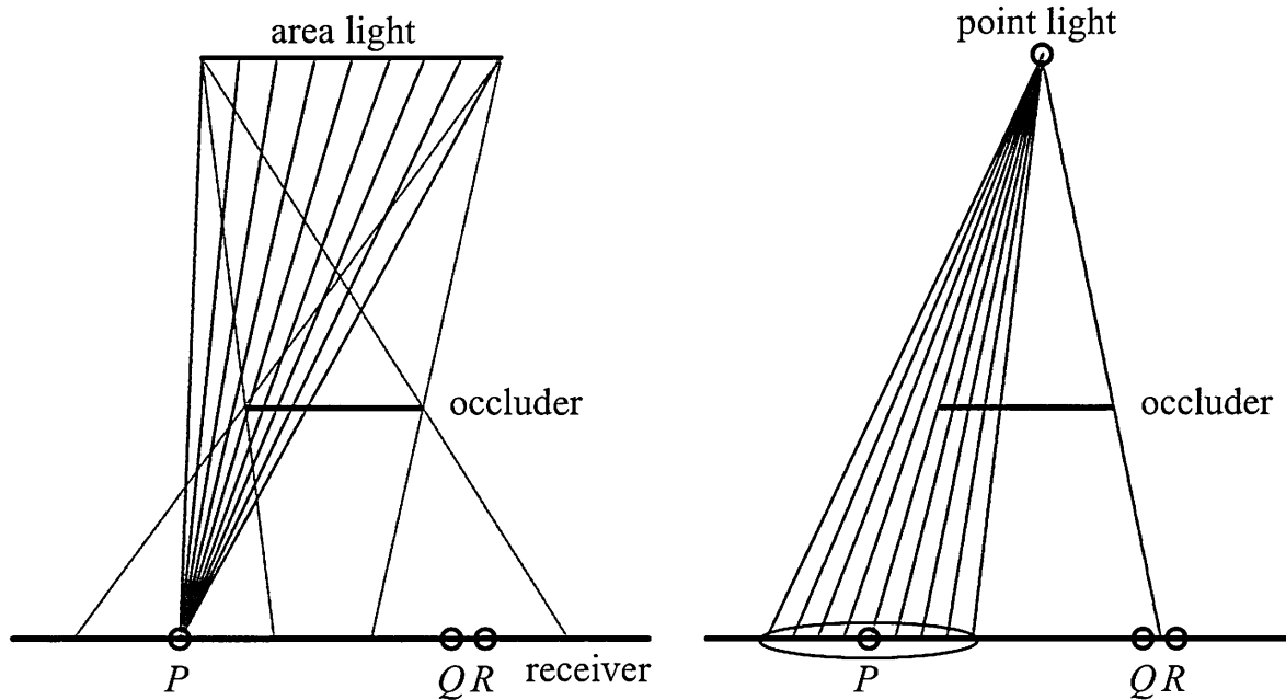
Figure 9.27. On the left, the brown lines from the area light source show where penumbras are formed. For a single point P on the receiver, the amount of illumination received could be computed by testing a set of points on the area light's surface and finding which are not blocked by any occluders. On the right, a point light does not cast a penumbra. PCF approximates the effect of an area light by reversing the process: At a given location, it samples over a comparable area on the shadow map to derive a percentage of how many samples are illuminated. The red ellipse shows the area sampled on the shadow map. Ideally, the width of this disk is proportional to the distance between the receiver and occluder.
