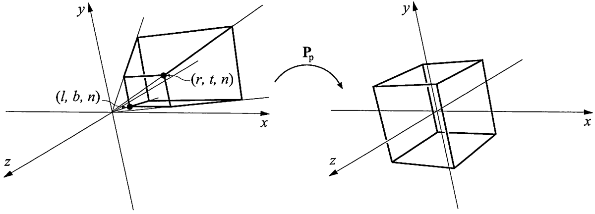
Figure 4.19. The matrix \mathbf{P}_p transforms the view frustum into the unit cube, which is called the canonical view volume.
