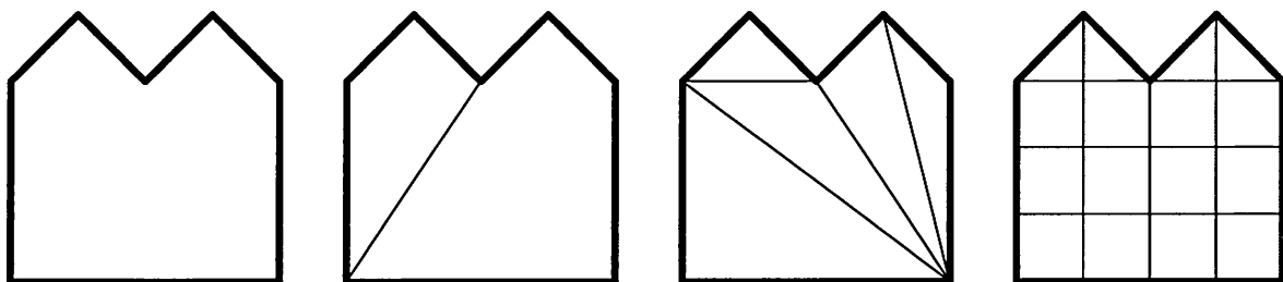
Figure 12.1. Various types of tessellation. The leftmost polygon is not tessellated, the next is partitioned into convex regions, the next is triangulated, and the rightmost is uniformly meshed.
