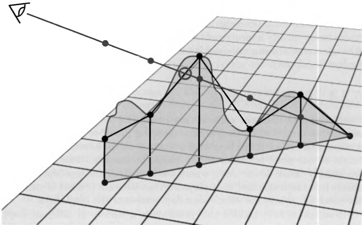
Figure 6.33. The green eye ray is projected onto the surface plane, which is sampled at regular intervals (the violet dots) and the heights are retrieved. The algorithm finds the first intersection of the eye ray with the black line segments approximating the curved height field.
