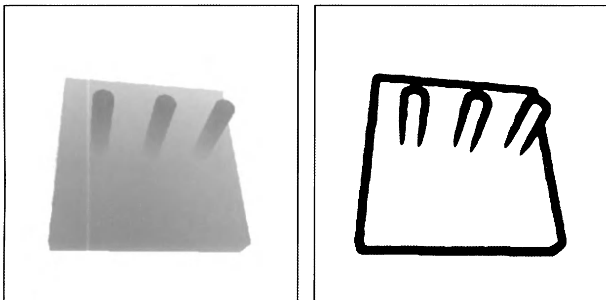
Figure 9.28. The depth map on the left has edge detection and dilation applied, to create an edge map, on the right. This map identifies potential penumbra areas. Time is saved by applying PCF to only these areas and using single samples for the rest. ( Images courtesy of John Isidoro, ATI Research, Inc. )
