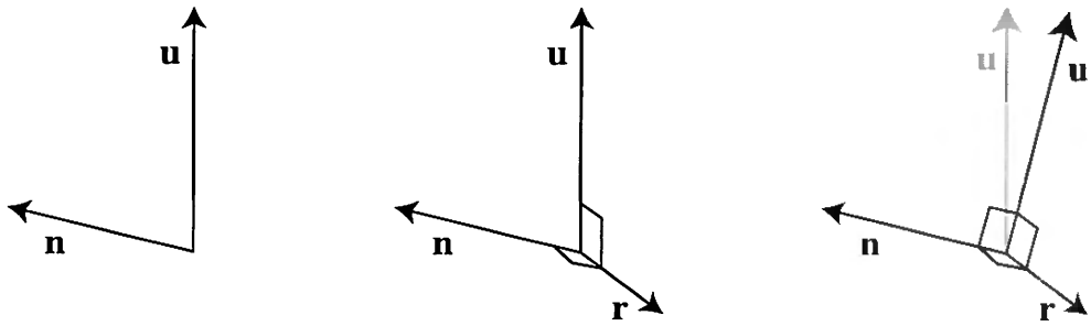
Figure 10.4. Given a desired surface normal direction \mathbf{n} and an approximate up vector direction \mathbf{u} , we wish to establish a set of three mutually perpendicular vectors to orient the billboard. In the middle figure, the “right” vector \mathbf{r} is found by taking the cross product of \mathbf{u} and \mathbf{n} , and so is perpendicular to both of them. In the right figure, the fixed vector \mathbf{n} is crossed with \mathbf{r} to give a mutually perpendicular up vector \mathbf{u}' .
