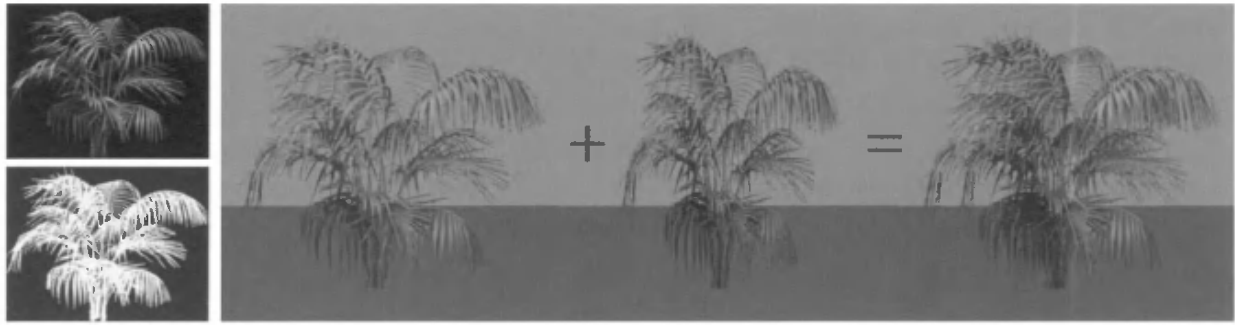
Figure 6.24. On the left, the bush texture map and the 1-bit alpha channel map below it. On the right, the bush rendered on a single polygon; by adding a second copy of the polygon rotated 90 degrees, we form an inexpensive three-dimensional bush.
