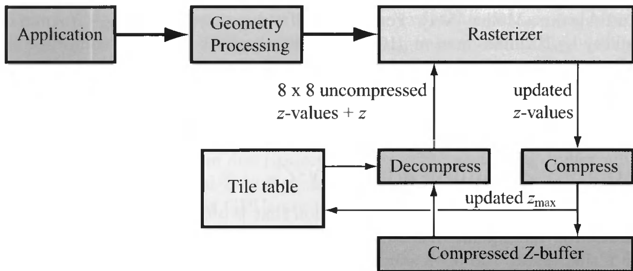
Figure 18.14. Block diagram of hardware techniques for fast clear of the Z -buffer, compression of Z -buffer, and Z -culling. Applies to other types of buffers too.
