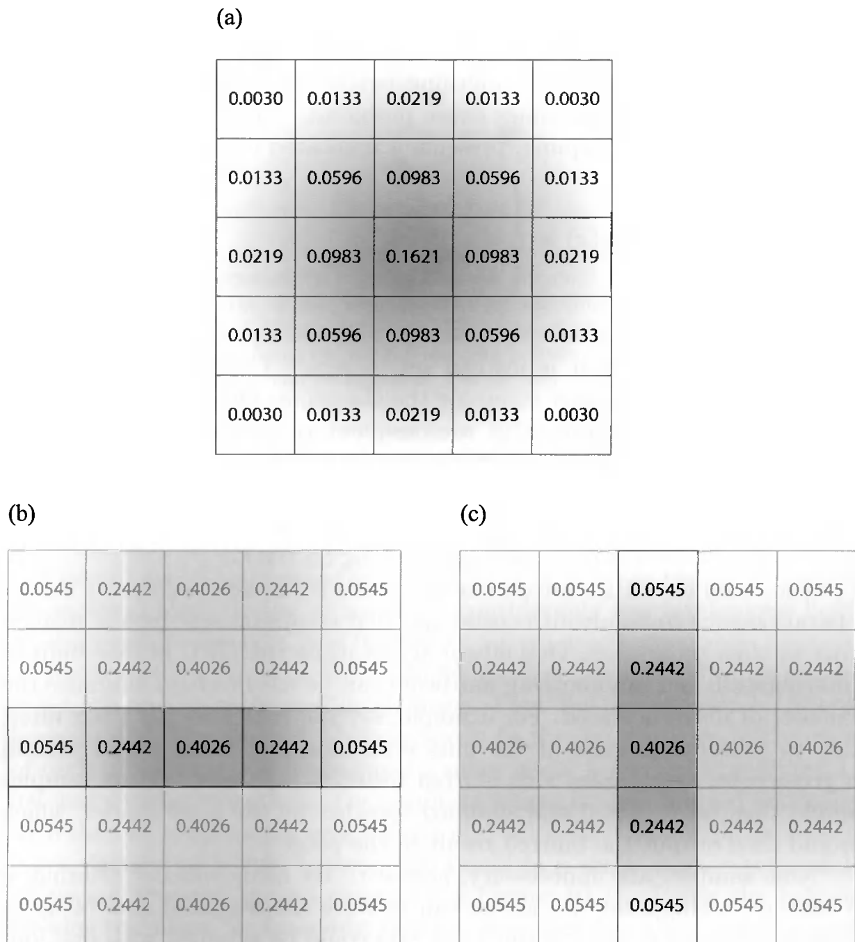
Figure 10.21. One way to use a Gaussian blur kernel is to sample a 5 \times 5 area, weighting each contribution and summing them. Part (a) of the figure shows these weights for a blur kernel with \sigma = 1 . Using separable filters, two one-dimensional Gaussian blurs, (b) and (c), are performed, with the same net result. The first pass, shown in (b) for 5 separate rows, blurs each pixel horizontally using 5 samples in its row. The second pass, (c), applies a 5-sample vertical blur filter to the resulting image from (b) to give the final result. Multiplying the weights in (b) by those in (c) gives the same weights as in (a), showing that this filter is equivalent and therefore separable. Instead of needing 25 samples, as in (a), each of (b) and (c) effectively each use 5 per pixel, for a total of 10 samples.
