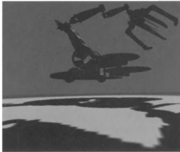
Figure 9.19. Perspective aliasing stairstepping artifacts due to the shadow map projection being magnified.
