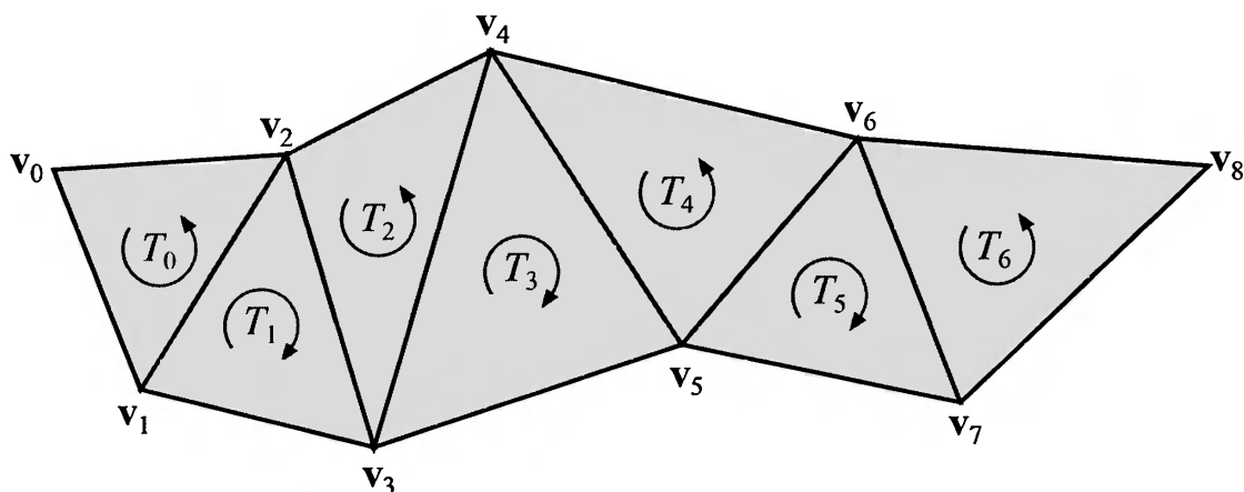
Figure 12.13. A sequence of triangles that can be represented as one triangle strip. Note that the orientation changes from triangle to triangle in the strip, and that the first triangle in the strip sets the orientation of all triangles. Internally, counterclockwise order is kept consistent by traversing vertices 0-1-2, 1-3-2, 2-3-4, 3-5-4, and so on.
