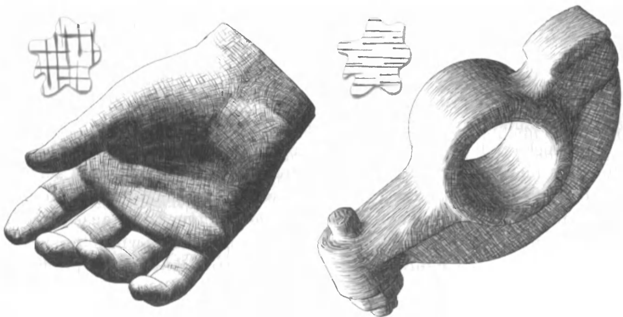
Figure 11.15. Two models rendered using tonal art maps (TAMs) . The swatches show the lapped texture pattern used to render each. (Images courtesy of Emil Praun, Princeton University.)
