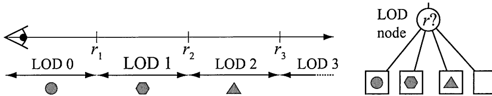
Figure 14.26. The left part of this illustration shows how range-based LODs work. Note that the fourth LOD is an empty object, so when the object is farther away than r_3 , nothing is drawn, because the object is not contributing enough to the image to be worth the effort. The right part shows a LOD node in a scene graph. Only one of the children of a LOD node is descended based on r .
