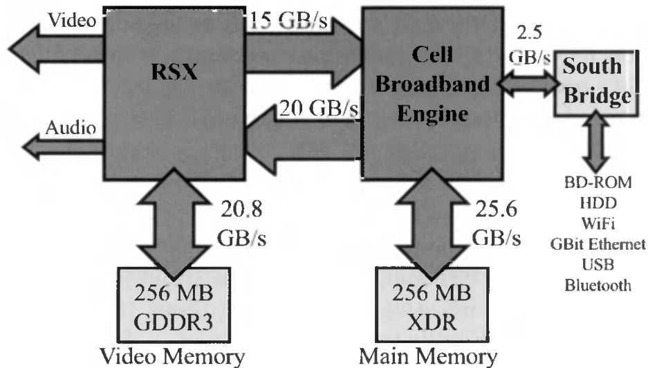
Figure 18.17. PLAYSTATION 3 architecture. (Illustration after Perthuis [1002].)
