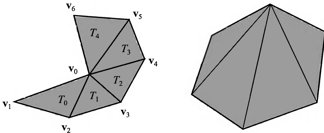
Figure 12.12. The left figure illustrates the concept of a triangle fan. Triangle T_0 sends vertices \mathbf{v}_0 (the center vertex), \mathbf{v}_1 , and \mathbf{v}_2 . The subsequent triangles, T_i ( i > 0 ), send only vertex \mathbf{v}_{i+2} . The right figure shows a convex polygon, which can always be turned into one triangle fan.
