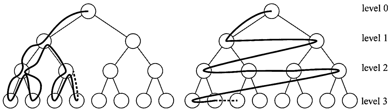
Figure 17.14. Depth-first (left) versus breadth-first (right) traversal. Depth-first traversal is often used in collision detection when traversing the bounding volume hierarchies, but for time-critical CD, breadth-first traversal is used.
