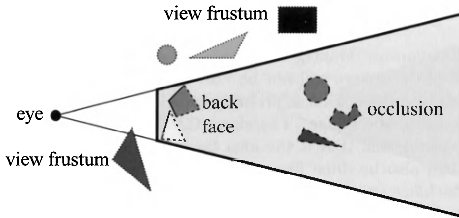
Figure 14.9. Different culling techniques. Culled geometry is dashed. (Illustration after Cohen-Or et al. [185].)
