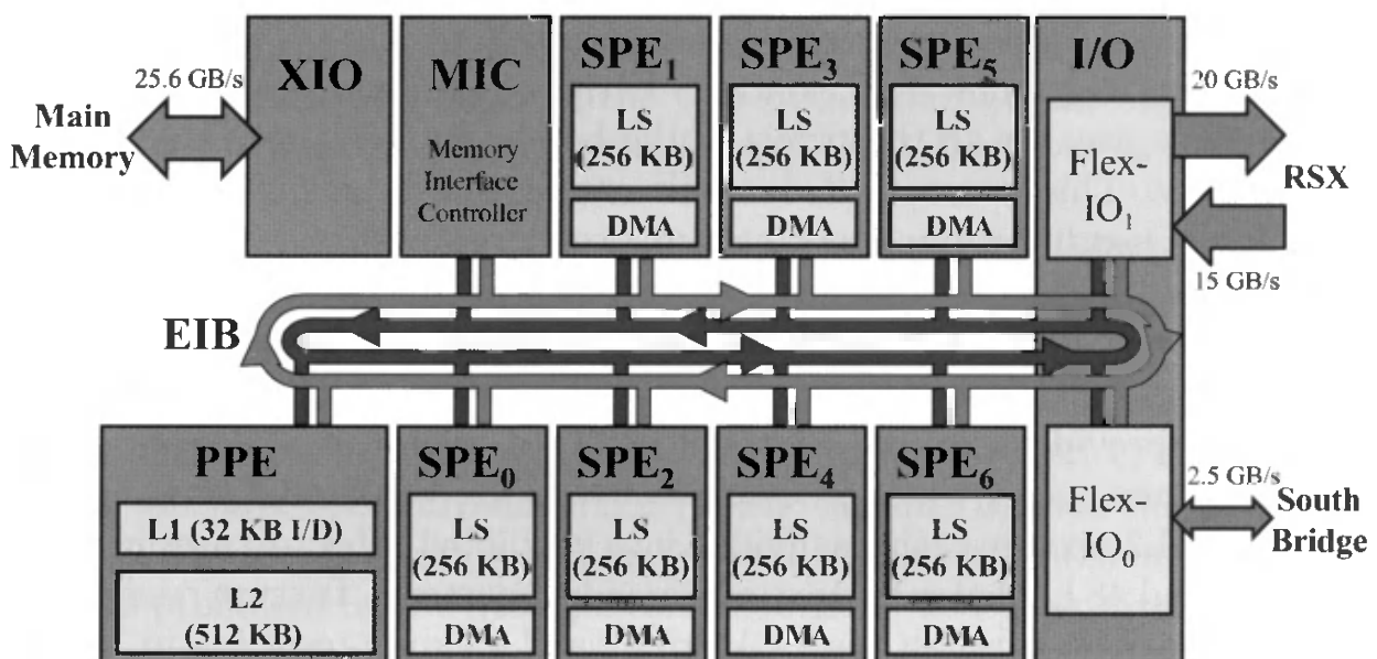
Figure 18.19. Cell Broadband Engine architecture. (Illustration after Perthuis [1002].)
