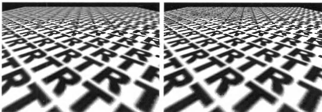
Figure 6.18. Mipmap versus anisotropic filtering. Trilinear mipmapping has been done on the left, and 16:1 anisotropic filtering on the right, both at a 640 \times 450 resolution, using ATI Radeon hardware. Towards the horizon, anisotropic filtering provides a sharper result, with minimal aliasing.
