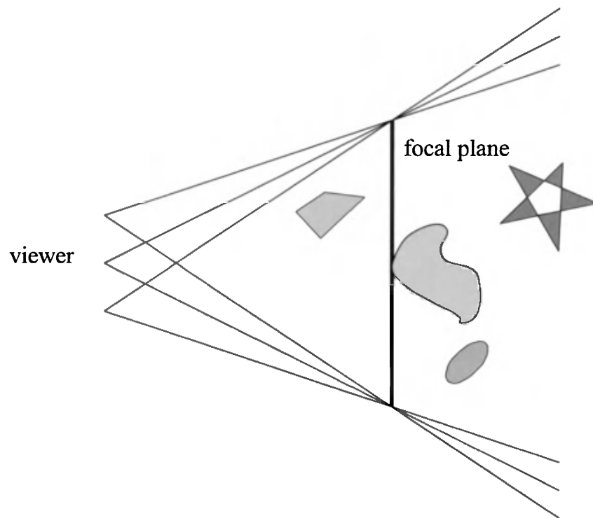
Figure 10.29. Depth of field via accumulation. The viewer's location is moved a small amount, keeping the view direction pointing at the focal point, and the images are accumulated.
