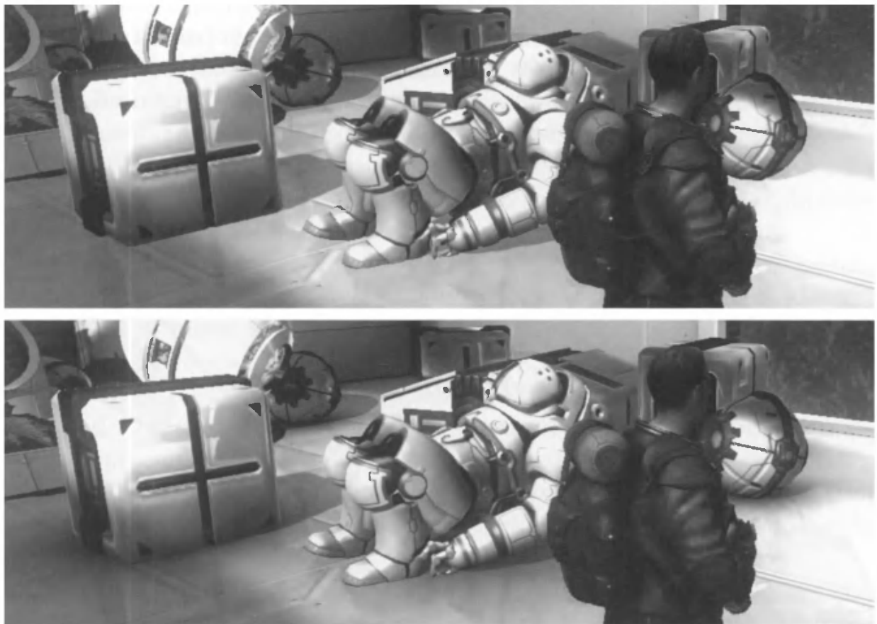
Figure 9.66. On the top, objects cast shadows on the floor but with no ambient effect. On the bottom, ambient occlusion fields from the objects cause the floor to darken near them. These subtle touches give a richness to the lighting in the scene. (Images courtesy of Emergent Game Technologies and Third Degree Games.)
