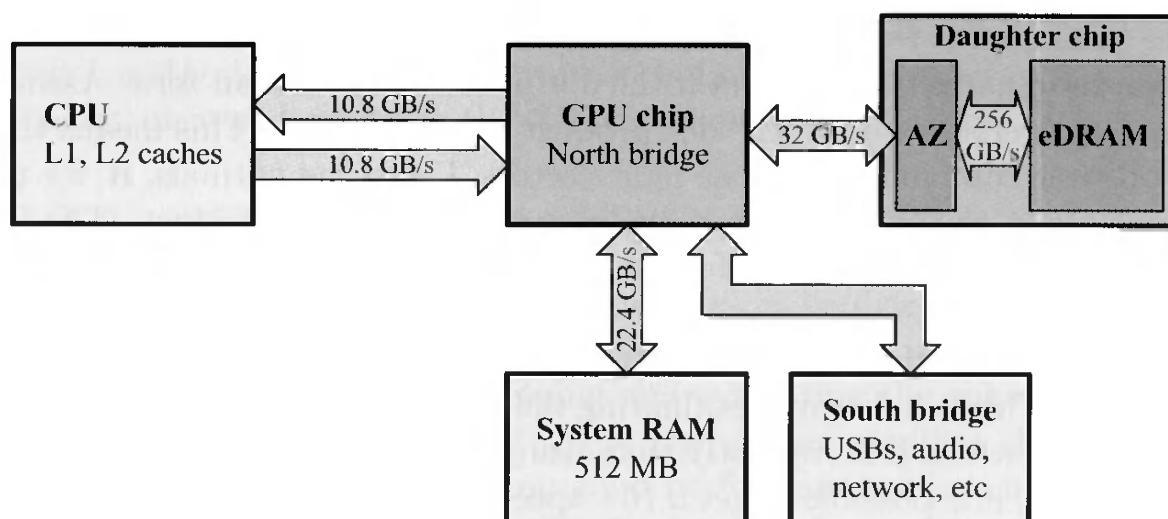
Figure 18.15. Xbox 360 memory architecture.
