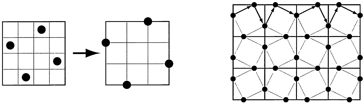
Figure 5.34. To the left, the RGSS sampling pattern is shown. This costs four samples per pixel. By moving these out to the pixel edges, sample sharing can occur across edges. However, for this to work out, every other pixel must have a reflected sample pattern, as shown on the right. The resulting sample pattern is called FLIPQUAD and costs two samples per pixel
