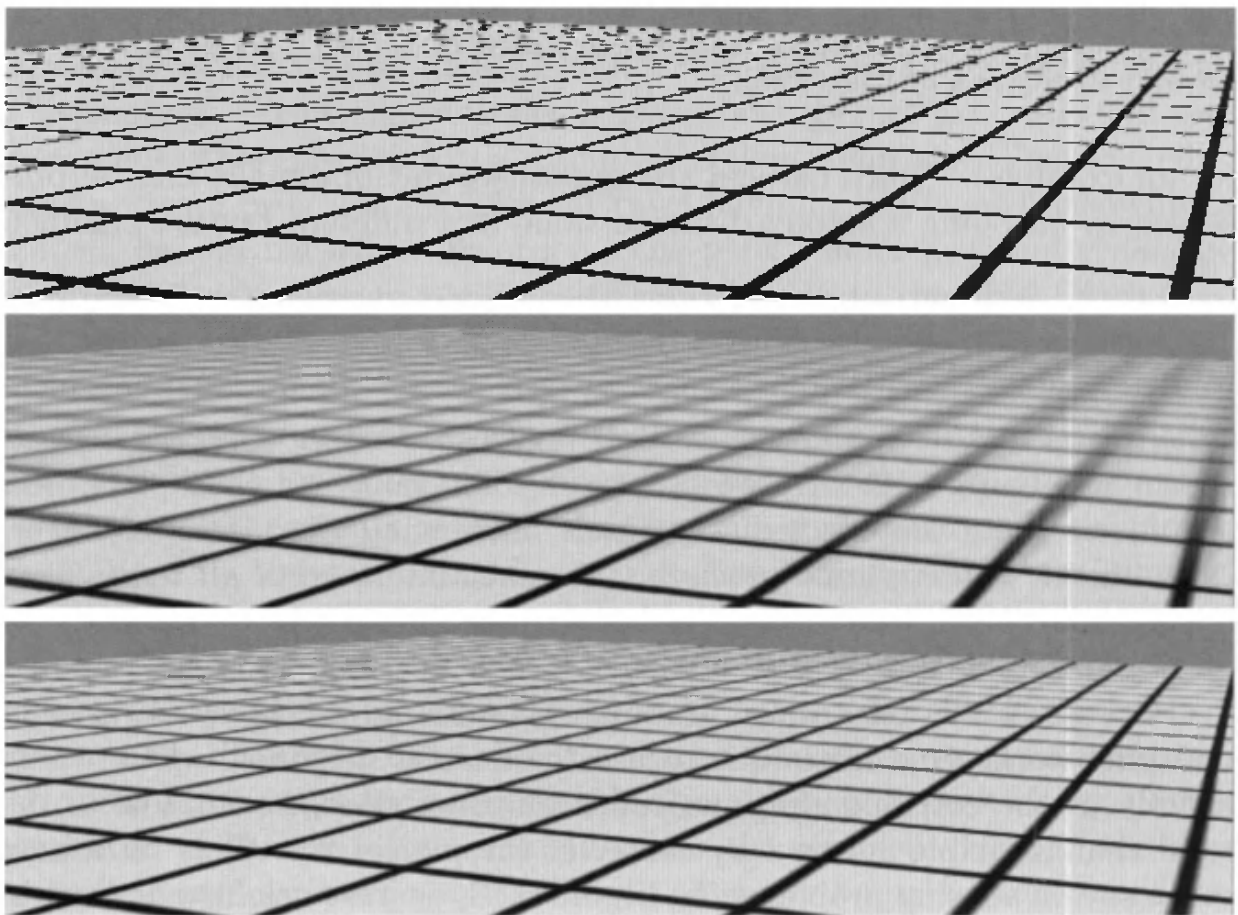
Figure 6.13. The top image was rendered with point sampling (nearest neighbor), the center with mipmapping, and the bottom with summed area tables.
