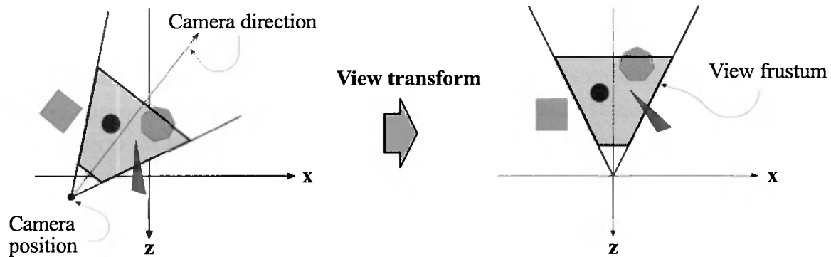
Figure 2.4. In the left illustration, the camera is located and oriented as the user wants it to be. The view transform relocates the camera at the origin, looking along the negative z-axis, as shown on the right. This is done to make the clipping and projection operations simpler and faster. The light gray area is the view volume. Here, perspective viewing is assumed, since the view volume is a frustum. Similar techniques apply to any kind of projection.
