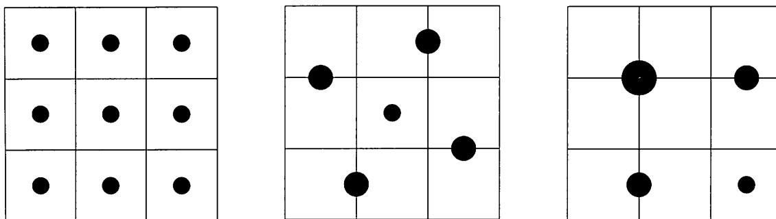
Figure 10.22. On the left, a box filter is applied by performing nine texture samples and averaging the contributions together. In the middle, a symmetric pattern of five samples is used, with the outside samples each representing two texels, and so each is given twice the weight of the center sample. This type of pattern can be useful for other filter kernels, where by moving the outside samples between their two texels, the relative contribution of each texel can be changed. On the right, a more efficient four sample pattern is used instead. The sample on the upper left interpolates between four texels' values. The ones on the upper right and lower left each interpolate the values of two texels. Each sample is given a weight proportional to the number of texels it represents.
