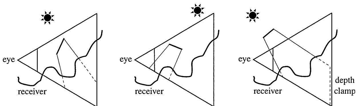
Figure 9.12. The z -pass and z -fail shadow volume methods; z -pass is shown as solid lines emanating from the occluder, z -fail as dashed lines beyond the receiver. On the left, if the z -fail method were used for the case shown, the shadow volume would need to be capped before reaching the far plane. In the middle, z -pass would give an incorrect count, as it penetrates the near plane. On the right, neither method can work without some way to avoid the clip by either the near or far plane; depth clamping’s effect is shown on z -fail.
