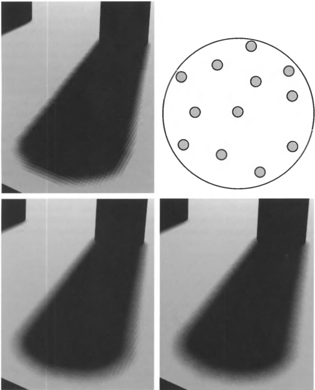
Figure 9.30. The upper left shows PCF sampling in a 4 \times 4 grid pattern. The upper right shows a 12-tap Poisson sampling pattern on a disk. Using this pattern to sample the shadow map gives the improved result on the lower left, though artifacts are still visible. On the lower right, the sampling pattern is rotated randomly around its center from pixel to pixel. The structured shadow artifacts turn into (much less objectionable) noise. (Images courtesy of John Isidoro, ATI Research, Inc.)
