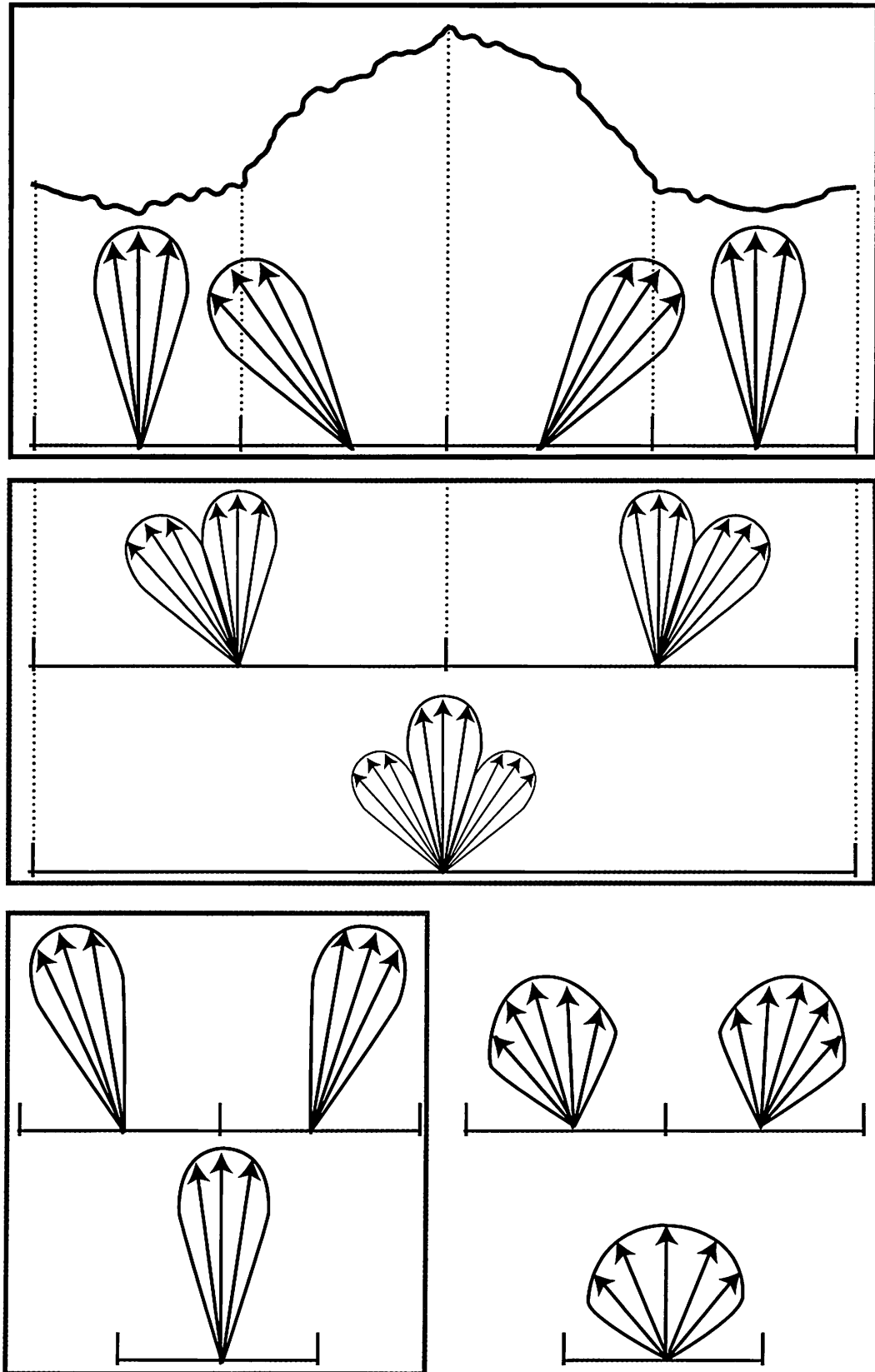
Figure 7.45. Part of the surface from Figure 7.44. The top shows the oriented NDFs, as well as the underlying surface geometry they implicitly define. The center shows ideal NDFs collected from the underlying geometry at lower resolutions. The bottom left shows the result of normal averaging, and the bottom right shows the result of cosine lobe fitting.
