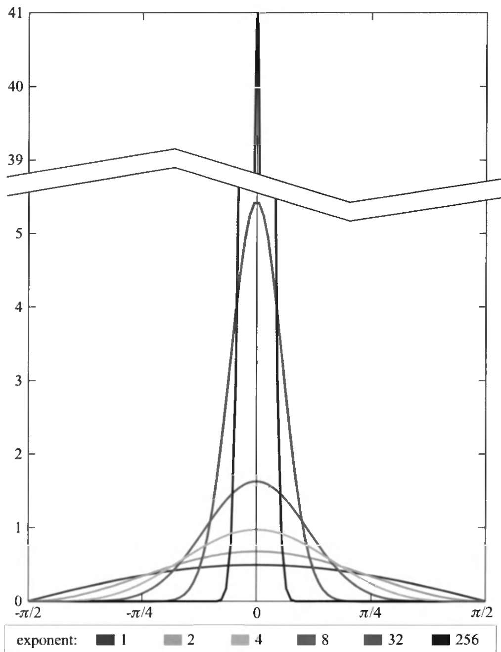
Figure 7.37. Graph of normalized cosine power term versus angle for various exponents. Increasing the exponent not only makes the curve narrower, but also higher. This increase in height compensates for the decrease in width, keeping the total reflected energy constant.
