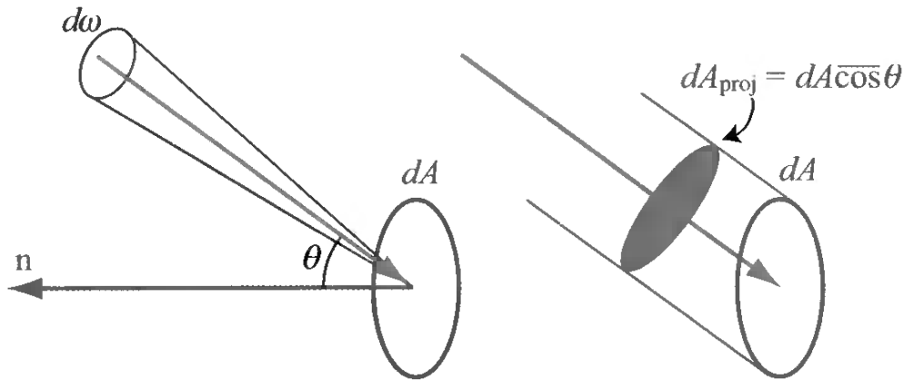
Figure 7.4. Radiance is power per unit projected area per unit solid angle.
