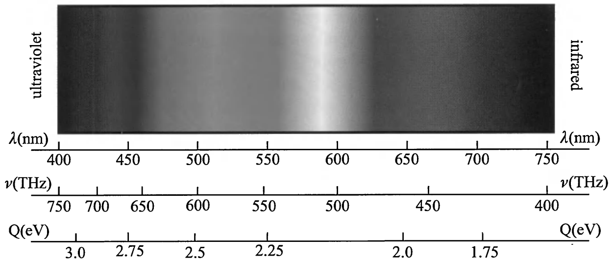
Figure 7.1. The visible spectrum. The top scale shows wavelength in nanometers, the middle scale shows frequency in terahertz ( 10^{12} Hertz), and the bottom scale shows photon energy in electron-volts (the amount of energy required to move a single electron over an electrical potential difference of one volt).
