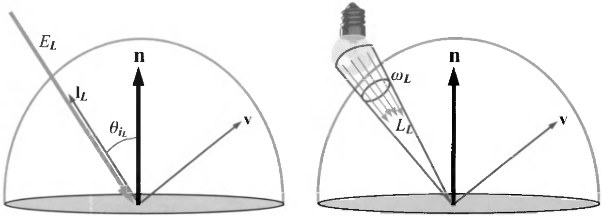
Figure 8.3. A surface illuminated by a light source. On the left, the light source is modeled as a point or directional light. On the right, it is modeled as an area light source.
