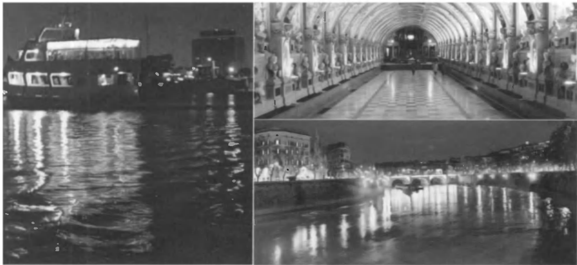
Figure 7.34. Photographs of surfaces lit and viewed at glancing angles. These surfaces clearly exhibit narrow highlights, which the highlights generated by half-vector-based BRDFs closely resemble. ( Photographs courtesy of Elan Ruskin. )
