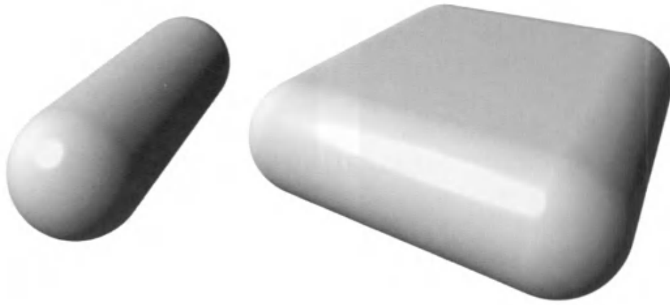
Figure 16.33. A line swept sphere (LSS) and rectangle swept sphere (RSS).
