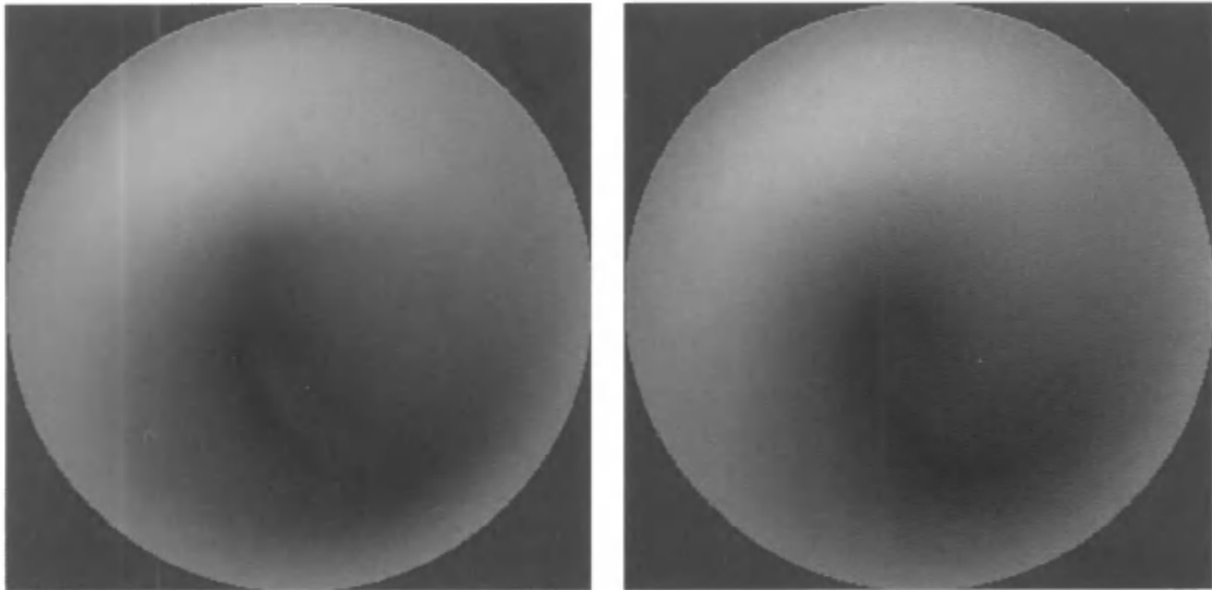
Figure 8.22. Irradiance maps formed from the Grace Cathedral sphere map. The left figure is formed by summing the weighted colors in the hemisphere above each pixel. The right figure is generated by deriving a nine-term function approximating this radiance map, then evaluating this function for each pixel. (Images courtesy of Ravi Ramamoorthi, Computer Graphics Laboratory, Stanford University.)
