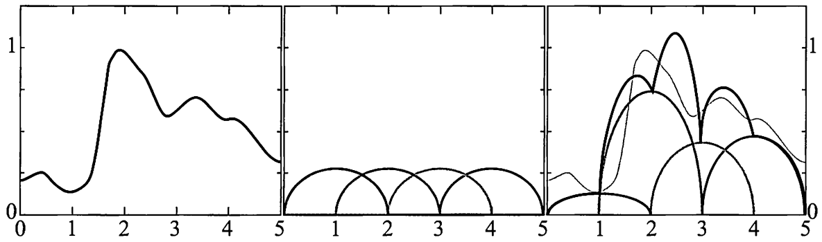
Figure 8.25. A simple example of basis functions. In this case, the space is “functions that have values between 0 and 1 for inputs between 0 and 5.” The left side shows an example of such a function. The middle shows a set of basis functions (each color is a different function). The right side shows an approximation to the target function, formed by multiplying each of the basis functions by a weight (the basis functions are shown scaled by their respective weights) and summing them (the black line shows the result of this sum, which is an approximation to the original function, shown in gray for comparison).
