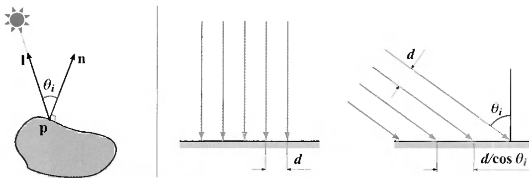
Figure 5.4. The diagram on the left shows the lighting geometry. In the center, light is shown hitting a surface straight-on, and on the right it is shown hitting the surface at an angle.
