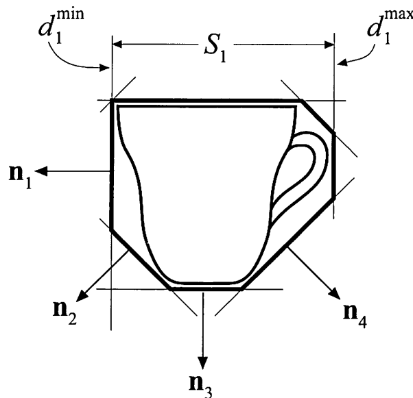
Figure 16.4. An example of a two-dimensional 8-DOP for a tea cup, with all normals, \mathbf{n}_i , shown along with the zero'th slab, S_1 , and the “size” of the slab: d_1^{\min} and d_1^{\max} .
