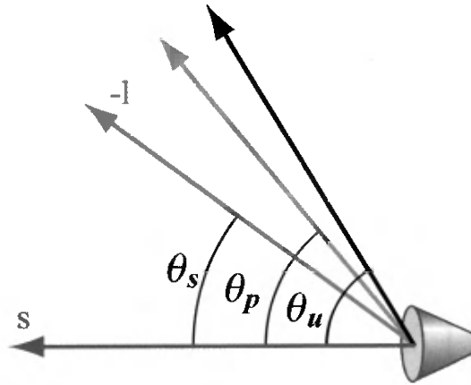
Figure 7.12. A spotlight. \theta_s is the angle from the light's defined direction \mathbf{s} to the vector -\mathbf{l} , the direction to the surface. \theta_p shows the penumbra and \theta_u the umbra angles defined for the light. Beyond the umbra angle the spotlight has no effect.
