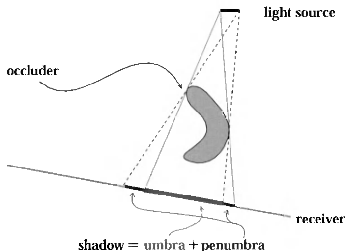
Figure 9.3. Shadow terminology: light source, occluder, receiver, shadow, umbra, and penumbra.
