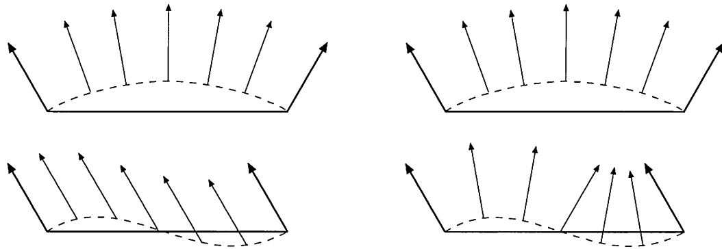
Figure 13.23. This figure illustrates why quadratic interpolation of normals is needed, and why linear interpolation is not sufficient. The left column shows what happens when linear interpolation of normals is used. This works fine when the normals describe a convex surface (top), but breaks down when the surface has an inflection (bottom). The right column illustrates quadratic interpolation. ( Illustration after van Overveld and Wyvill [1297]. )
