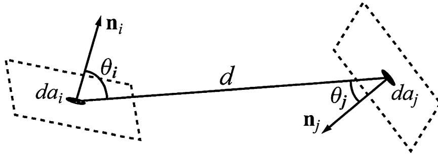
Figure 9.58. The form factor between two surface points.
