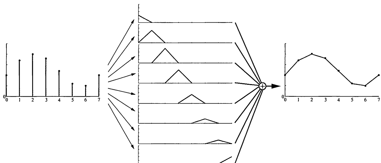
Figure 5.24. The sampled signal (left) is reconstructed using the tent filter. The reconstructed signal is shown to the right.
