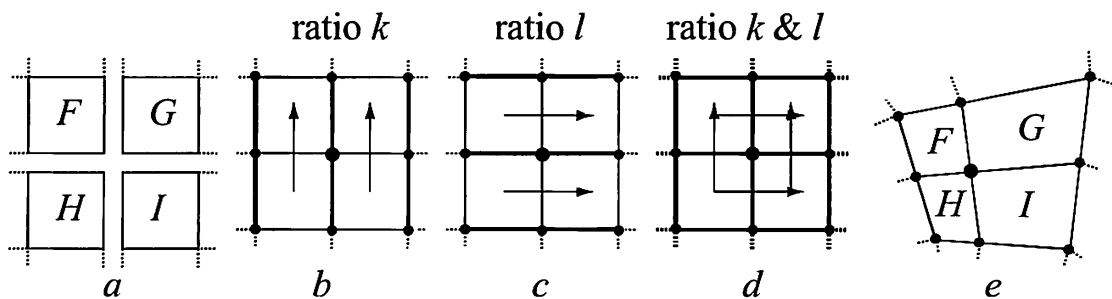
Figure 13.27. a) Four patches, F , G , H , and I , are to be stitched together, where all patches share one corner. b) In the vertical direction, the three sets of three points (on each bold line) must use the same ratio, k . This relationship is not shown here; see the rightmost figure. A similar process is done for c), where, in the horizontal direction, both patches must use the same ratio, l . d) When stitched together, all four patches must use ratio k vertically, and l horizontally. e) The result is shown, in which the ratios are correctly computed for the nine control points closest to (and including) the shared control point.
