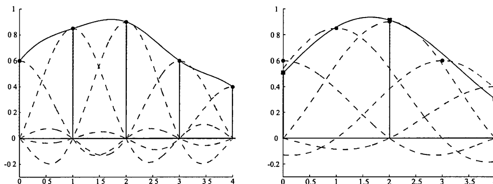
Figure 5.27. On the left is the sampled signal, and the reconstructed signal. On the right, the filter width has doubled in order to double the interval between the samples, that is, minification has taken place.
