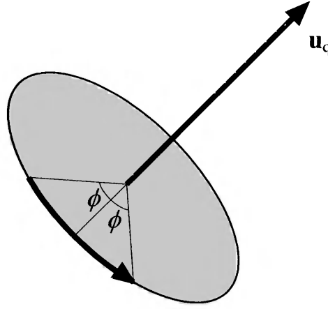
Figure 4.8. Illustration of the rotation transform represented by a unit quaternion, \hat{\mathbf{q}} = (\sin \phi \mathbf{u}_q, \cos \phi) . The transform rotates 2\phi radians around the axis \mathbf{u}_q .
