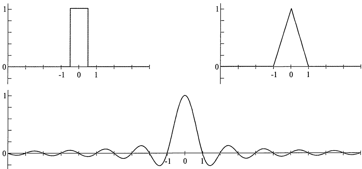
Figure 5.22. The top left shows the box filter, and the top right the tent filter. The bottom shows the sinc filter (which has been clamped on the x -axis here).
