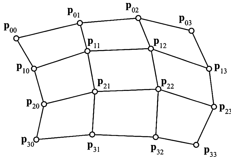
Figure 13.62. A bicubic Bézier patch with 4 \times 4 control points.
