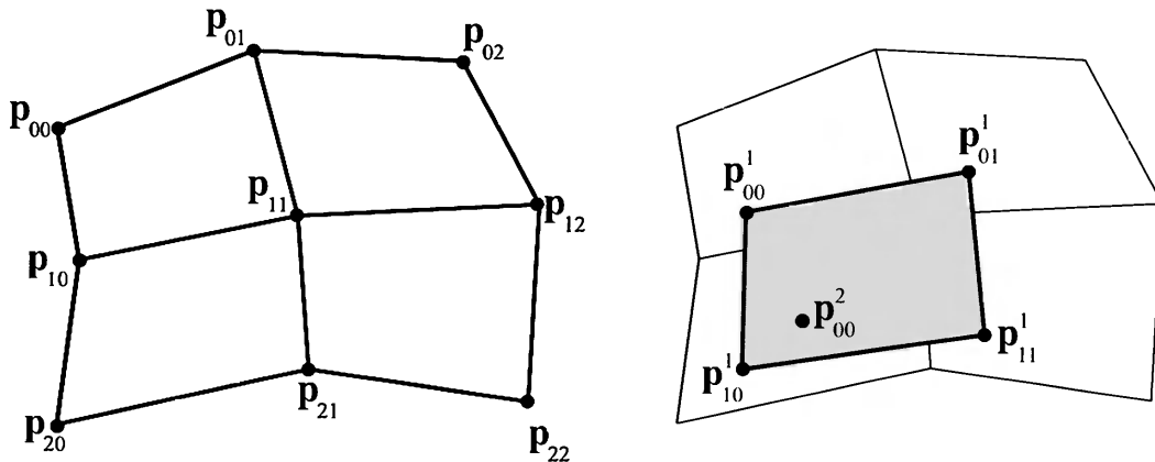
Figure 13.15. Left: a biquadratic Bézier surface, defined by nine control points, \mathbf{p}_{ij} . Right: To generate a point on the Bézier surface, four points \mathbf{p}_{ij}^1 are first created using bilinear interpolation from the nearest control points. Finally, the point surface \mathbf{p}(u, v) = \mathbf{p}_{00}^2 is bilinearly interpolated from these created points.
