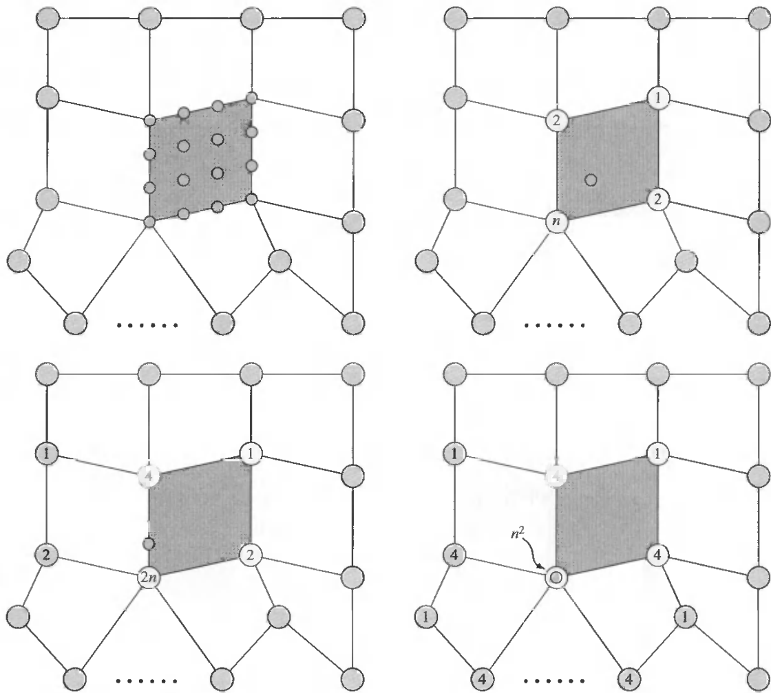
Figure 13.64. Top left: part of a quad mesh, where we want to compute a Bézier patch for the gray quad. The lower left vertex in the gray quad is extraordinary, since its valence is n \neq 4 . The blue vertices are neighboring quads' vertices, and the green circles are the control points of the Bézier patch. The following three illustrations show the different masks used to compute the green control points.
