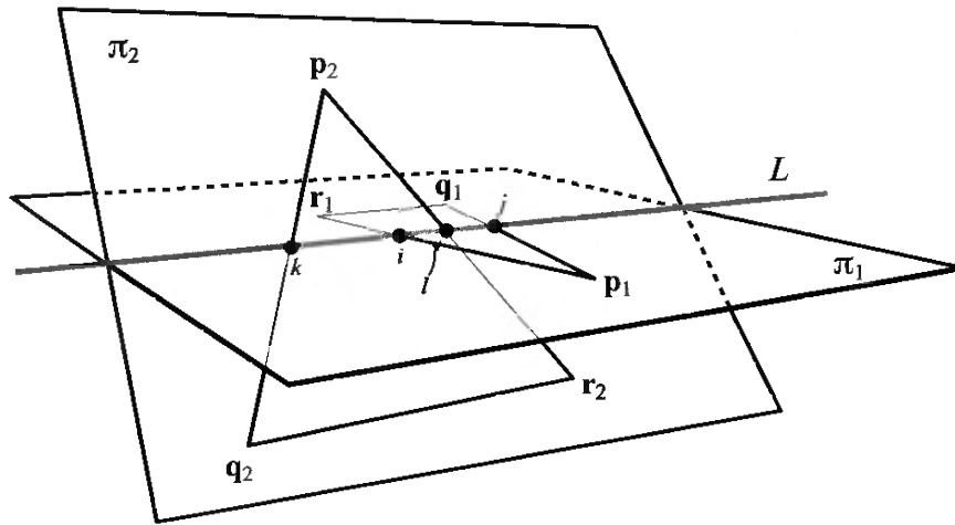
Figure 16.17. Two intersecting triangles with their intersection shown on the line of intersection, L . The intervals on L are also shown and are represented by i , j , k , and l .
