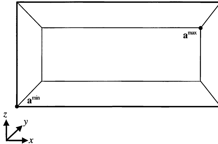
Figure 16.2. A three-dimensional AABB, A , with its extreme points, \mathbf{a}^{\min} and \mathbf{a}^{\max} , and the axes of the standard basis.
