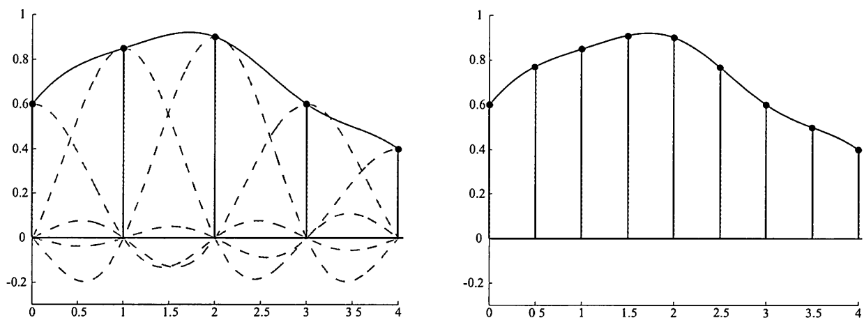
Figure 5.26. On the left is the sampled signal, and the reconstructed signal. On the right, the reconstructed signal has been resampled at double the sample rate, that is, magnification has taken place.
