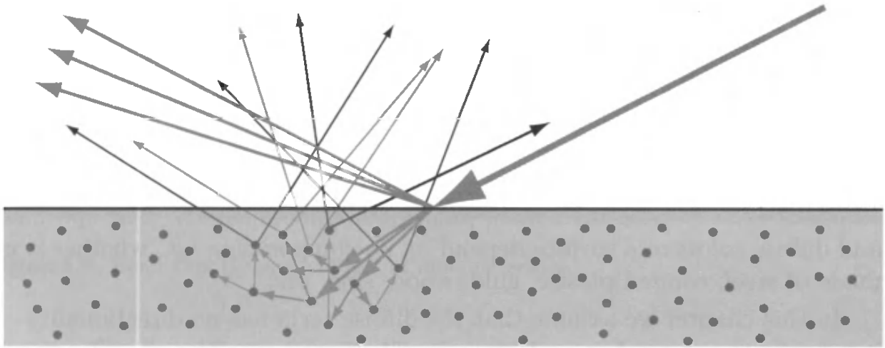
Figure 5.7. Interactions with reflected and transmitted light.
