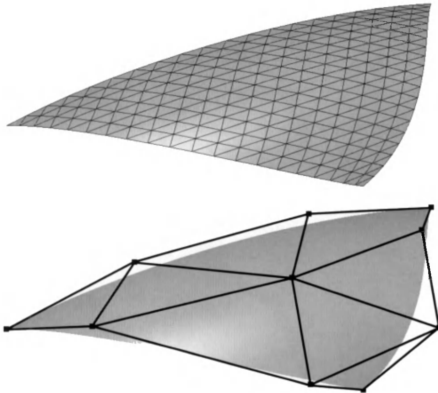
Figure 13.20. Top: wireframe of a Bézier triangle. Bottom: shaded surface together with control points.
