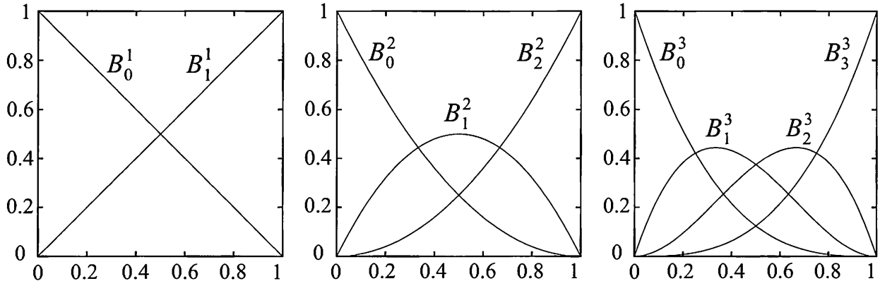
Figure 13.6. Bernstein polynomials for n = 1 , n = 2 , and n = 3 (left to right). The left figure shows linear interpolation, the middle quadratic interpolation, and the right cubic interpolation. These are the blending functions used in the Bernstein form of Bézier curves. So, to evaluate a quadratic curve (middle diagram) at a certain t -value, just find the t -value on the x -axis, and then go vertically until the three curves are encountered, which gives the weights for the three control points. Note that B_i^n(t) \geq 0 , when t \in [0, 1] , and the symmetry of these blending functions: B_i^n(t) = B_{n-i}^n(1-t) .
