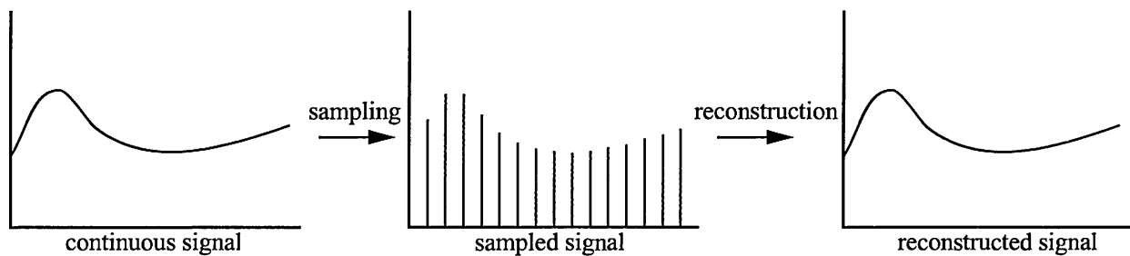
Figure 5.19. A continuous signal (left) is sampled (middle), and then the original signal is recovered by reconstruction (right).
