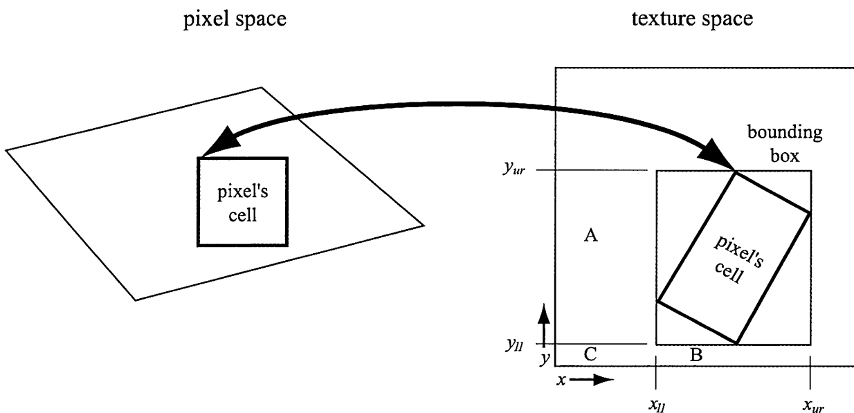
Figure 6.16. The pixel cell is back-projected onto the texture, bound by a rectangle; the four corners of the rectangle are used to access the summed-area table.
