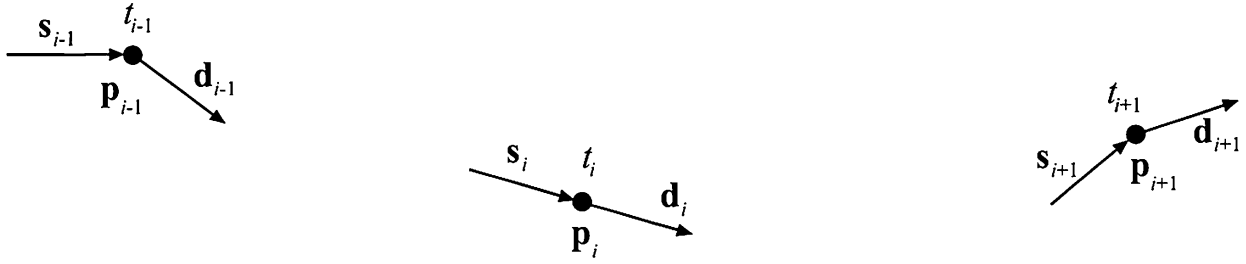
Figure 13.13. Incoming and outgoing tangents for Kochanek-Bartels curves. At each control point \mathbf{p}_i , its time t_i is also shown, where t_i > t_{i-1} , for all i .
