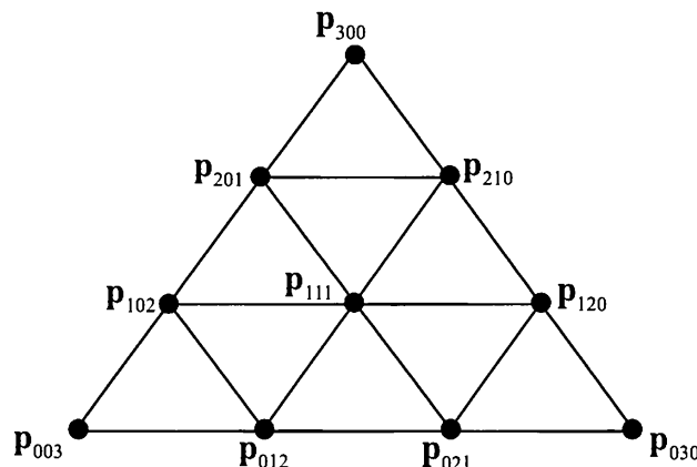
Figure 13.19. The control points of a Bézier triangle with degree three (cubic).
