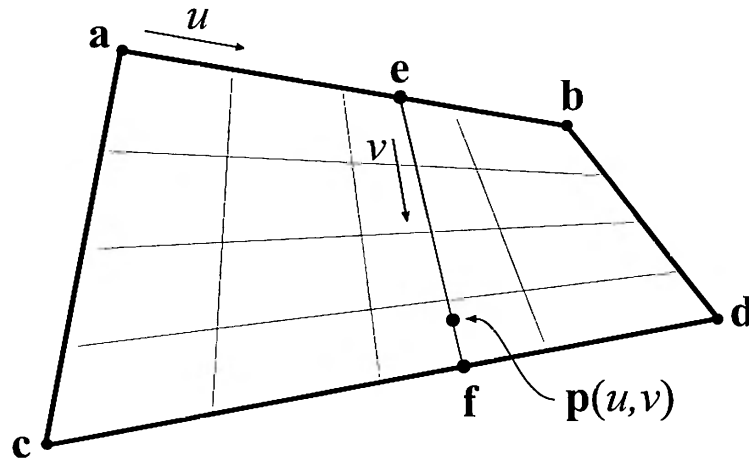
Figure 13.14. Bilinear interpolation using four points.
