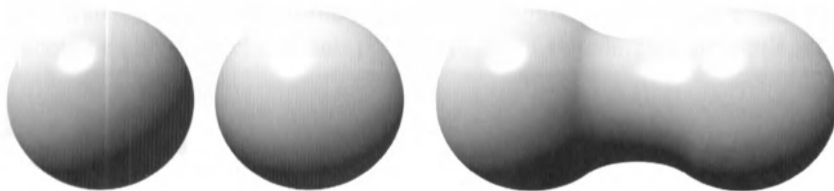
Figure 13.28. The two spheres on the left are blended together into the shape on the right.
