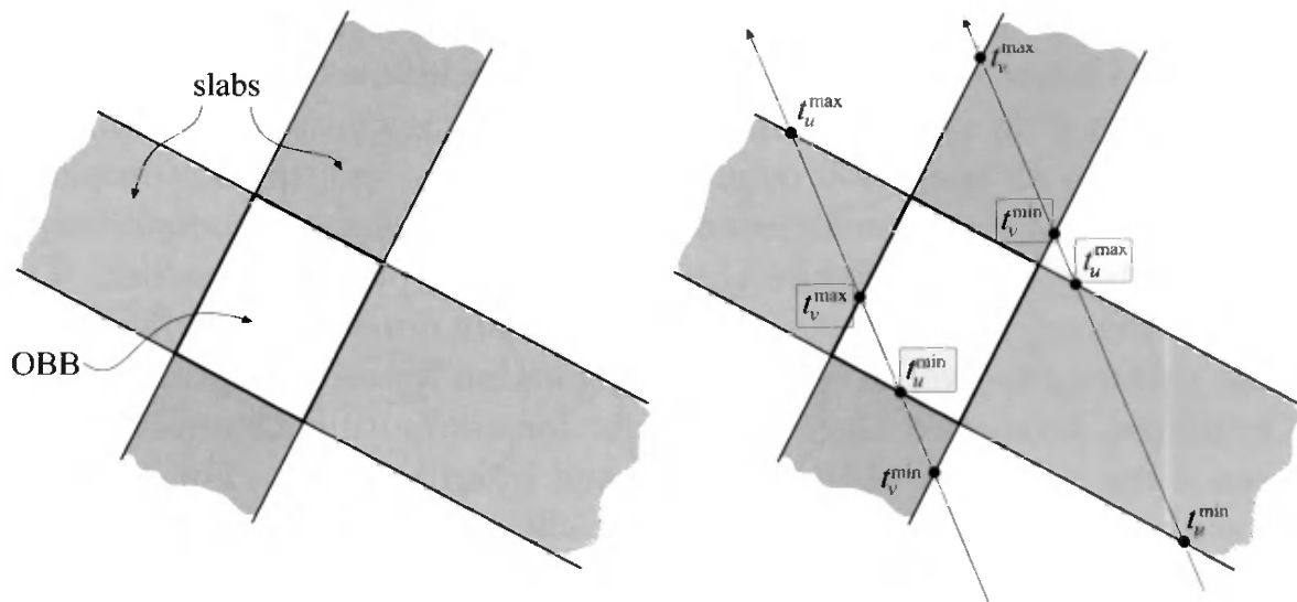
Figure 16.7. The left figure shows a two-dimensional OBB ( oriented bounding box ) formed by two slabs, while the right shows two rays that are tested for intersection with the OBB. All t -values are shown, and they are subscripted with u for the green slab and with v for the other. The extreme t -values are marked with boxes. The left ray hits the OBB since t^{\min} < t^{\max} , and the right ray misses since t^{\max} < t^{\min} .
