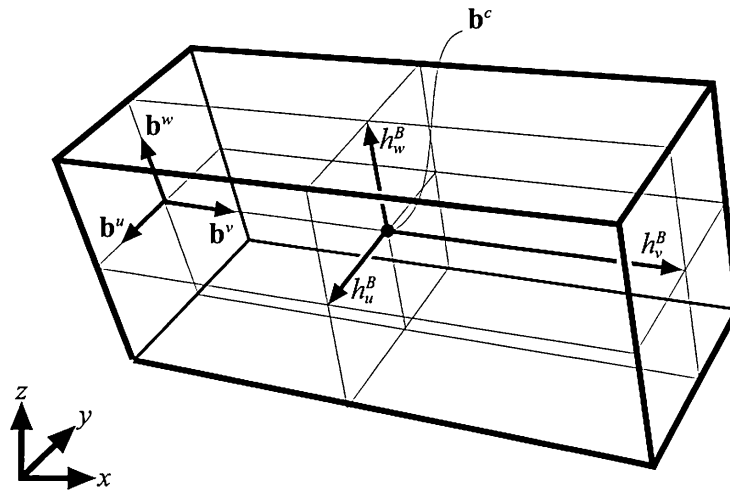
Figure 16.3. A three-dimensional OBB, B , with its center point, \mathbf{b}^c , and its normalized, positively oriented side vectors, \mathbf{b}^u , \mathbf{b}^v , and \mathbf{b}^w . The half-lengths of the sides, h_u^B , h_v^B , and h_w^B , are the distances from the center of the box to the center of the faces, as shown.
