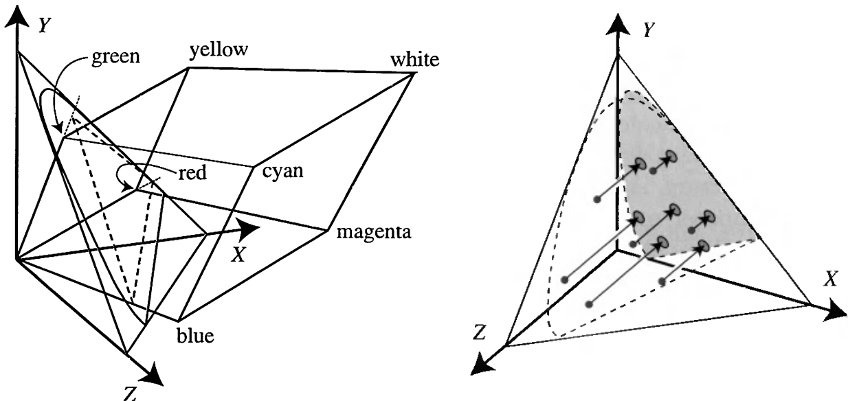
Figure 7.10. On the left, the RGB color cube is shown in XYZ space, along with its gamut projection (in violet) and chromaticity diagram (in blue) onto the X + Y + Z = 1 plane. Lines radiating from the origin have a constant chromaticity value, varying only in luminance. On the right, seven points on the plane X + Y + Z = 1 , and so in xyz coordinates, are projected onto the XY plane (by dropping the z value). The chromaticity diagram outline is shown for both planes, with the resulting diagram shown in gray.
