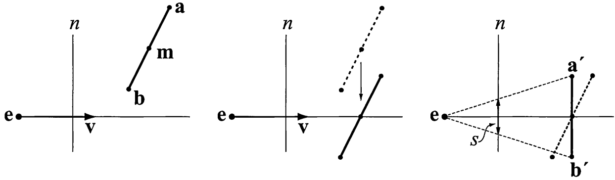
Figure 13.61. Estimation of the screen-space projection, s , of the line segment.
