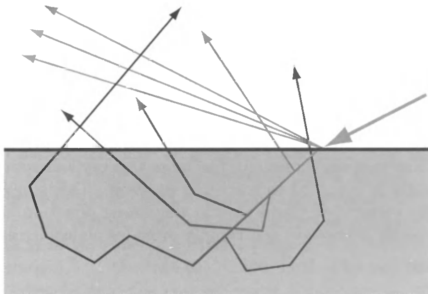
Figure 9.54. Light scattering through an object. Initially the light transmitted into the object travels in the refraction direction, but scattering causes it to change direction repeatedly until it leaves the material. The length of the path through the material determines the percentage of light lost to absorption.
