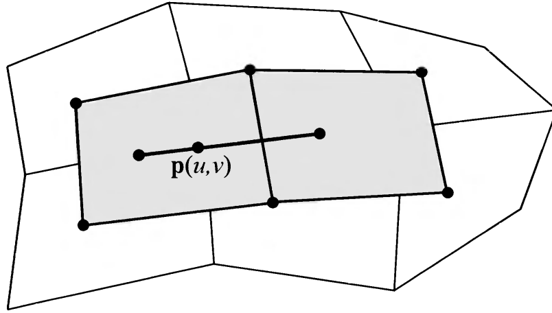
Figure 13.16. Different degrees in different directions.
