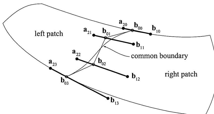
Figure 13.25. How to stitch together two Bézier patches with C^1 continuity. All control points on bold lines must be collinear, and they must have the same ratio between the two segment lengths. Note that \mathbf{a}_{3j} = \mathbf{b}_{0j} to get a shared boundary between patches. This can also be seen to the right in Figure 13.26.
