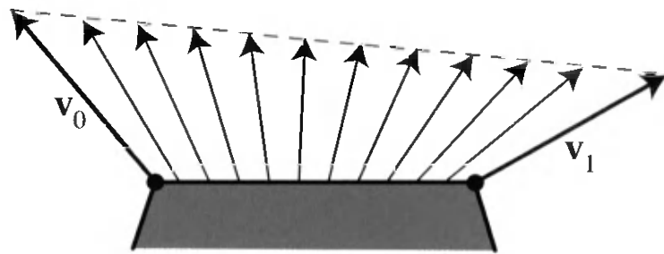
Figure 5.16. Linear interpolation of unit normals at vertices across a surface gives interpolated vectors that are less than a length of one.
