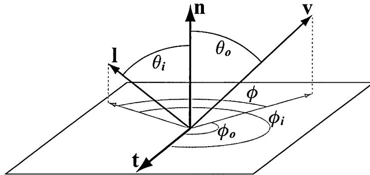
Figure 7.15. The BRDF. Azimuth angles \phi_i and \phi_o are given with respect to a given tangent vector \mathbf{t} . The relative azimuth angle \phi (used for isotropic BRDFs instead of \phi_i and \phi_o ) does not require a reference tangent vector.
