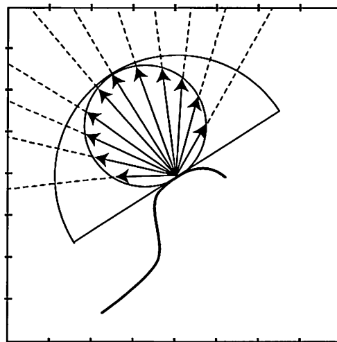
Figure 8.21. Computing an irradiance environment map. The cosine weighted hemisphere around the surface normal is sampled from the environment texture (a cube map in this case) and summed to obtain the irradiance, which is view-independent. The green square represents a cross section of the cube map, and the red tick marks denote the boundaries between texels. Although a cube map representation is shown, any environment representation can be used.
