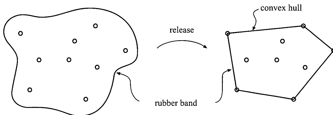
Figure A.6. The rubberband/nail scheme in action. The left figure shows the rubber band before it has been released and the right figure shows the result after. Then the rubber band is a representation of the convex hull of the nails.
