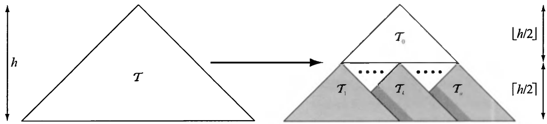
Figure 14.7. The van Emde Boas layout of a tree, T , is created by splitting the height, h , of the tree in two. This creates the subtrees, T_0, T_1, \dots, T_n , and each subtree is split recursively in the same manner until only one node per subtree remains.
