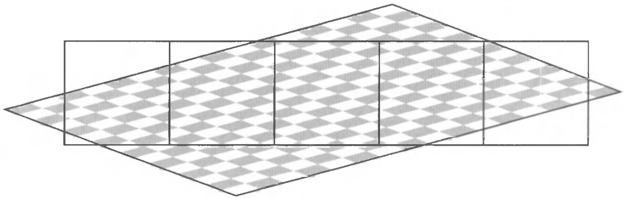
Figure 6.12. Minification: A view of a checkerboard-textured polygon through a row of pixel cells, showing roughly how a number of texels affect each pixel.
