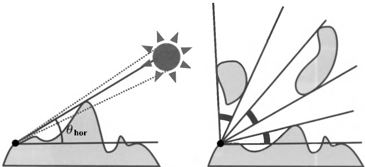
Figure 9.67. On the left: The horizon angle in the direction of an area light source is shown in relation to the upper and lower extents of the light source. These values can be used to generate a partial occlusion value for soft shadowing. On the right: Storing a sequence of occluded angle intervals, instead of a single horizon angle, enables modeling non-heightfield geometry.
