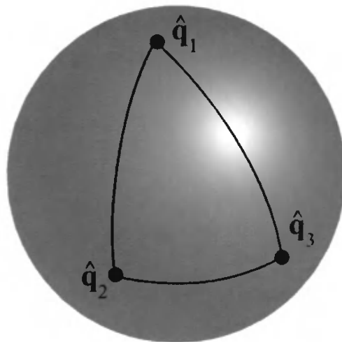
Figure 4.9. Unit quaternions are represented as points on the unit sphere. The function slerp is used to interpolate between the quaternions, and the interpolated path is a great arc on the sphere. Note that interpolating from \hat{q}_1 to \hat{q}_2 and interpolating from \hat{q}_1 to \hat{q}_3 to \hat{q}_2 are not the same thing, even though they arrive at the same orientation.
