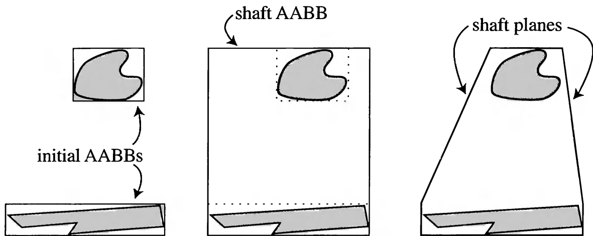
Figure 16.27. Two initial AABBs define a shaft. First, the shaft's AABB is formed to enclose these two AABBs. Then, planes are added to the shaft's definition to chop off volumes of space that are not between the initial AABBs.
