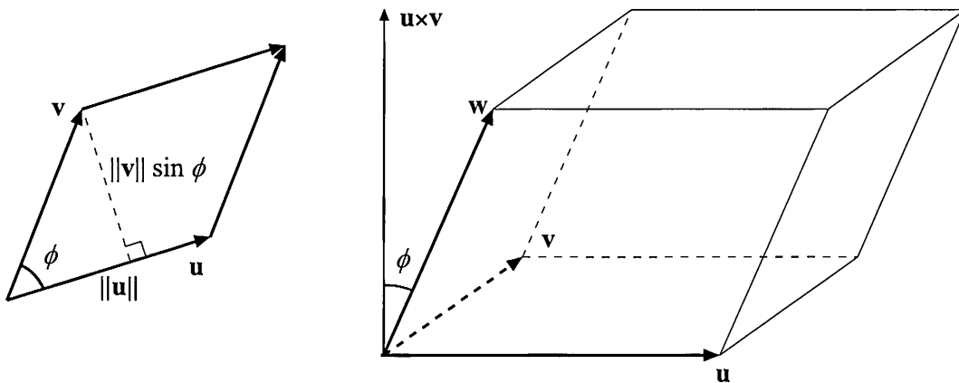
Figure A.7. Left figure: a parallelogram whose area is computed by multiplying the length of the base ( \|\mathbf{u}\| ) with the height ( \|\mathbf{v}\| \sin \phi ). Right figure: the volume of a parallelepiped is given by (\mathbf{u} \times \mathbf{v}) \cdot \mathbf{w} .
