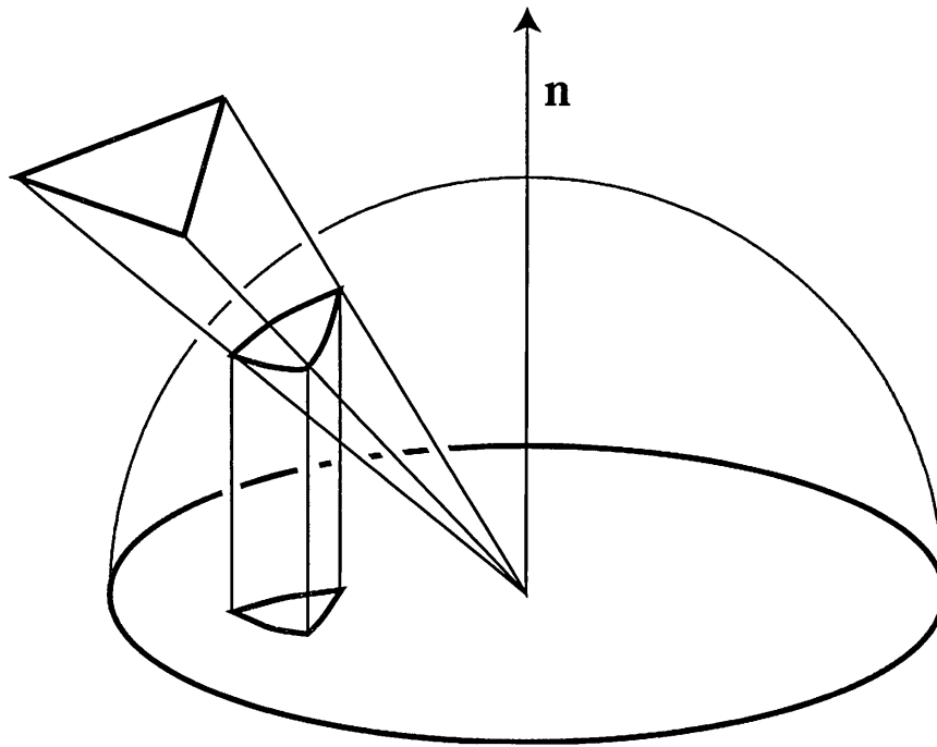
Figure 9.59. For a given receiving point, a patch is projected onto the hemisphere, then onto the ground plane to compute the form factor between the two.
