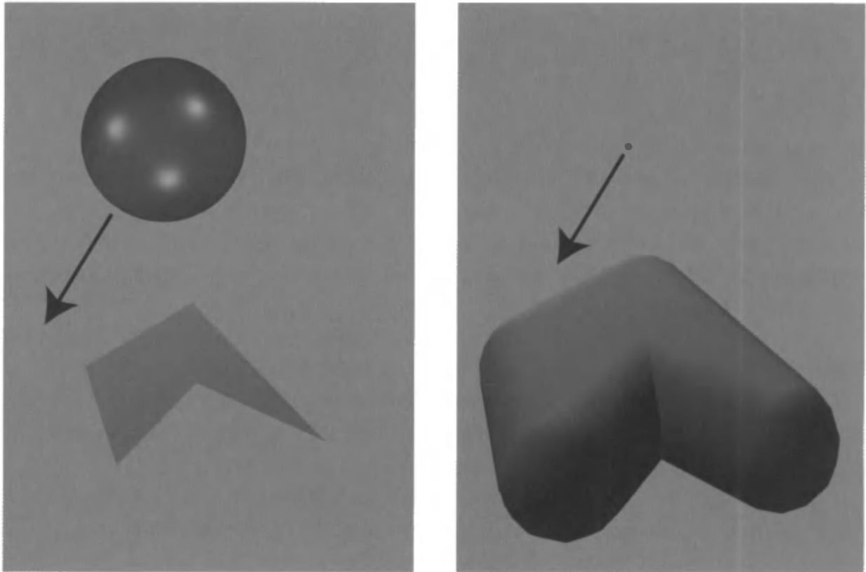
Figure 16.31. In the left figure, a sphere moves towards a polygon. In the right figure, a ray shoots at an “inflated” version of the polygon. The two intersection tests are equivalent.
