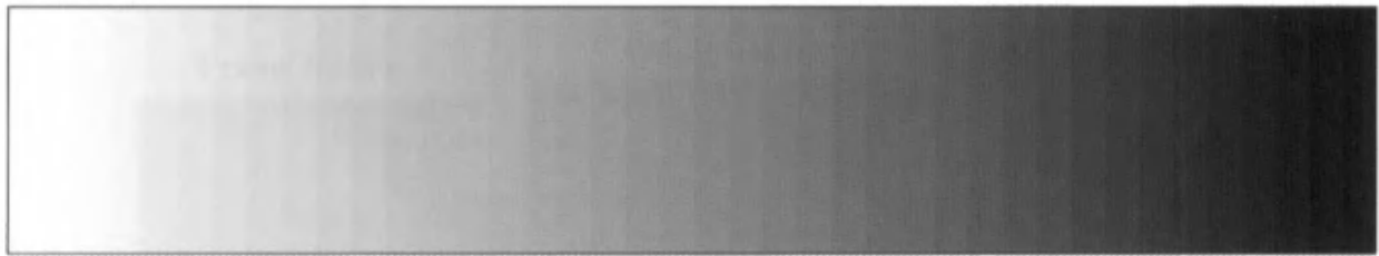
Figure 18.3. As the rectangle is shaded from white to black, banding appears. Although each grayscale bar has a solid intensity level, each can appear to be darker on the left and lighter on the right due to Mach banding.
