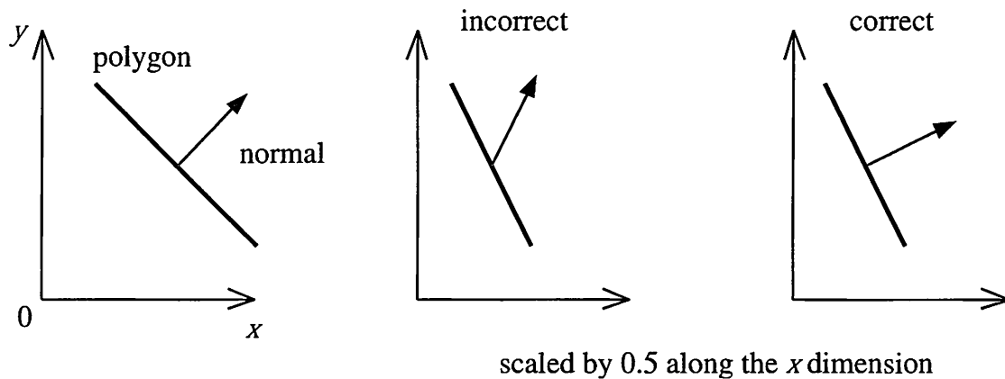
Figure 4.5. On the left is the original geometry, a polygon and its normal shown from the side. The middle illustration shows what happens if the model is scaled along the x -axis by 0.5 and the normal uses the same matrix. The right figure shows the proper transform of the normal.
