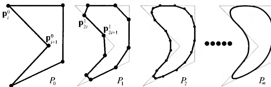
Figure 13.29. Chaikin's subdivision scheme in action. The initial polygon P_0 is subdivided once into P_1 , and then again into P_2 . As can be seen, the corners of each polygon, P_i , are cut off during subdivision. After infinitely many subdivisions, the limit curve P_\infty is obtained. This is an approximating scheme as the curve does not go through the initial points.
