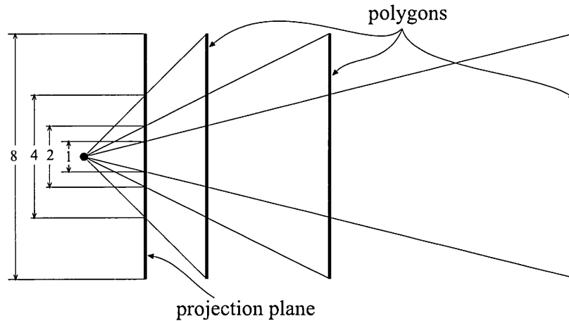
Figure 14.27. This illustration shows how the size of the projection of objects is halved when the distance is doubled.
