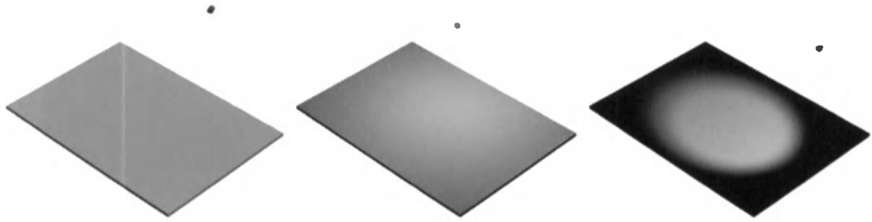
Figure 7.13. Some types of lights: directional, omni with no falloff, and spotlight with a smooth transition.
