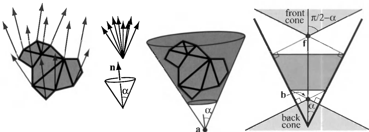
Figure 14.11. Left: a set of polygons and their normals. Middle-left: the normals are collected (top), and a minimal cone (bottom), defined by one normal \mathbf{n} , and a half-angle, \alpha , is constructed. Middle-right: the cone is anchored at a point \mathbf{a} , and truncated so that it also contains all points on the polygons. Right: a cross section of a truncated cone. The light gray region on the top is the frontfacing cone, and the light gray region at the bottom is the backfacing cone. The points \mathbf{f} and \mathbf{b} are respectively the apexes of the front and backfacing cones.
