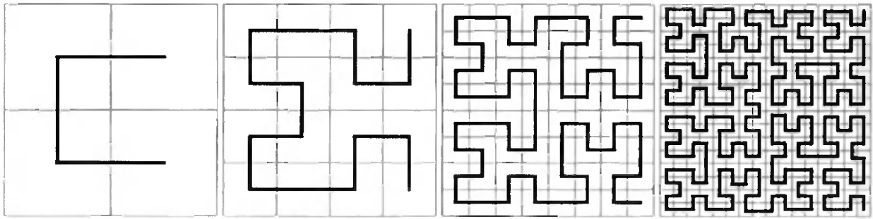
Figure 12.18. An illustration of four generations of Hilbert curves. The thin lines represent the grid, and the bold lines the Hilbert curve. As can be seen, the curve visits every grid cell, and it is self-similar at all scales. A nice property is that the Hilbert curve visits every grid cell within 2 \times 2 cells, then within 4 \times 4 cells, then within 8 \times 8 cells, and so on.
