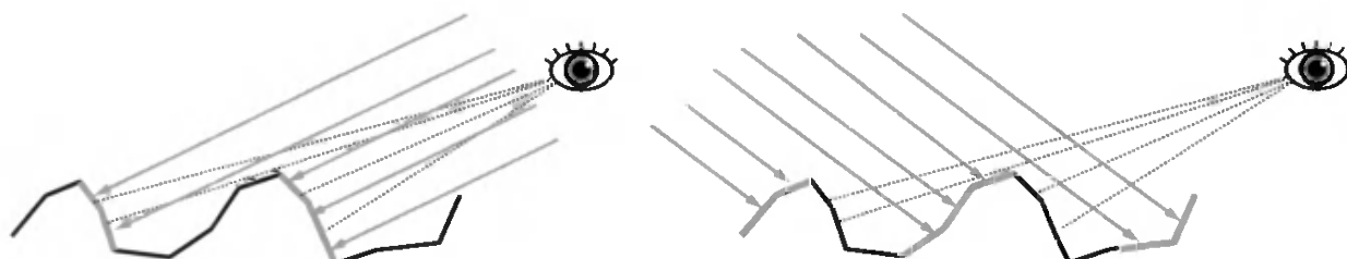
Figure 7.28. Retro-reflection due to microscale roughness. Both sides show a rough surface with low Fresnel reflectance and high scattering albedo (so body reflectance is visually important). On the left, the viewing and lighting directions are similar. The parts of the microgeometry that are brightly lit are also the ones that are highly visible, leading to a bright appearance. On the right, the viewing and lighting directions differ greatly. In this case, the brightly lit areas are occluded from view and the visible areas are shadowed. This leads to a darker appearance.
