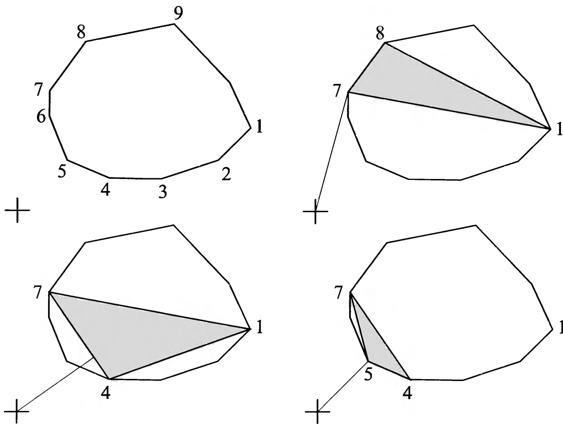
Figure 17.16. Upper left: The minimum distance between the origin and the polygon is to be computed. Upper right: An arbitrary triangle is chosen as a starting point for the algorithm, and the minimum distance to that triangle is computed. Vertex 7 is closest. Lower left: In the next step, all vertices are projected onto the line from the origin to vertex 7, and the closest vertex replaces the one in the triangle that is farthest away on this projection. Thus vertex 4 replaces vertex 8. The closest point on this triangle is then found, which is located on the edge from vertex 4 to 7. Lower right: The vertices are projected onto the line from the origin to the closest point from the previous step, and vertex 5 thus replaces vertex 1, which is farthest away on the projection. Vertex 5 is the closest point on this triangle, and when the vertices are projected on the line to vertex 5, we find that vertex 5 is the closest point overall. This completes the iteration. At this time the closest point on the triangle is found, which also happens to be vertex 5. This point is returned. (Illustration after Jiménez et al. [611].)
