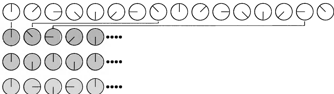
Figure 5.20. The top row shows a spinning wheel (original signal). This is inadequately sampled in second row, making it appear to move in the opposite direction. This is an example of aliasing due to a too low sampling rate. In the third row, the sampling rate is exactly two samples per revolution, and we cannot determine in which direction the wheel is spinning. This is the Nyquist limit. In the fourth row, the sampling rate is higher than two samples per revolution, and we suddenly can see that the wheel spins in the right direction.
