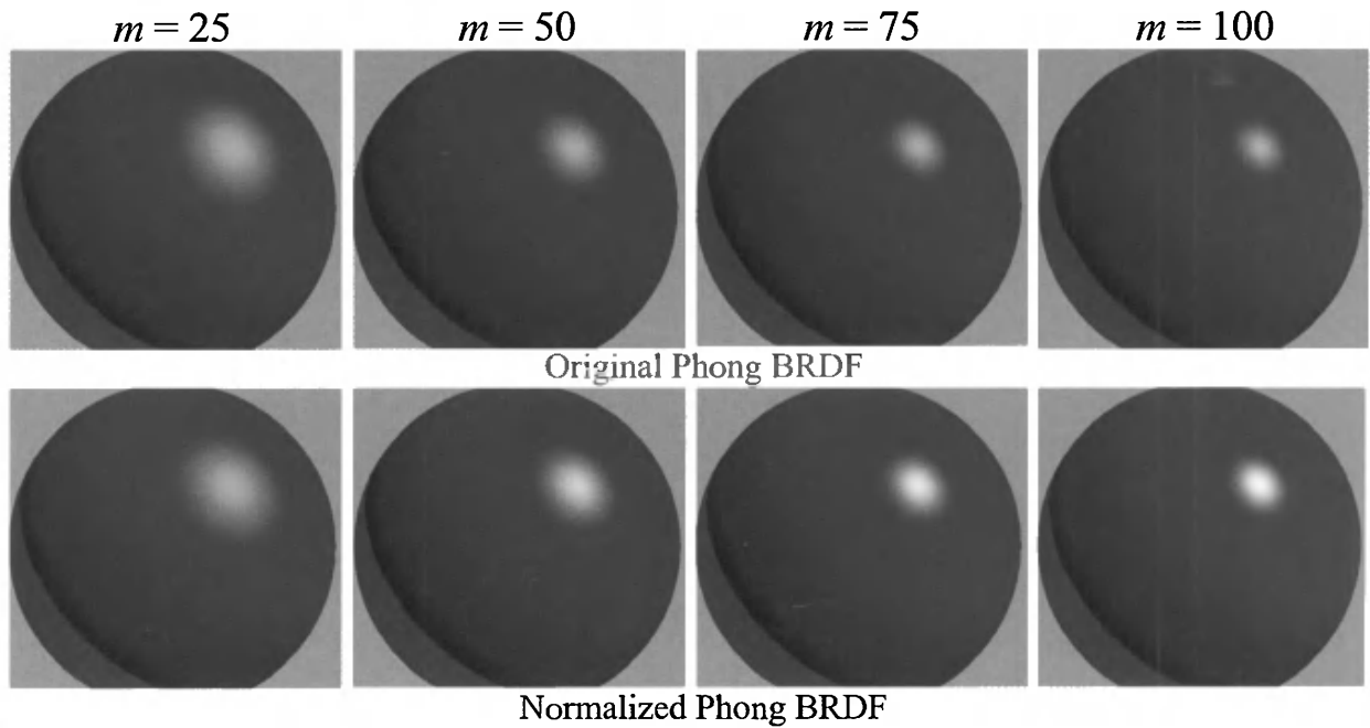
Figure 7.38. Rendered images of a red plastic sphere. The bottom row of images was rendered with the normalized Phong BRDF, using c_{\text{spec}} = 0.05 (an appropriate value for plastic). The value of c_{\text{diff}} was set to [0.95, 0, 0] , for maximum saturation and brightness without violating energy conservation. The top row of images was rendered with the original (not normalized) Phong BRDF, using values of c_{\text{spec}} and c_{\text{diff}} chosen so that the two leftmost images match. The value of the smoothness parameter m increases from right to left, and the other BRDF parameters are held constant for each row. The intent is to render spheres made of the same substance (red plastic) but of differing surface smoothness. It can be seen that in the bottom row, the highlight grows much brighter as it gets narrower, which is the correct behavior—the outgoing light is concentrated in a narrower cone, so it is brighter. In the top row, the highlight remains equally bright as it gets narrower, so there is a loss of energy and the surface appears to be getting less reflective.
