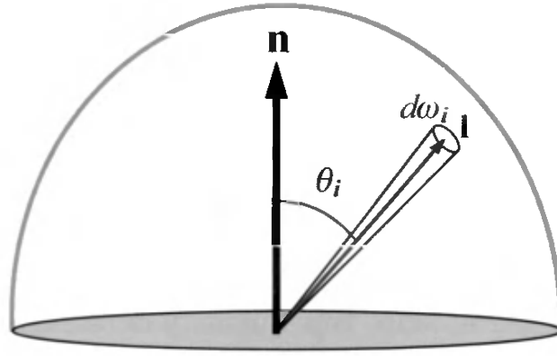
Figure 8.2. A surface point illuminated from all directions on the hemisphere. An example light direction \mathbf{l} and an infinitesimal solid angle d\omega_i around it are shown.
