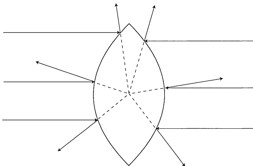
Figure 8.17. Two paraboloid mirrors that capture an environment using diametrically opposite views. The reflected view vectors all extend to meet at the center of the object, the foci of both paraboloids.
