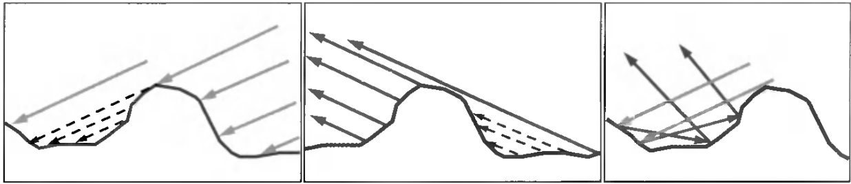
Figure 7.26. Geometrical effects of microscale structure. On the left, the black dashed arrows indicate an area that is shadowed (occluded from the light) by other microgeometry. In the center, the red dashed arrows indicate an area that is masked (occluded from view) by other microgeometry. On the right, interreflection of light between the microscale structures is shown.
