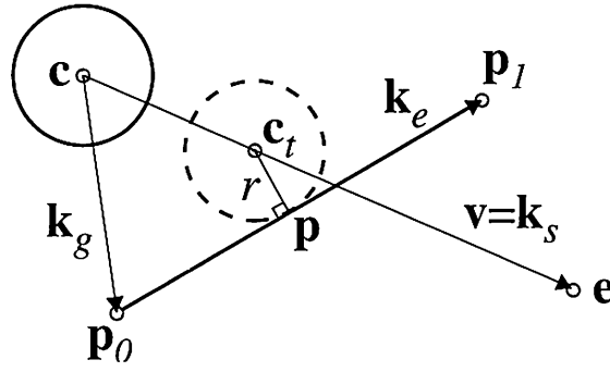
Figure 16.30. Notation for the intersection test of a moving sphere and a polygon edge. (After Schroeder [1137].)
