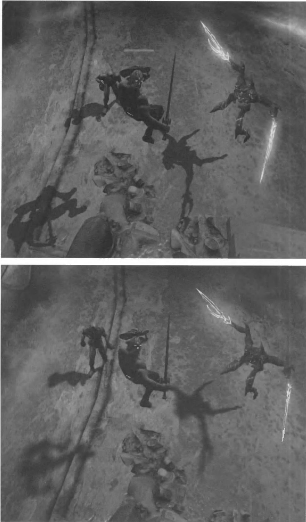
Figure 9.4. The upper image was rendered with hard shadows, while the lower was rendered with soft shadows. The soft shadow has a smaller umbra region (i.e., area fully in shadow), and the softness increases with the distance from the receiving point (the ground) [916]. (Images from “ Hellgate: London ” courtesy of Flagship Studios, Inc.)
