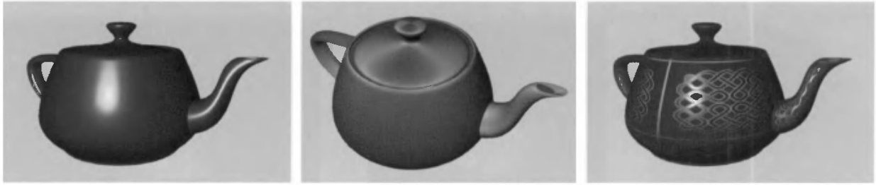
Figure 7.43. Materials rendered using factorization [835], where the BRDF is approximated by pairs of two-dimensional textures. From left to right, the materials are a blue Krylon latex enamel, satin, and a textured velvet body with garnet red paint on the knot shape. The paints and velvet are from measured BRDF data [190, 200], and the satin is computed using the analytic Poulin-Fournier anisotropic reflectance model [1027]. (Images generated by the “brdfview” program by McCool, Ang, and Ahmad.)
