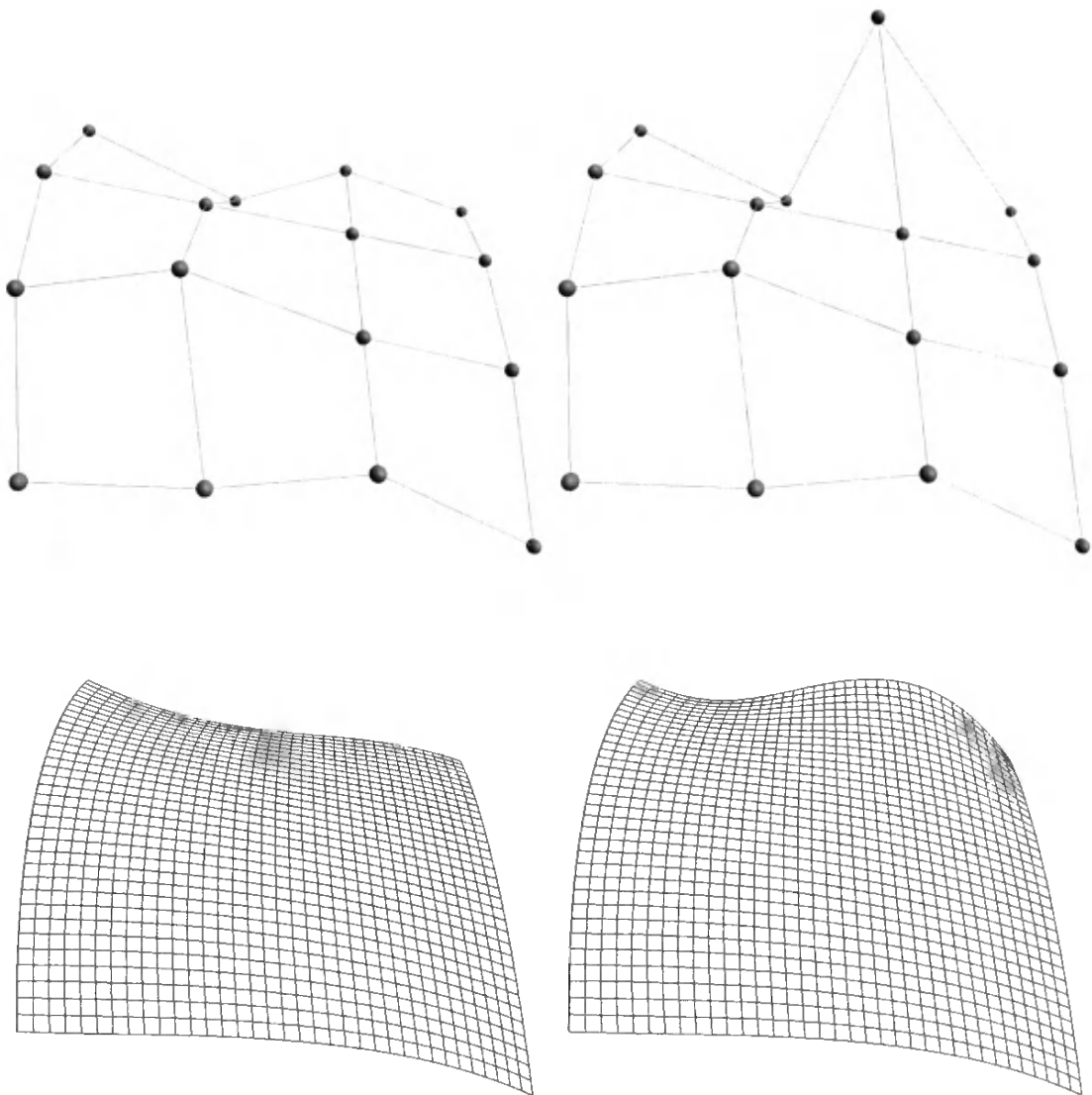
Figure 13.18. This set of images shows what happens to a Bézier patch when one vertex is moved. Most of the change is near the moved control point.
