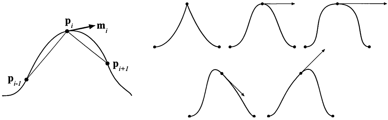
Figure 13.12. One method of computing the tangents is to use a combination of the chords (left). The upper row at the right shows three curves with different tension parameters ( a ). The left curve has a \approx 1 , which means high tension; the middle curve has a \approx 0 , which is default tension; and the right curve has a \approx -1 , which is low tension. The bottom row of two curves at the right shows different bias parameters. The curve on the left has a negative bias, and the right curve has a positive bias.
