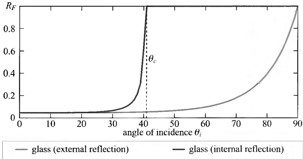
Figure 7.22. Comparison of internal and external reflectance curves at a glass-air interface.
