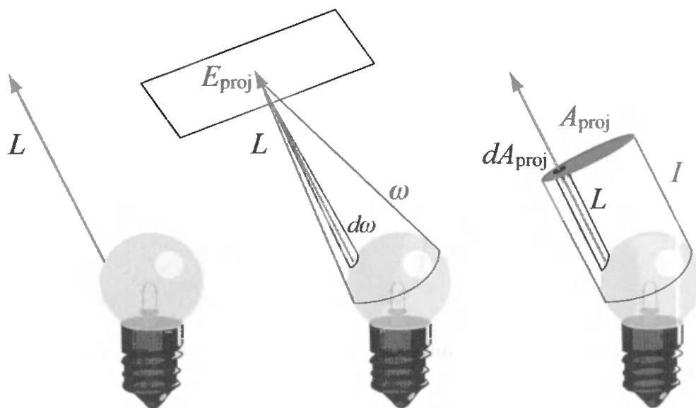
Figure 7.5. Radiance, radiance computed from irradiance, and radiance from intensity.
