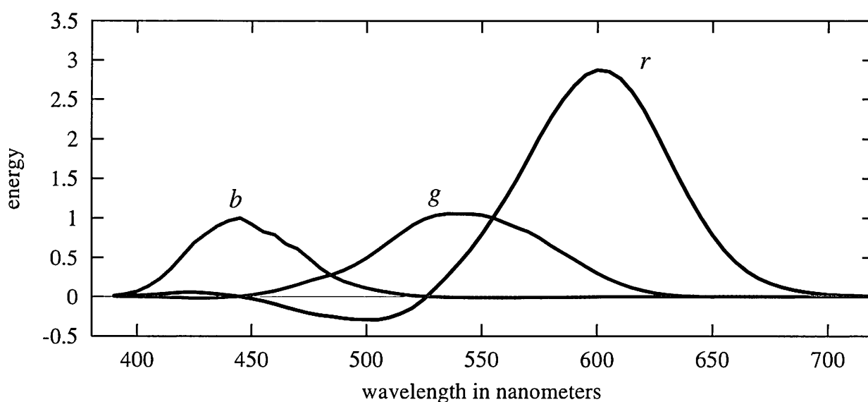
Figure 7.8. The r , g , and b 2-degree color matching curves, from Stiles & Burch (1955). Values are shown in terms of energy, not the [-1, 1] knob range. These color matching curves are not to be confused with the spectral distributions of the light sources used in the color matching experiment.
