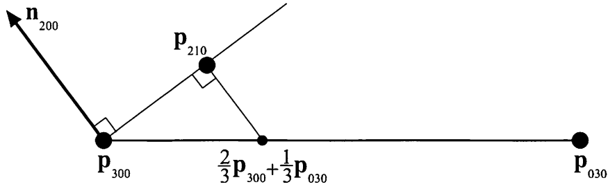
Figure 13.22. How the Bézier point \mathbf{p}_{210} is computed using the normal \mathbf{n}_{200} at \mathbf{p}_{300} , and the two corner points \mathbf{p}_{300} and \mathbf{p}_{030} .
