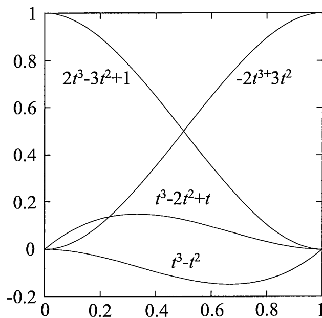
Figure 13.10. Blending functions for Hermite cubic interpolation. Note the asymmetry of the blending functions for the tangents. Negating the blending function t^3 - t^2 and \mathbf{m}_1 in Equation 13.17 would give a symmetrical look.
