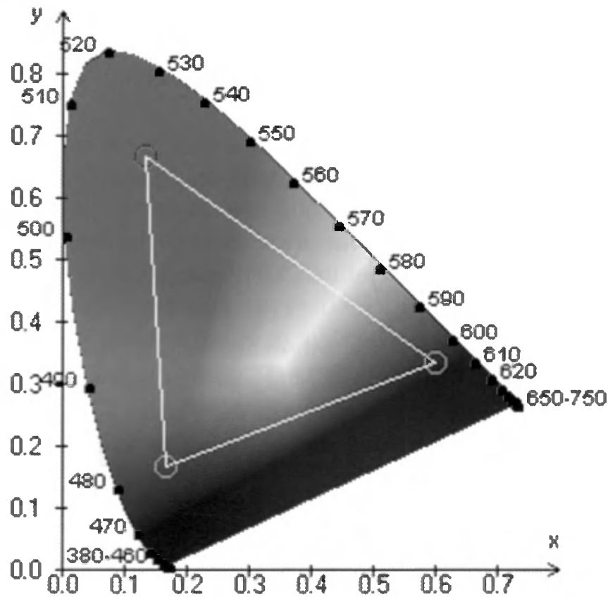
Figure 7.11. The chromaticity diagram. The curve is labeled with the corresponding pure wavelength colors, and a typical gamut is shown with the triangle. (Image generated by a Java applet from the Computer Science Department, Rochester Institute of Technology.)
