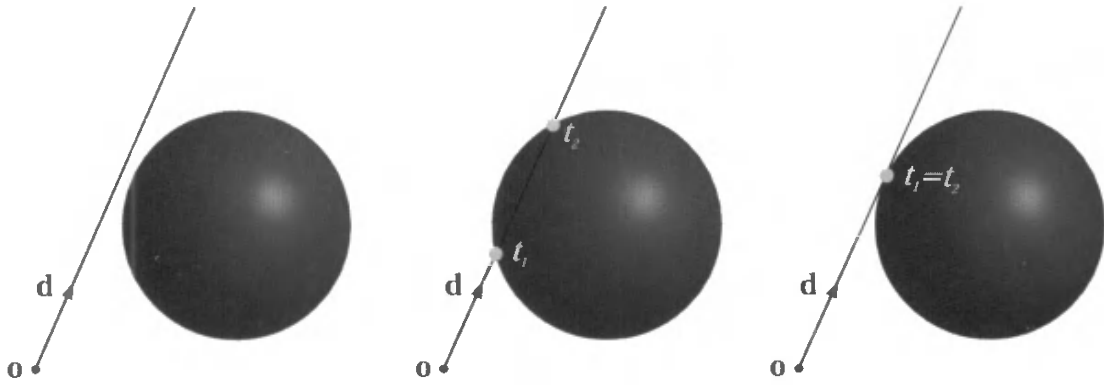
Figure 16.5. The left image shows a ray that misses a sphere and consequently b^2 - c < 0 . The middle image shows a ray that intersects a sphere at two points ( b^2 - c > 0 ) determined by the scalars t_1 and t_2 . The right image illustrates the case where b^2 - c = 0 , which means that the two intersection points coincide.
