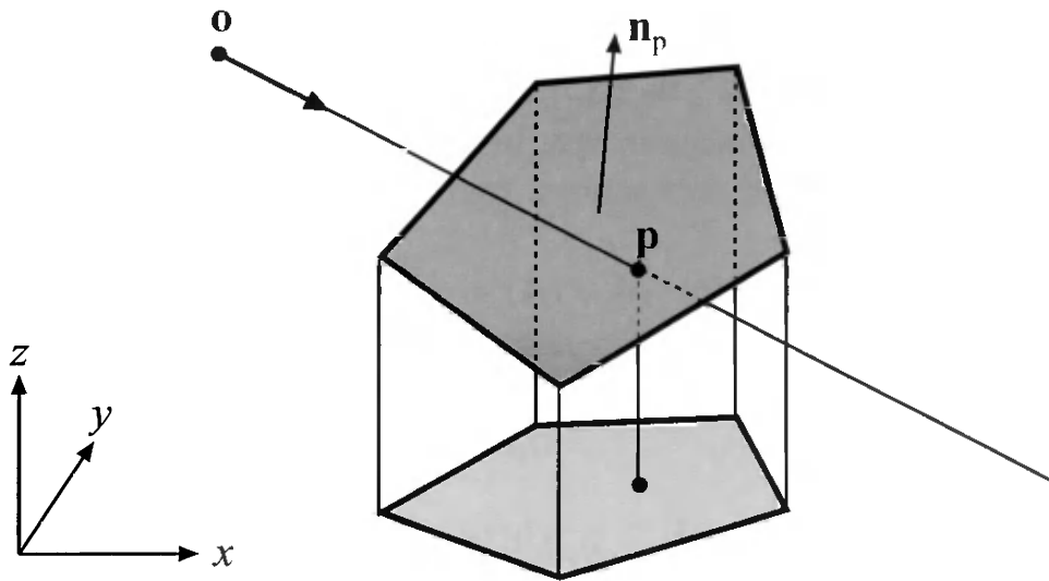
Figure 16.11. Orthographic projection of polygon vertices and intersection point p onto the xy -plane, where the area of the projected polygon is maximized. This is an example of using dimension reduction to obtain simpler calculations.
