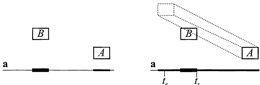
Figure 16.32. Left: the stationary SAT illustrated for an axis \mathbf{a} . A and B do not overlap on this axis. Right: the dynamic SAT illustrated. A moves and the projection of its interval on \mathbf{a} is tracked during the movement. Here, the two objects overlap on axis \mathbf{a} .
