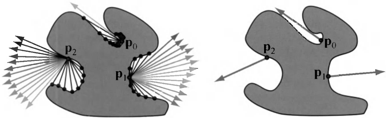
Figure 9.37. An object under ambient illumination. Three points ( p_0 , p_1 , and p_2 ) are shown. On the left, blocked directions are shown as black rays ending in intersection points (black circles). Unblocked directions are shown as arrows, colored according to the cosine factor, so arrows closer to the surface normal are lighter. On the right, each blue arrow shows the average unoccluded direction or bent normal .
