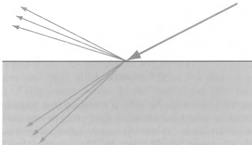
Figure 5.6. Light scattering at a surface—reflection and refraction.
