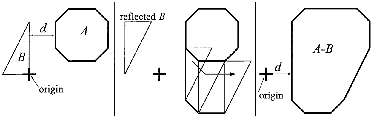
Figure 17.15. To the left, two convex objects A and B are shown. To construct A - B , first move A and B so that one reference point is at the origin (already done at the left). Then B is reflected, as shown in the middle, and the chosen reference point on B is put on the surface of A and then the reflected B is swept around A . This creates A - B , to the right. The minimum distance, d , is shown both on the left and the right.
