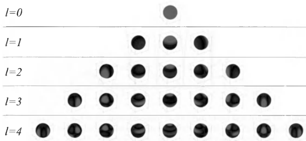
Figure 8.27. The first five frequency bands of spherical harmonics. Each spherical harmonic function has areas of positive values (colored green) and areas of negative values (colored red). ( Spherical harmonic visualizations courtesy of Robin Green. )
