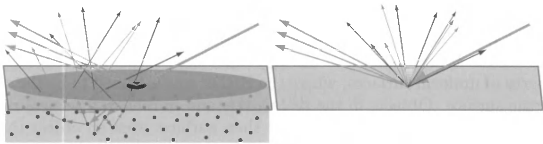
Figure 7.16. Light interacting with a surface. On the left, we see the subsurface interactions causing light to be re-emitted away from the entry point. The red and green circles represent the region covered by a pixel at two different scales of observation. On the right, all subsurface scattered light is shown emitting from the entry point—the details of what happens under the surface are ignored.
