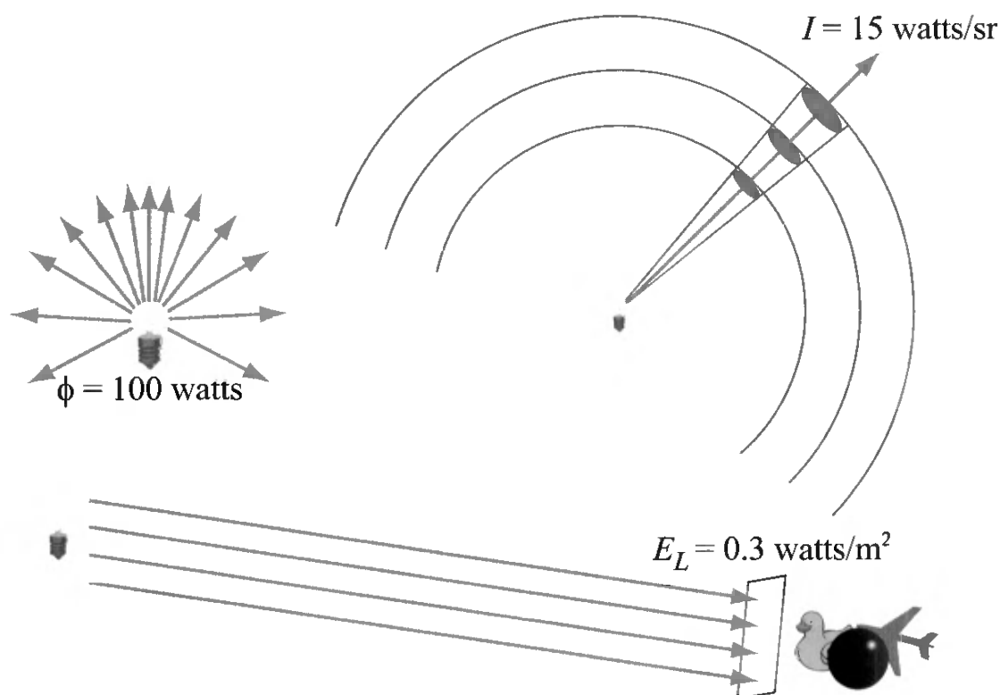
Figure 7.2. A light bulb. In the upper-left part of the figure, the light bulb’s radiant flux of 100 watts is shown. In the lower part of the figure, the light bulb is illuminating a small scene from a distance, so that its irradiance contribution E_L (measured in a plane perpendicular to the light direction) is a constant 0.3 watts per square meter over the scene. In the upper-right part of the figure, the intensity of the light bulb is measured in a given direction as 15 watts per steradian.
