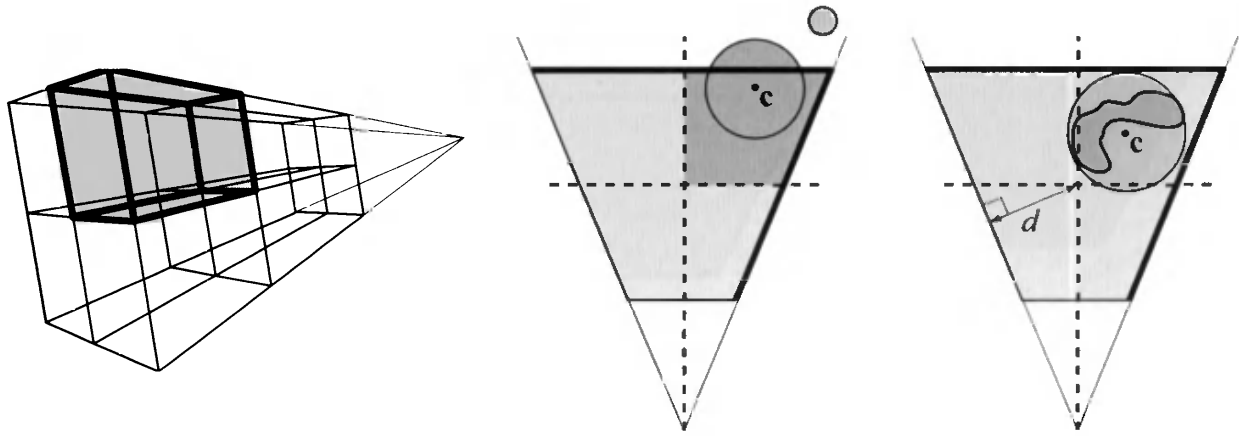
Figure 16.25. The left figure shows how a three-dimensional frustum is divided into eight octants. The other figure shows a two-dimensional example, where the sphere center c is in the upper right octant. The only planes that then need to be considered are the right and the far planes (thick black lines). Note that the small sphere is in the same octant as the large sphere. This technique also works for arbitrary objects, but the following condition must hold: The minimum distance, d , from the frustum center to the frustum planes must be larger than the radius of a tight bounding sphere around the object. If that condition is fulfilled, then the bounding sphere can be used to find the octant.
