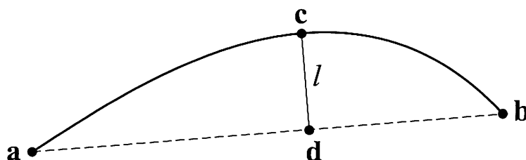
Figure 13.60. The points a and b have already been generated on this surface. The question is: Should a new point, that is c, be generated on the surface?
