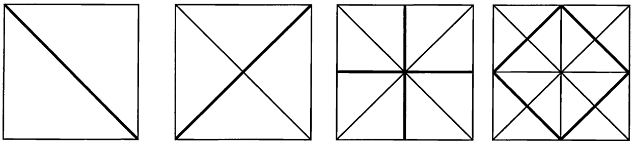
Figure 12.28. The triangle bintree. On the left, the heightfield is represented by two triangles at the topmost level. At each successive level, every triangle is split into two, with splits shown by the thick lines.
