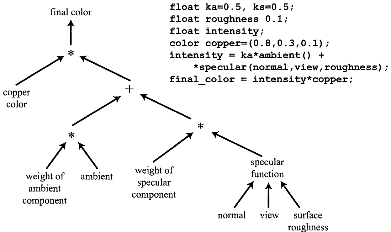
Figure 3.3. Shade tree for a simple copper shader, and its corresponding shader language program. (After Cook [194].)
