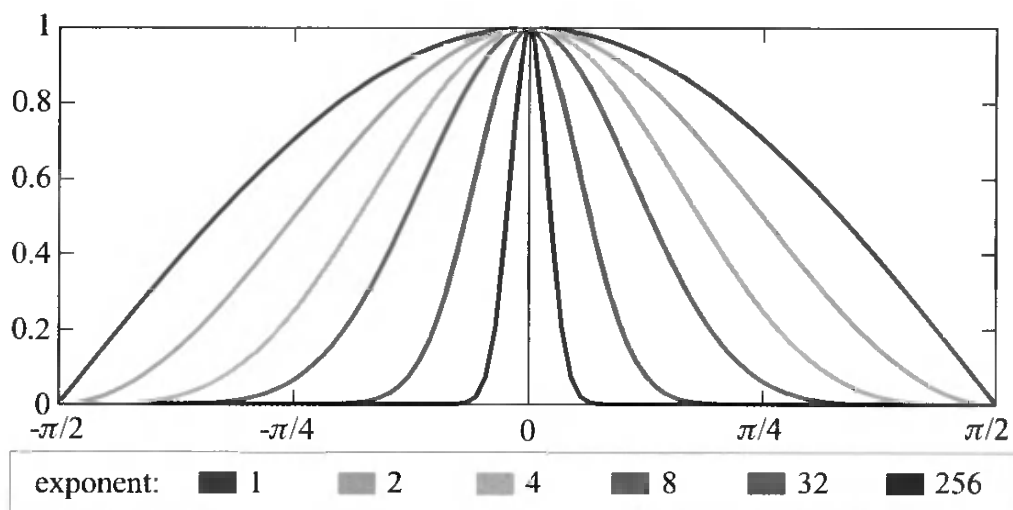
Figure 7.36. Graph of unnormalized cosine power term versus angle for various exponents. Increasing the exponent pulls the curve in, making for a tighter highlight. However, the height of the curve remains unchanged. This causes the total specularly reflected energy to decrease.
