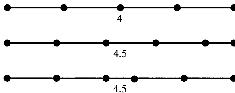
Figure 13.54. Top: integer tessellation. Middle: fractional tessellation, with the fraction to the right. Bottom: fractional tessellation with the fraction in the middle. This configuration avoids cracks between adjacent patches.
