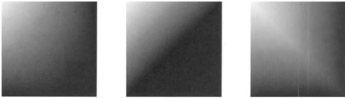
Figure 12.5. The left figure is rendered as a quadrilateral; the middle is two triangles with upper-right and lower-left corners connected; the right shows what happens when the other diagonal is used. The middle figure is better visually than the right one.
