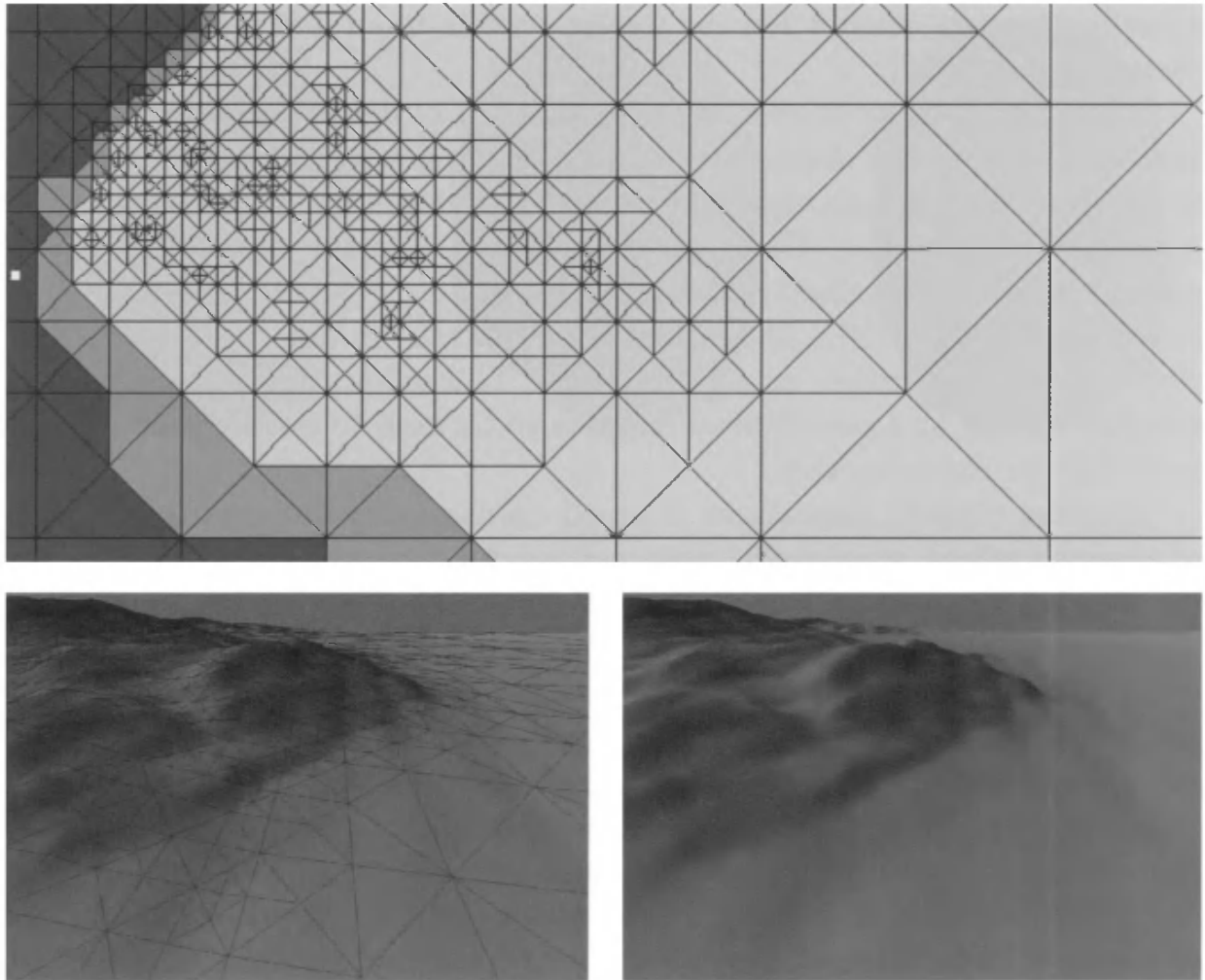
Figure 12.29. A ROAM view-dependent subdivision of the terrain. At top, the yellow dot on the left is the viewer. The blue areas are outside the view frustum, the light green are inside, and the dark green overlap the frustum's edges. (Images courtesy of Mark Duchaineau, LLNL.)
