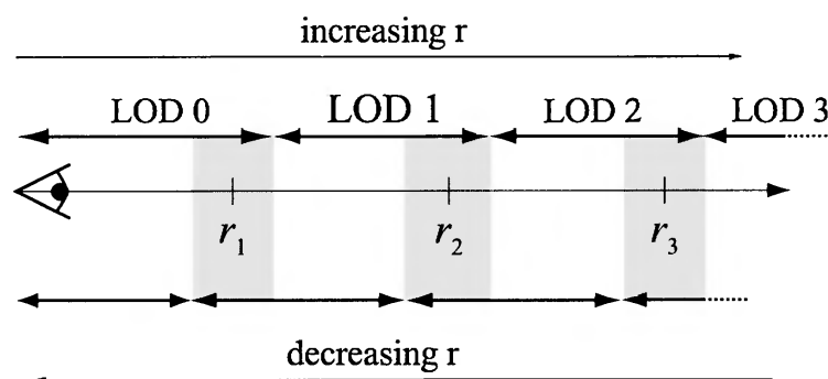
Figure 14.30. The gray areas illustrate the hysteresis regions for the LOD technique.
