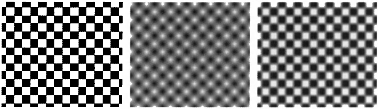
Figure 6.10. Nearest neighbor, bilinear interpolation, and part way in between by remapping, using the same 2 \times 2 checkerboard texture. Note how nearest neighbor sampling gives slightly different square sizes, since the texture and the image grid do not match perfectly.
