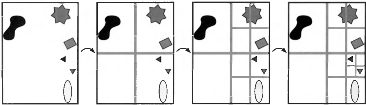
Figure 14.5. The construction of a quadtree. The construction starts from the left by enclosing all objects in a bounding box. Then the boxes are recursively divided into four equal-sized boxes until each box (in this case) is empty or contains one object.
