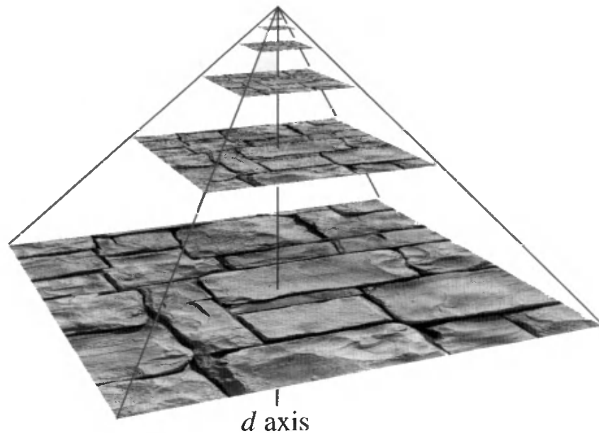
Figure 6.14. A mipmap is formed by taking the original image (level 0), at the base of the pyramid, and averaging each 2 \times 2 area into a texel value on the next level up. The vertical axis is the third texture coordinate, d . In this figure, d is not linear; it is a measure of which two texture levels a sample uses for interpolation.
