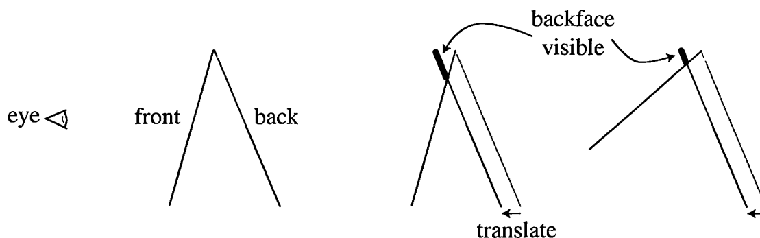
Figure 11.6. The z -bias method of silhouetting, done by translating the backface forward. If the frontface is at a different angle, as shown on the right, a different amount of the backface is visible. ( Illustration after Raskar and Cohen [1046]. )
