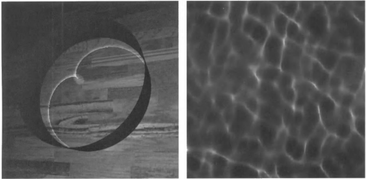
Figure 9.53. The caustic volumes technique can generate various types of caustics, such as those from a metallic ring or from the ocean’s surface [319].
