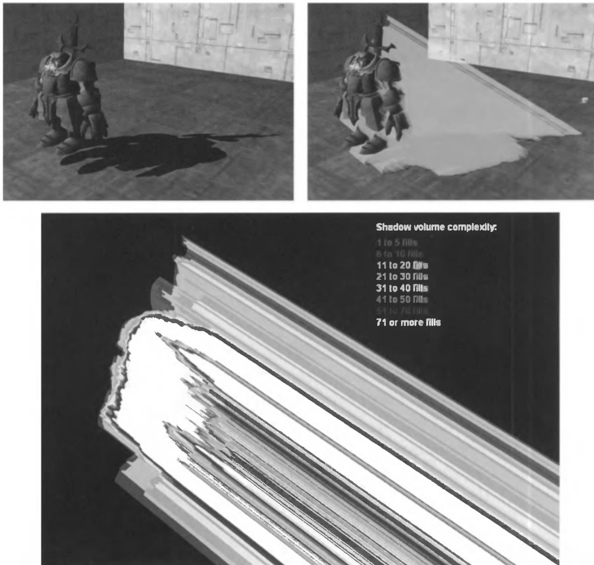
Figure 9.13. Shadow volumes. On the left, a character casts a shadow. On the right, the extruded triangles of the model are shown. Below, the number of times a pixel is drawn from the extruded triangles. (Images from Microsoft SDK [261] sample “ShadowVolume.”)
