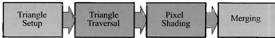
Figure 2.8. The rasterizer stage subdivided into a pipeline of functional stages.
