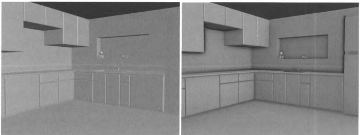
Figure 9.40. The Z-buffer unsharp mask technique for approximate ambient occlusion. The image on the left has no ambient occlusion; the image on the right includes an approximate ambient occlusion term generated with the Z-buffer unsharp mask technique. ( Images courtesy of Mike Pan. )
