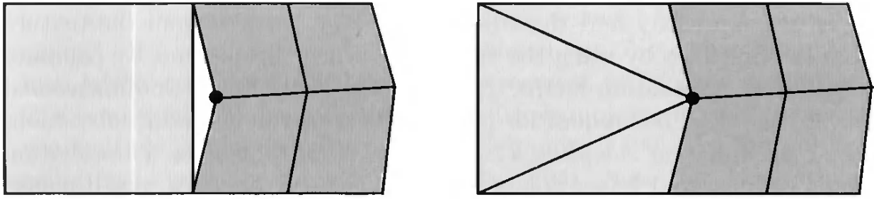
Figure 13.59. To the left, a crack is visible between the two regions. This is because the right has a higher tessellation rate than the left. The problem lies in that the right region has evaluated the surface where there is a black circle, and the left region has not. The standard solution is shown to the right.
