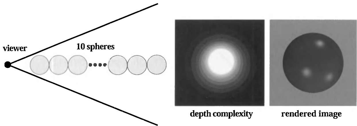
Figure 14.15. An illustration of how occlusion culling can be useful. Ten spheres are placed in a line, and the viewer is looking along this line (left). The depth complexity image in the middle shows that some pixels are written to several times, even though the final image (on the right) only shows one sphere.
