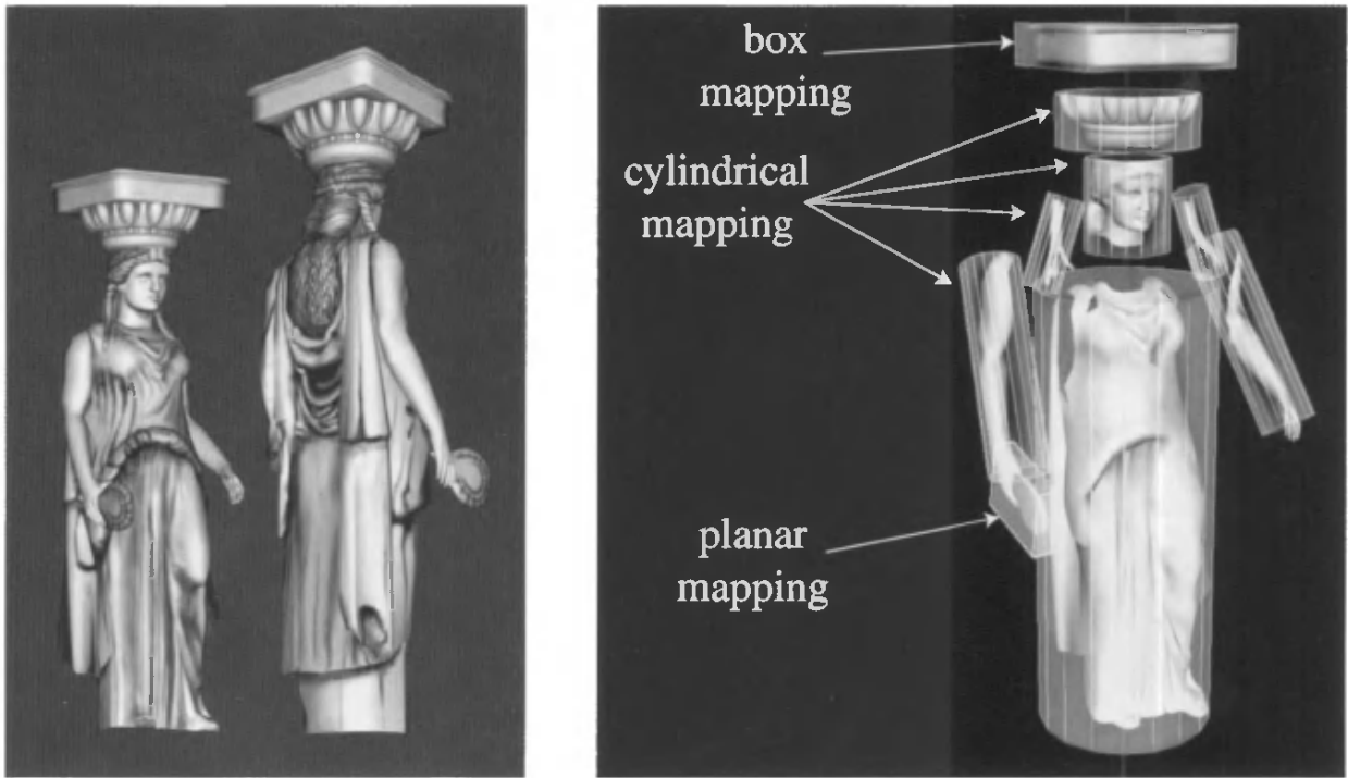
Figure 6.5. How various texture projections are used on a single model. ( Images courtesy of Tito Pagán. )
