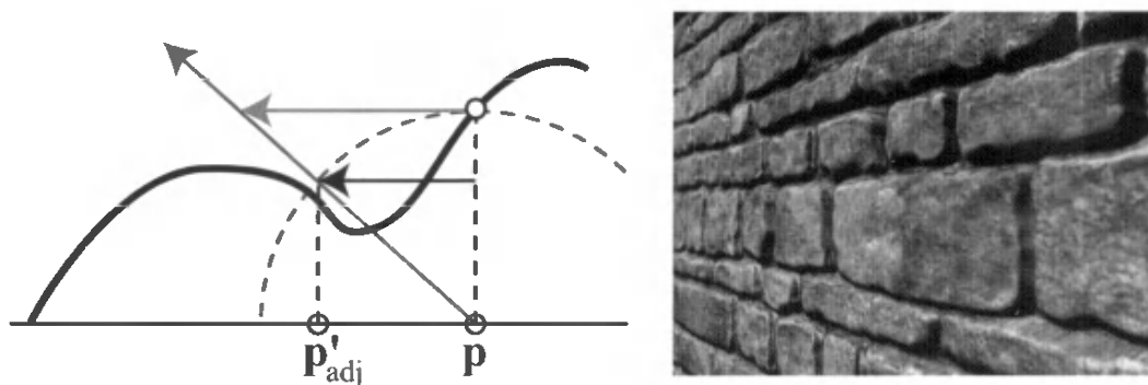
Figure 6.32. In parallax offset limiting, the offset moves at most the amount of the height away from the original location, shown as a dashed circular arc. The gray offset shows the original result, the black the limited result. On the right is a wall rendered with the technique. ( Image courtesy of Terry Welsh. )
