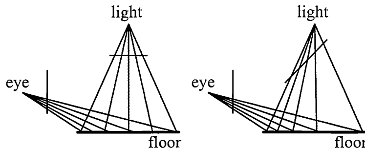
Figure 9.21. For an overhead light, on the left the sampling on the floor does not match the eye's rate. By changing the view direction and projection window, the light's sampling rate is biased toward having a higher density of texels nearer the eye.
