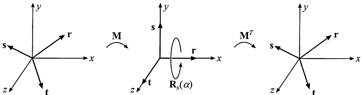
Figure 4.7. Rotation about an arbitrary axis, \mathbf{r} , is accomplished by finding an orthonormal basis formed by \mathbf{r} , \mathbf{s} , and \mathbf{t} . We then align this basis with the standard basis so that \mathbf{r} is aligned with the x -axis. The rotation around the x -axis is performed there, and finally we transform back.
