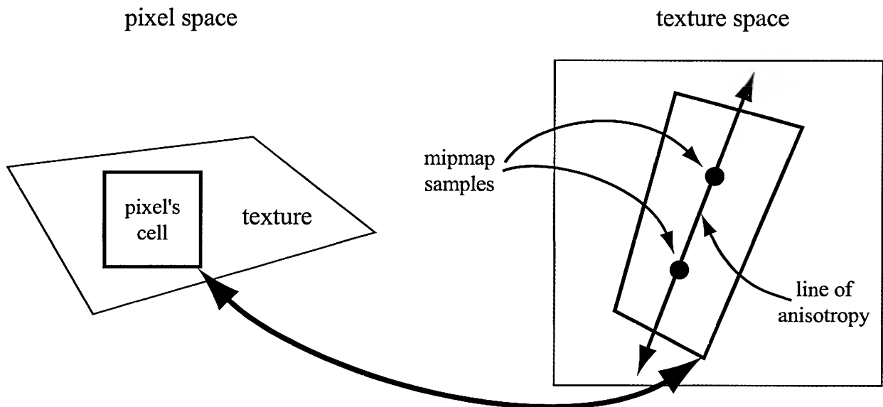
Figure 6.17. Anisotropic filtering. The back-projection of the pixel cell creates a quadrilateral. A line of anisotropy is formed between the longer sides.
