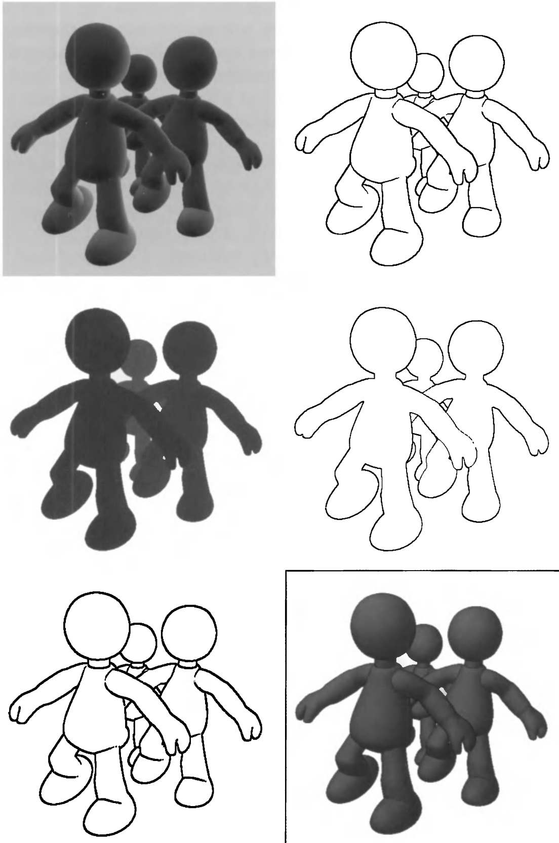
Figure 11.11. The normal map (upper left) and depth map (middle left) have edge detection applied to their values. The upper right shows edges found by processing the normal map, the upper middle from the z -depth map. The image on the lower left is a thickened composite. The final rendering in the lower right is made by shading the image with Gooch shading and compositing in the edges. ( Images courtesy of Drew Card and Jason L. Mitchell, ATI Technologies Inc. )
