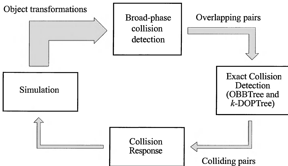
Figure 17.13. The outline of the collision detection system. The overlapping object pairs found by the first level broad phase CD algorithm are reported to the exact CD system, which, in turn, reports true collisions to a part of the system that should compute the collision response. Finally, all objects are treated by the simulation, where objects get their transforms, for example. (After Cohen et al. [181].)
