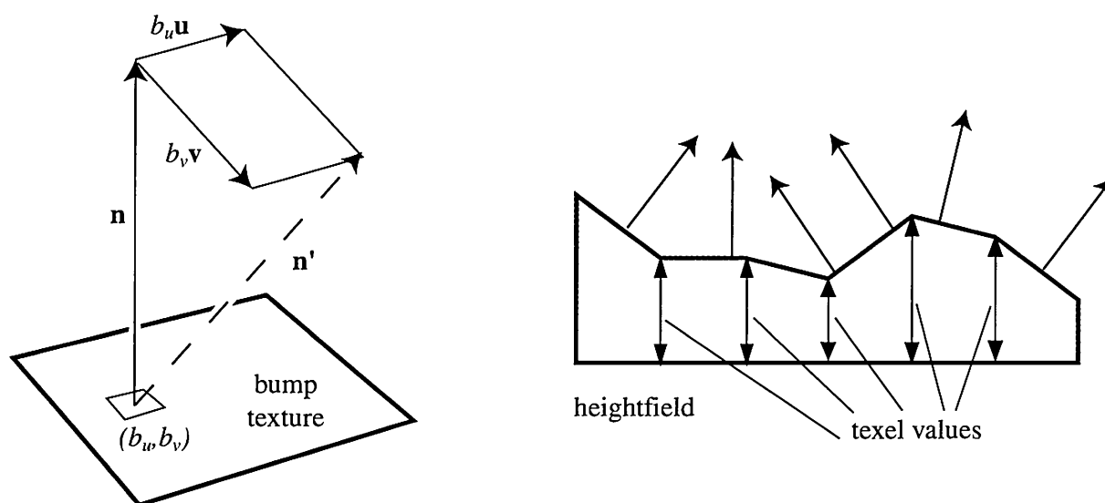
Figure 6.27. On the left, a normal vector \mathbf{n} is modified in the u and v directions by the (b_u, b_v) values taken from the bump texture, giving \mathbf{n}' (which is unnormalized). On the right, a heightfield and its effect on shading normals is shown. These normals could instead be interpolated between heights for a smoother look.
