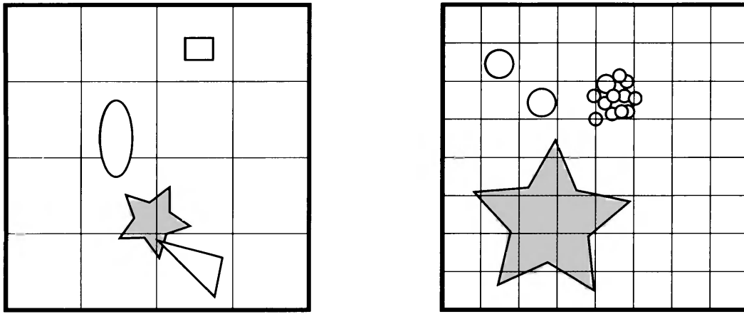
Figure 17.12. Left: a low-resolution two-dimensional grid with four objects. Note that since the ellipse and the star overlap a shared grid cell, these objects have to be tested using a BV/BV test. In this case, they do not collide. The triangle and the star also overlap a shared grid cell, and they do in fact collide. Right: a higher-resolution grid. As can be seen, the star overlaps with many grid cells, which can make this procedure expensive. Also note that there are many smaller objects where clumping occurs, and this is another possible source of inefficiency.
