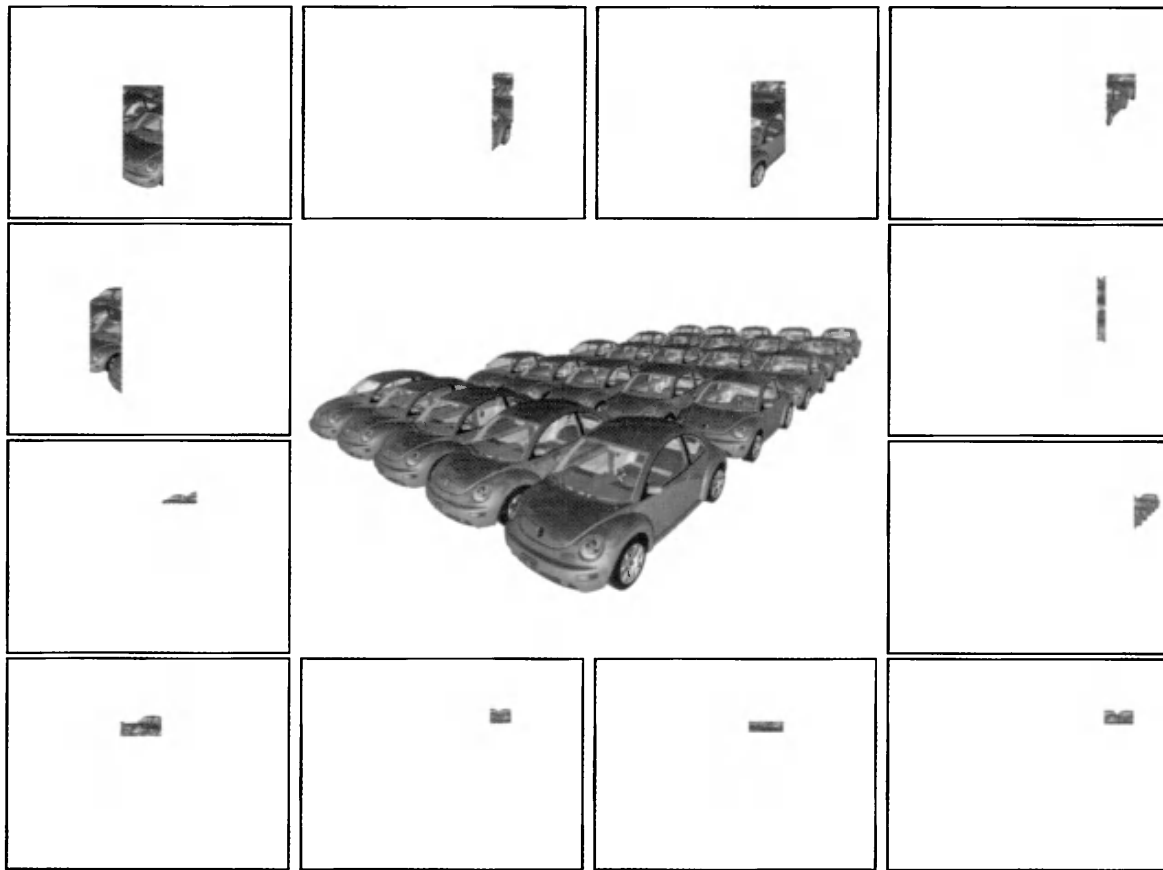
Figure 18.10. Sort-first splits the screen into separate tiles and assigns a processor to each tile, as shown here. A primitive is then sent to the processors whose tiles they overlap. This is in contrast to sort-middle architecture, which needs to sort all triangles after geometry processing has occurred. Only after all triangles have been sorted can per-pixel rasterization start. ( Images courtesy of Marcus Roth and Dirk Reinert. )
