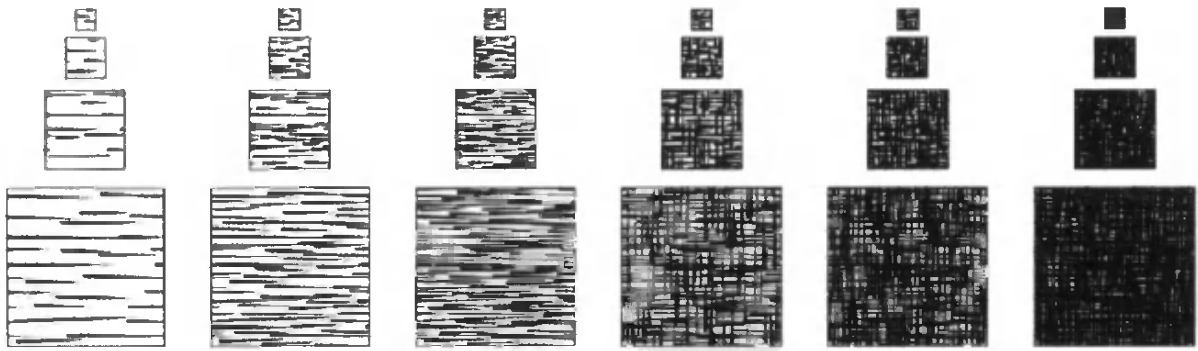
Figure 11.14. Tonal art maps (TAMs). Strokes are drawn into the mipmap levels. Each mipmap level contains all the strokes from the textures to the left and above it. In this way, interpolation between mip levels and adjoining textures is smooth. (Images courtesy of Emil Praun, Princeton University.)
